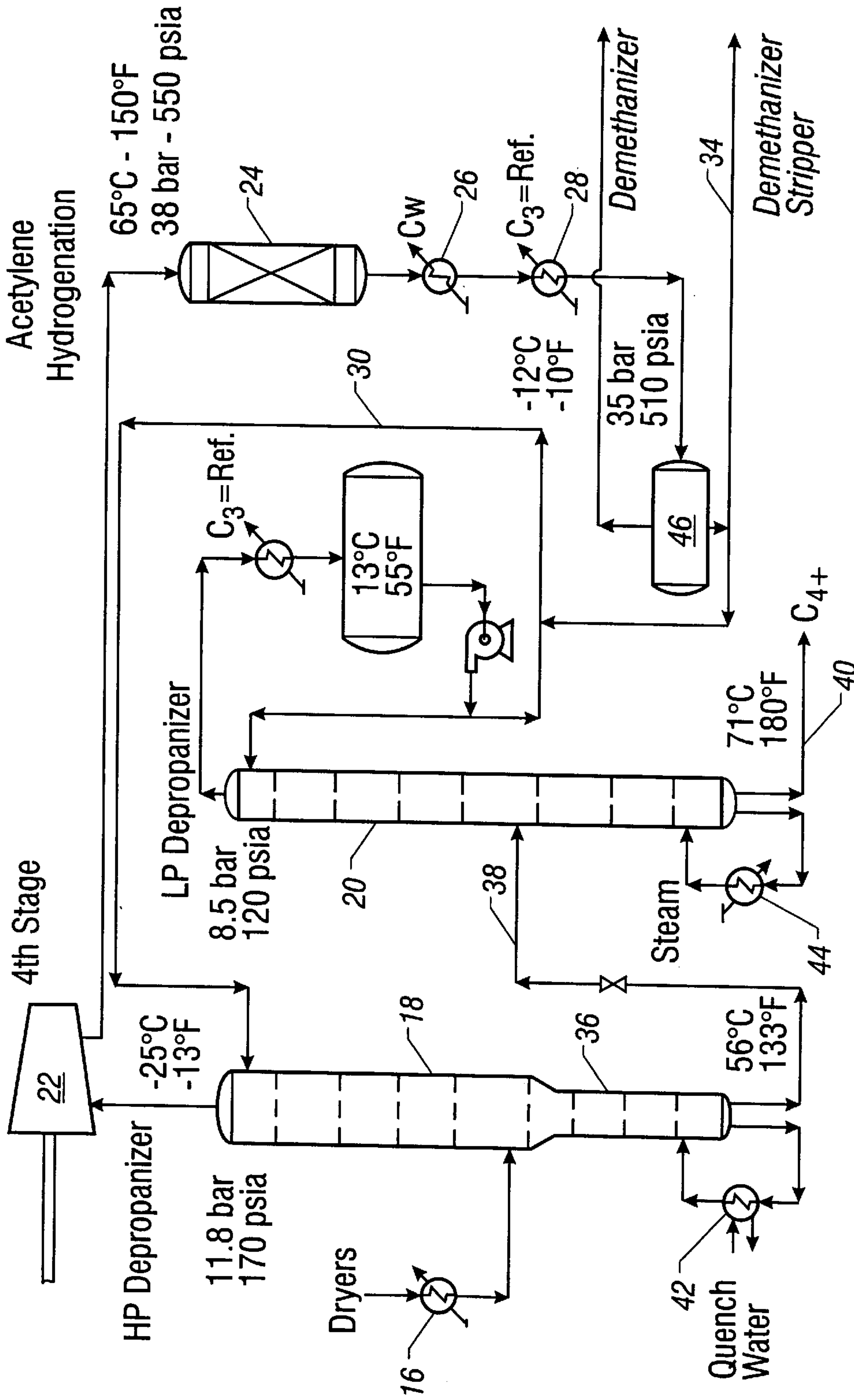
FIG. 3 (PRIOR ART)
