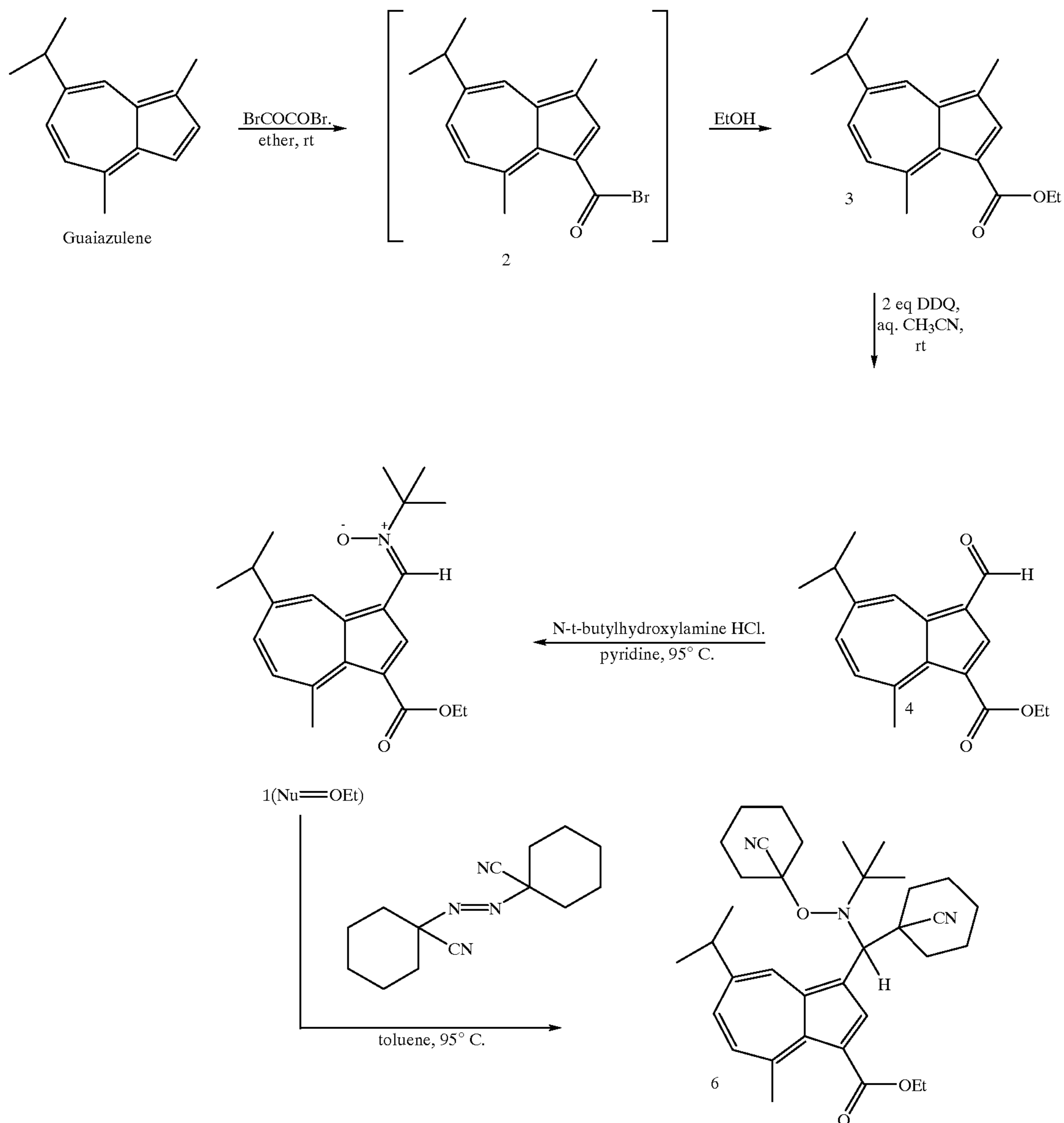
SCHEME 1
