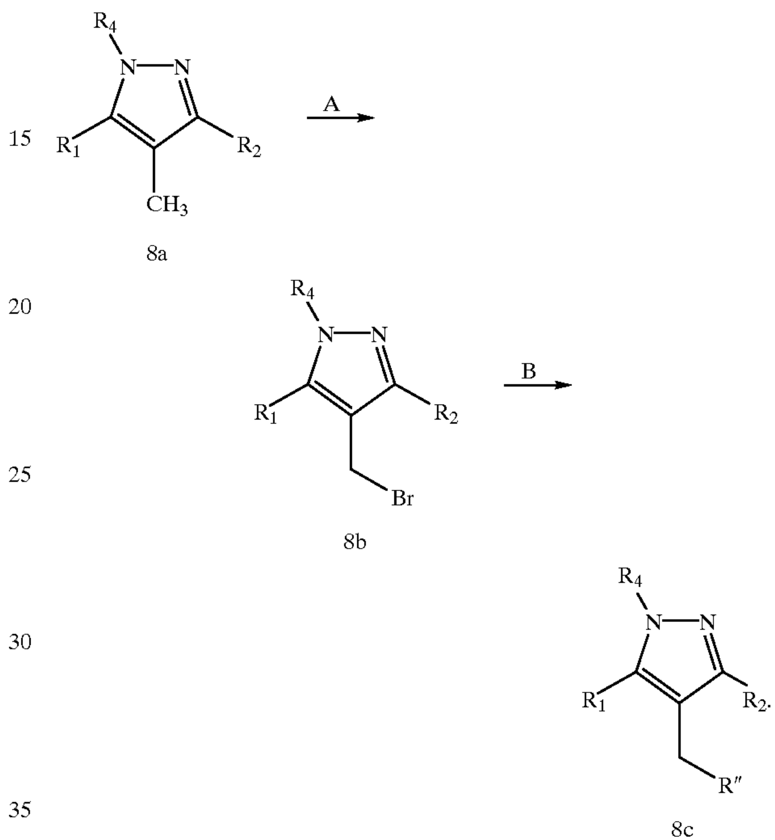
Scheme 8
