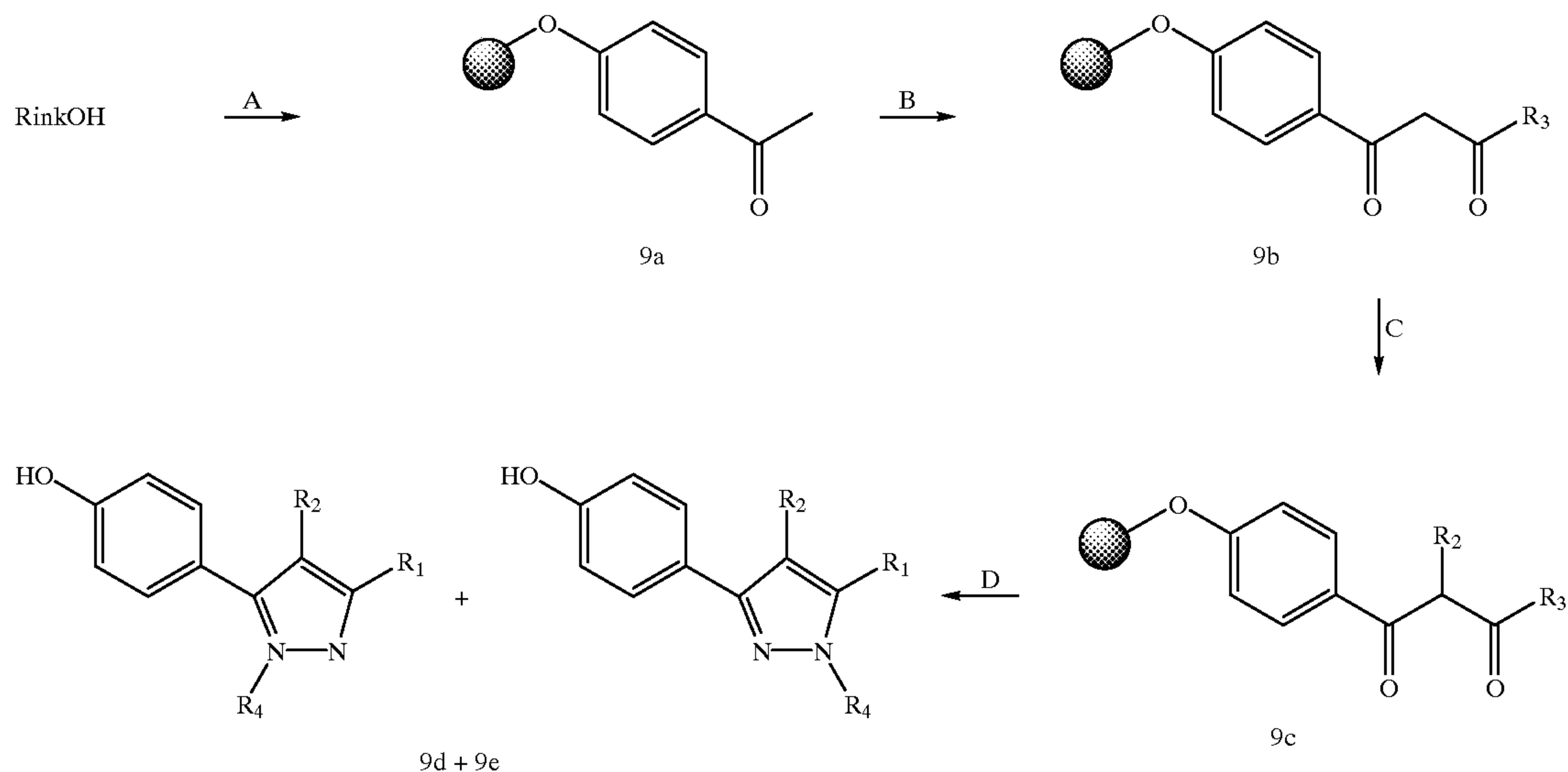
Scheme 9
