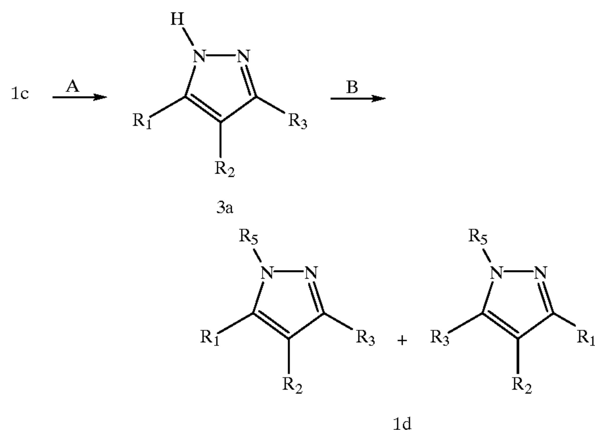
Scheme 3
