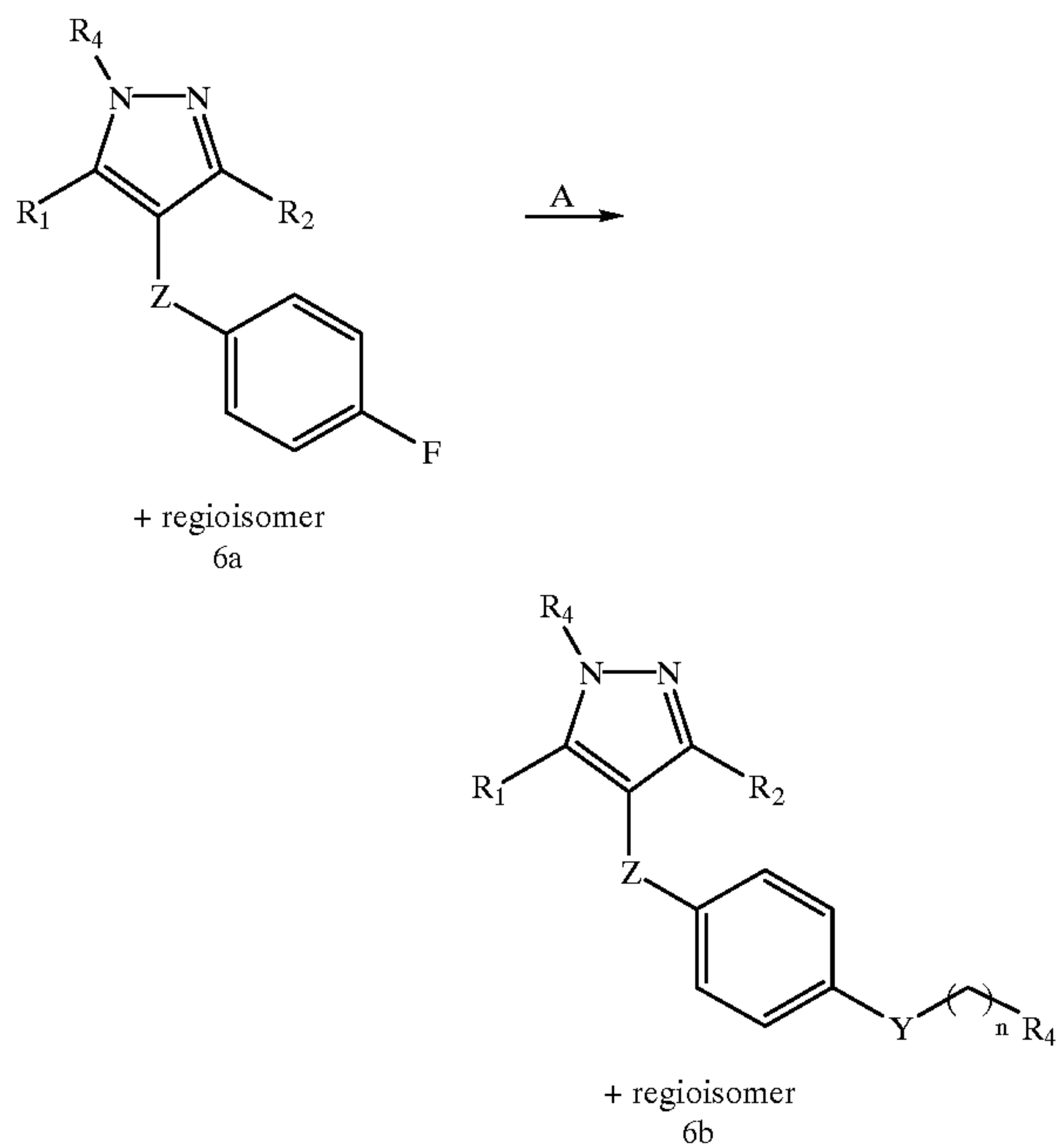
Scheme 6
