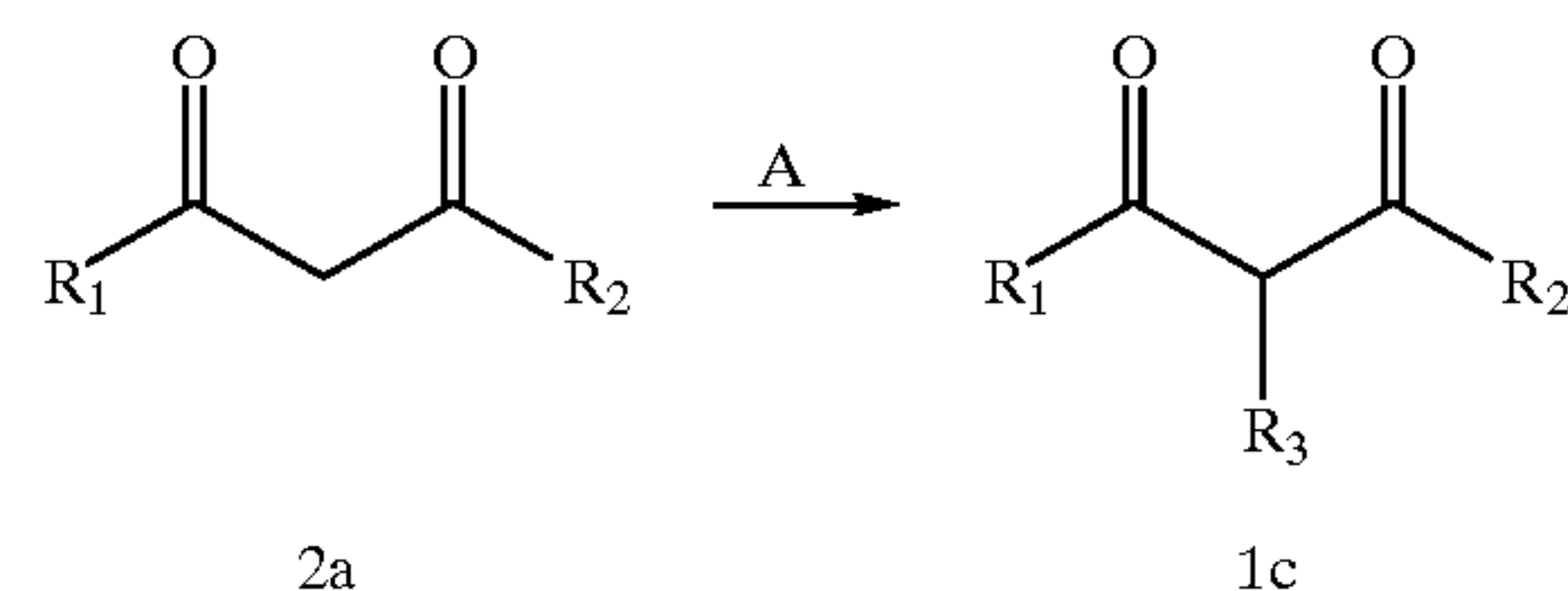
Scheme 2
