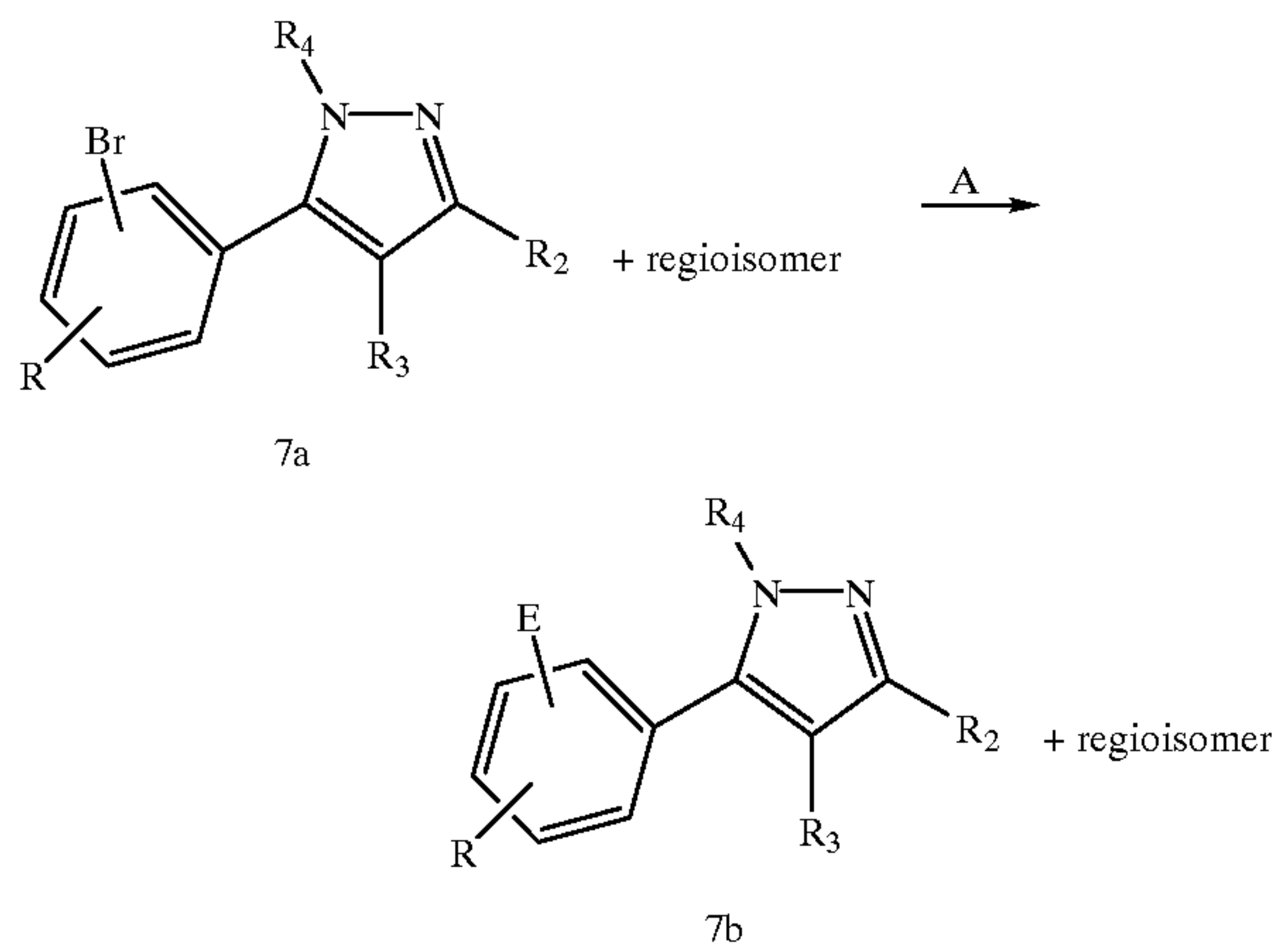
Scheme 7
