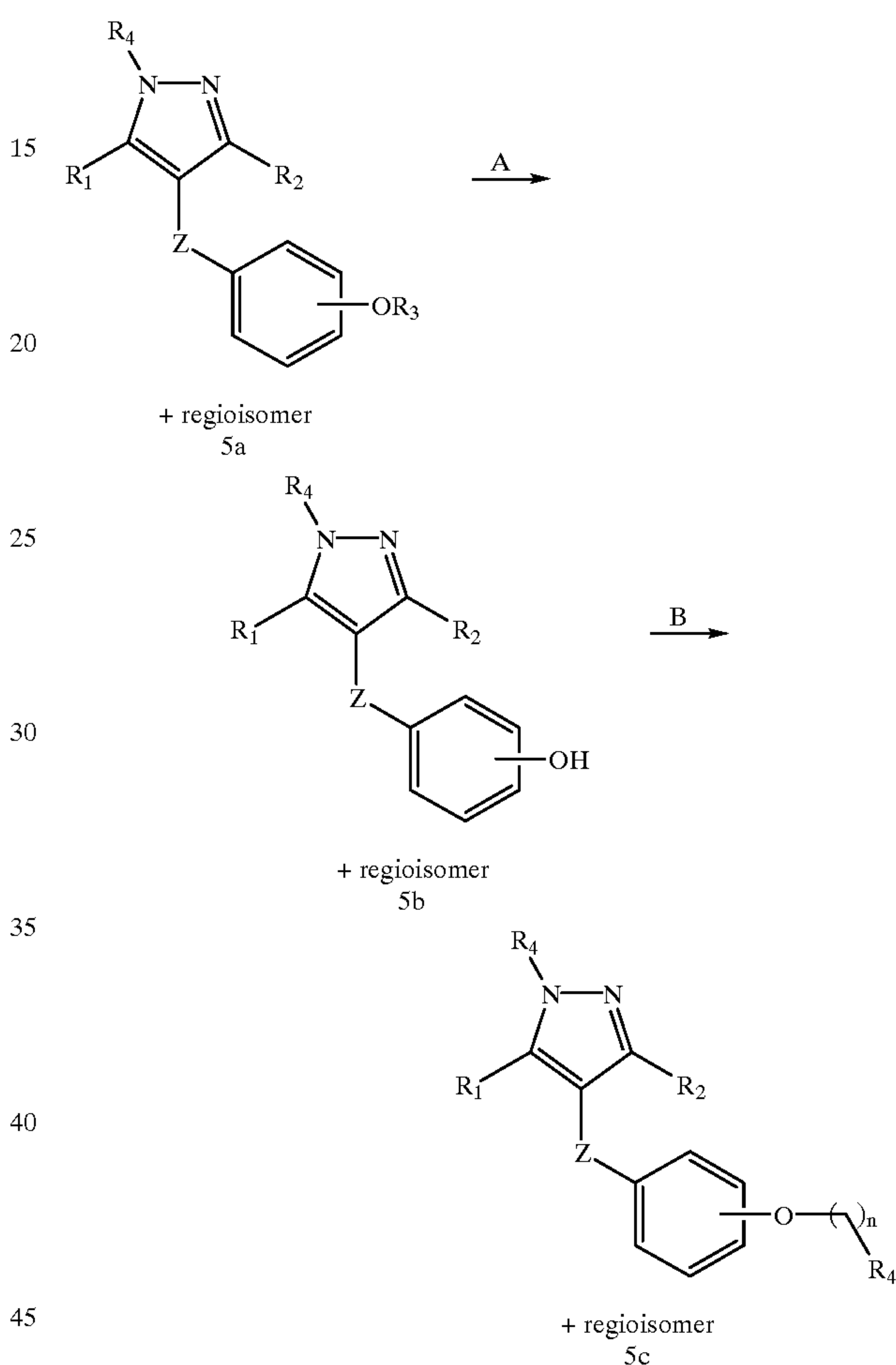
Scheme 5
