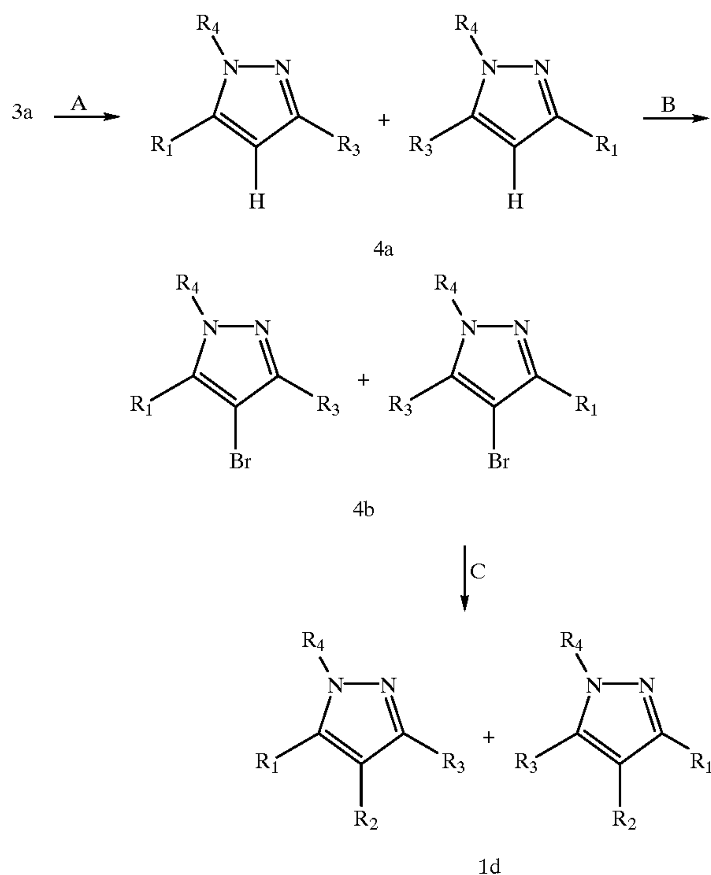
Scheme 4
