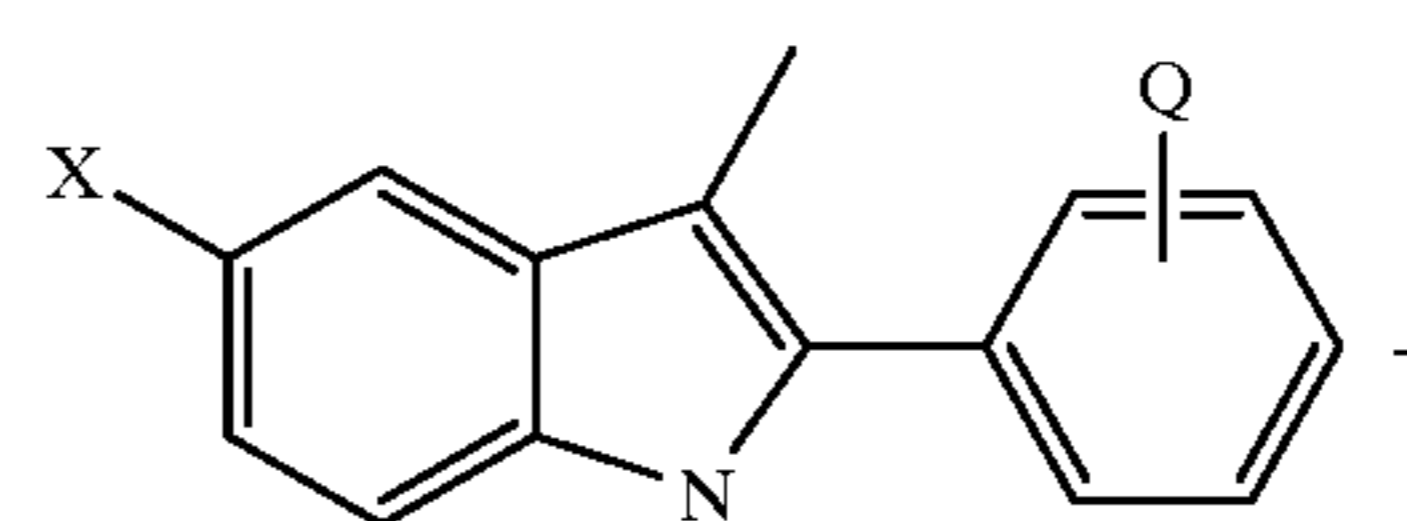
Scheme 9
