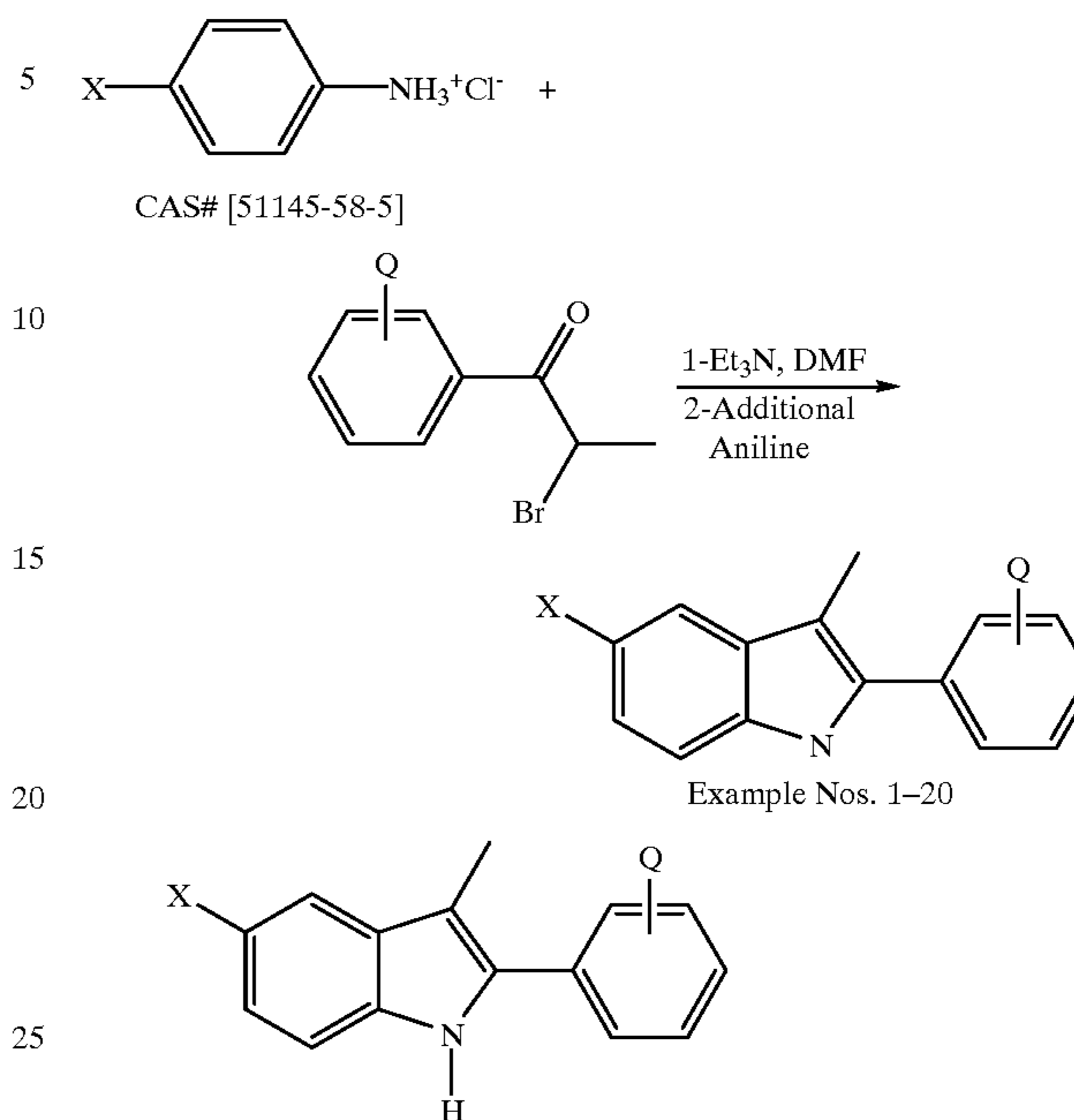
Scheme 8
