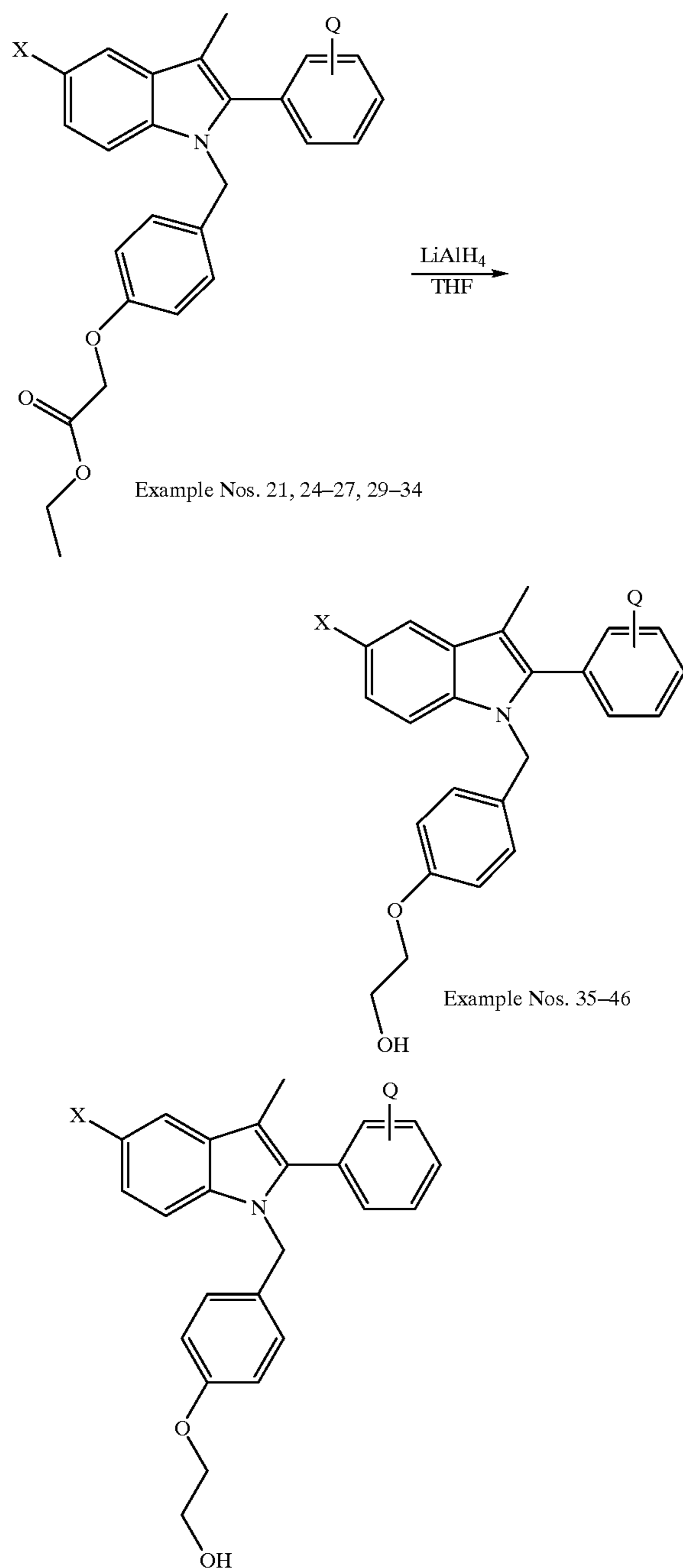
Scheme 10
