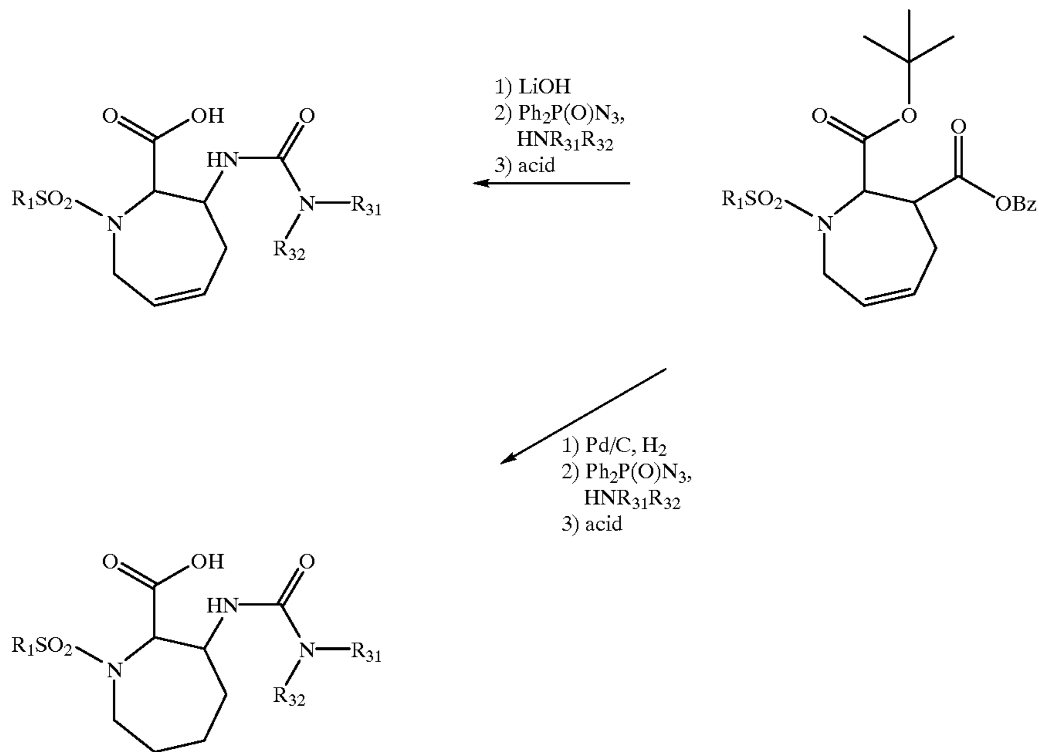
SCHEME III
