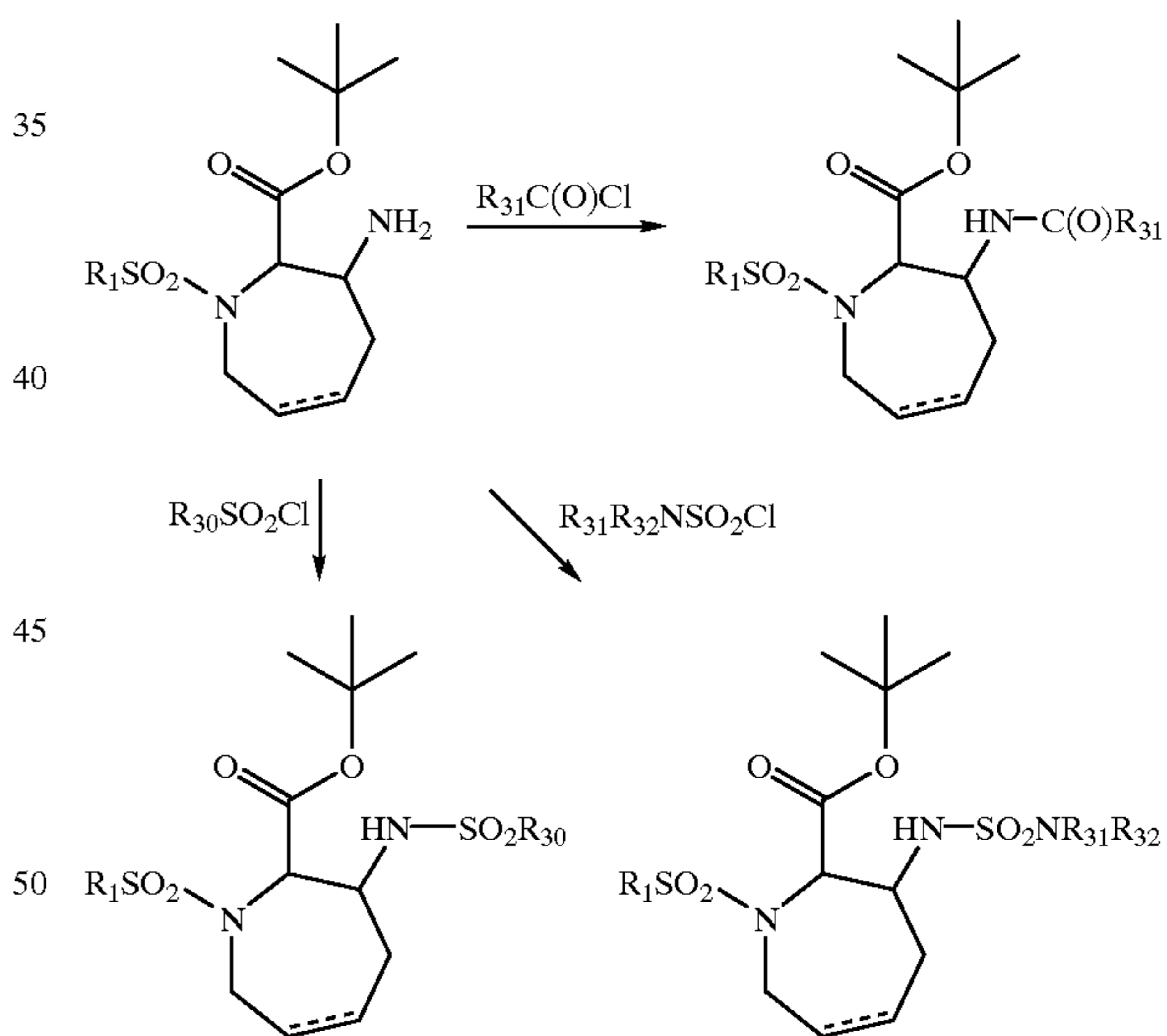
SCHEME V
