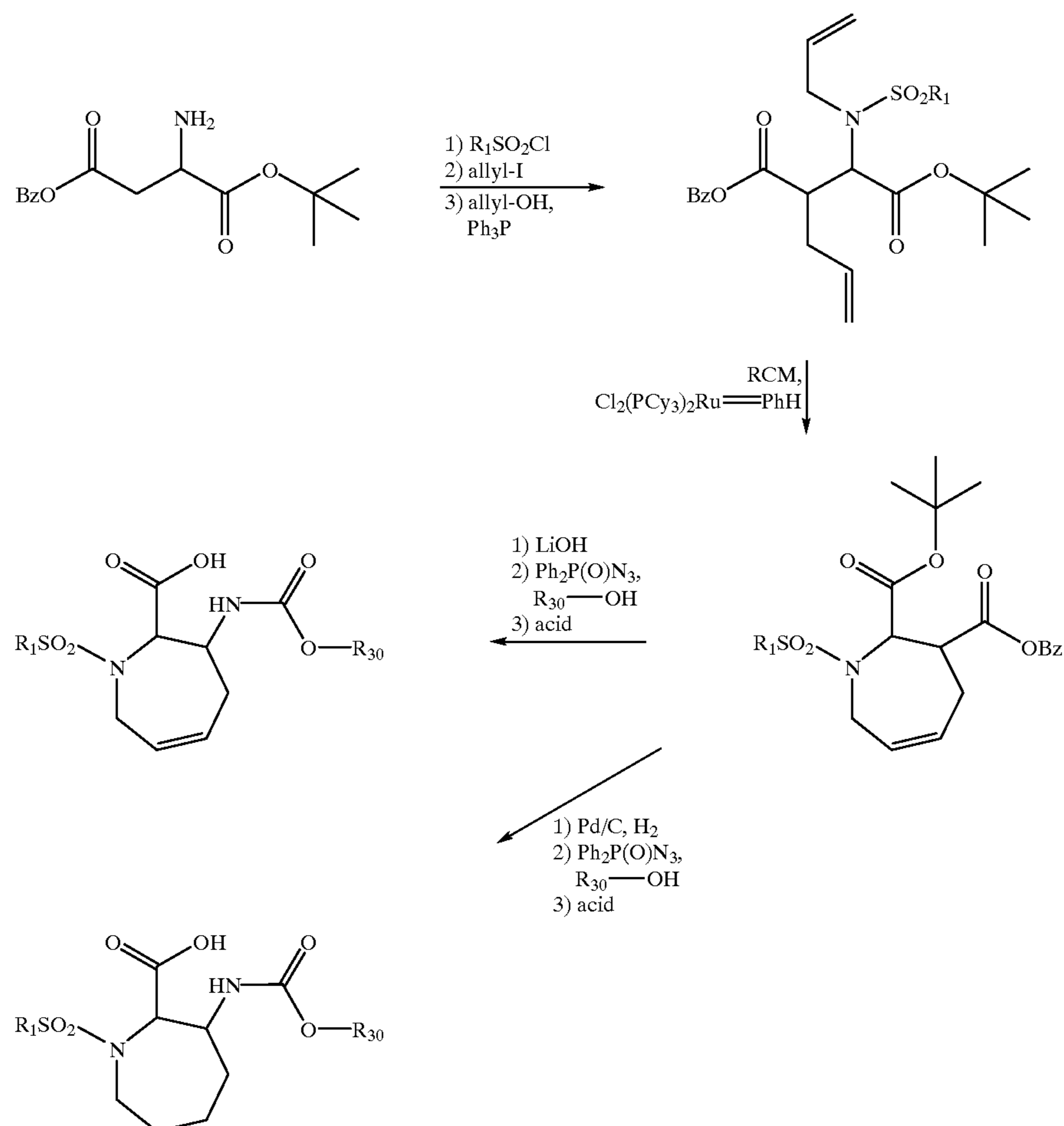
SCHEME II
