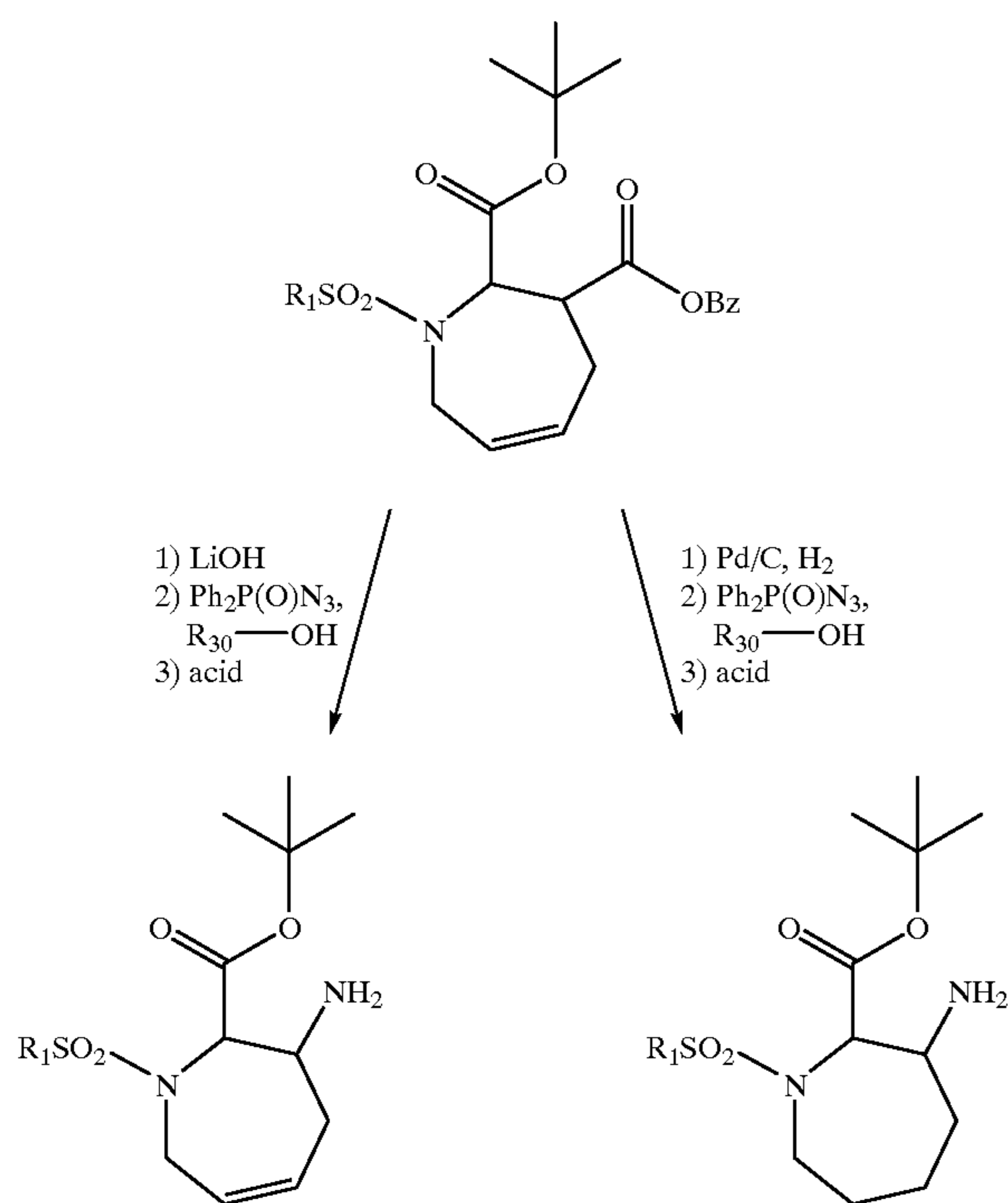
SCHEME IV
