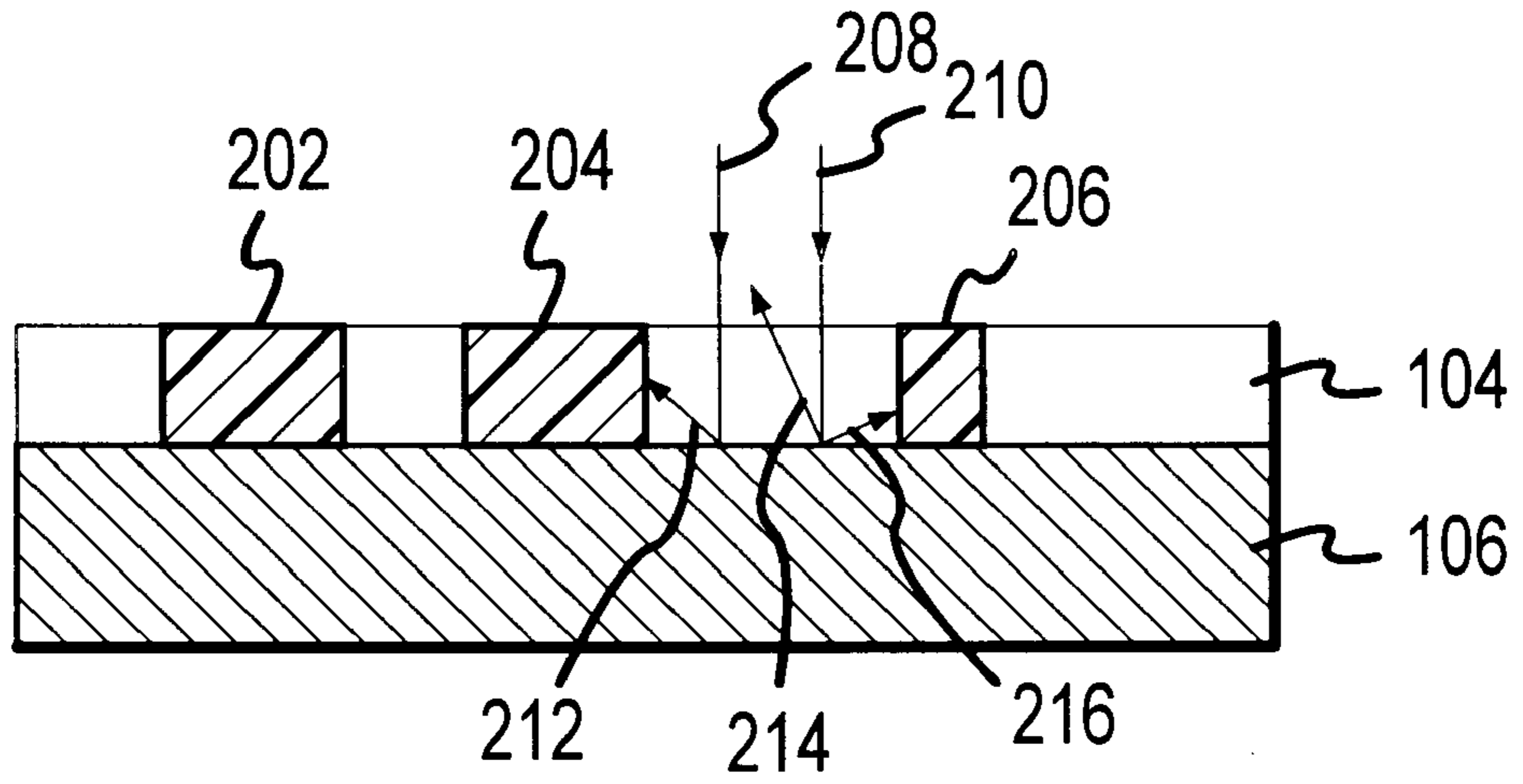
PRIOR ART FIG.2a
