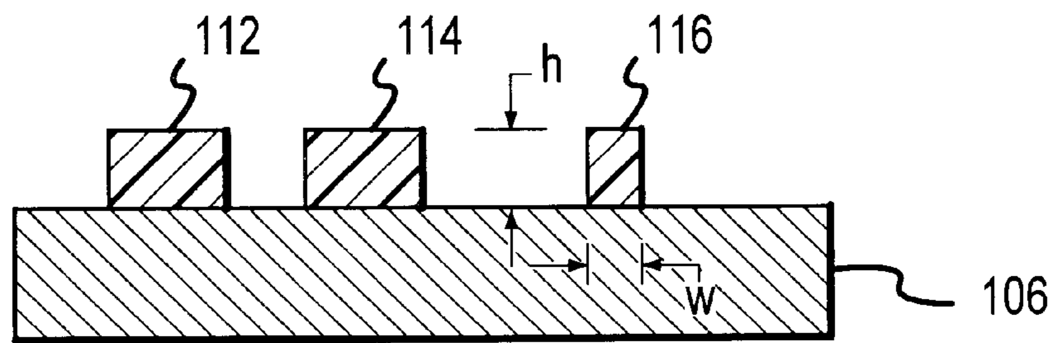
PRIOR ART FIG. 1b
