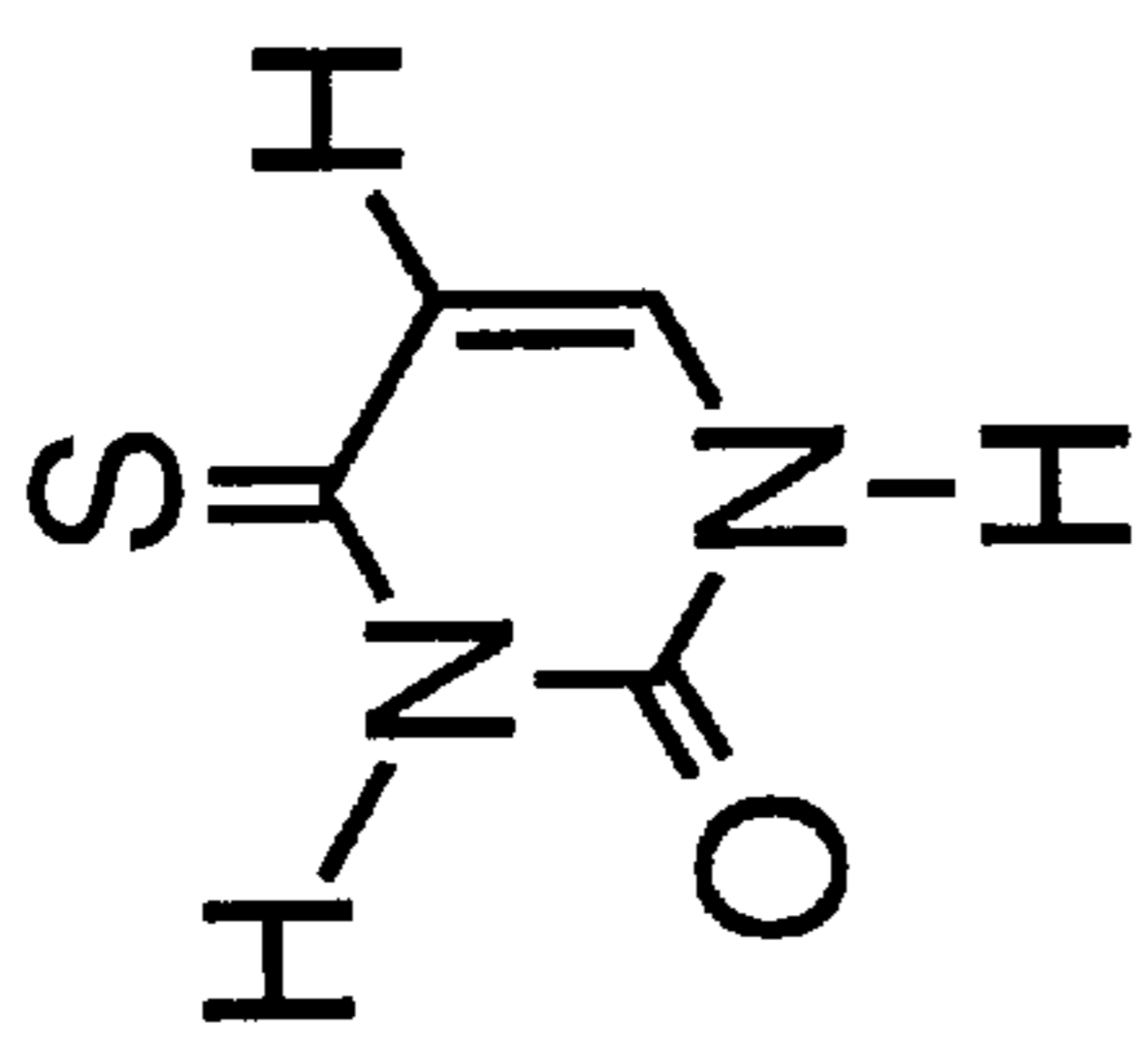
4-thiouracil
