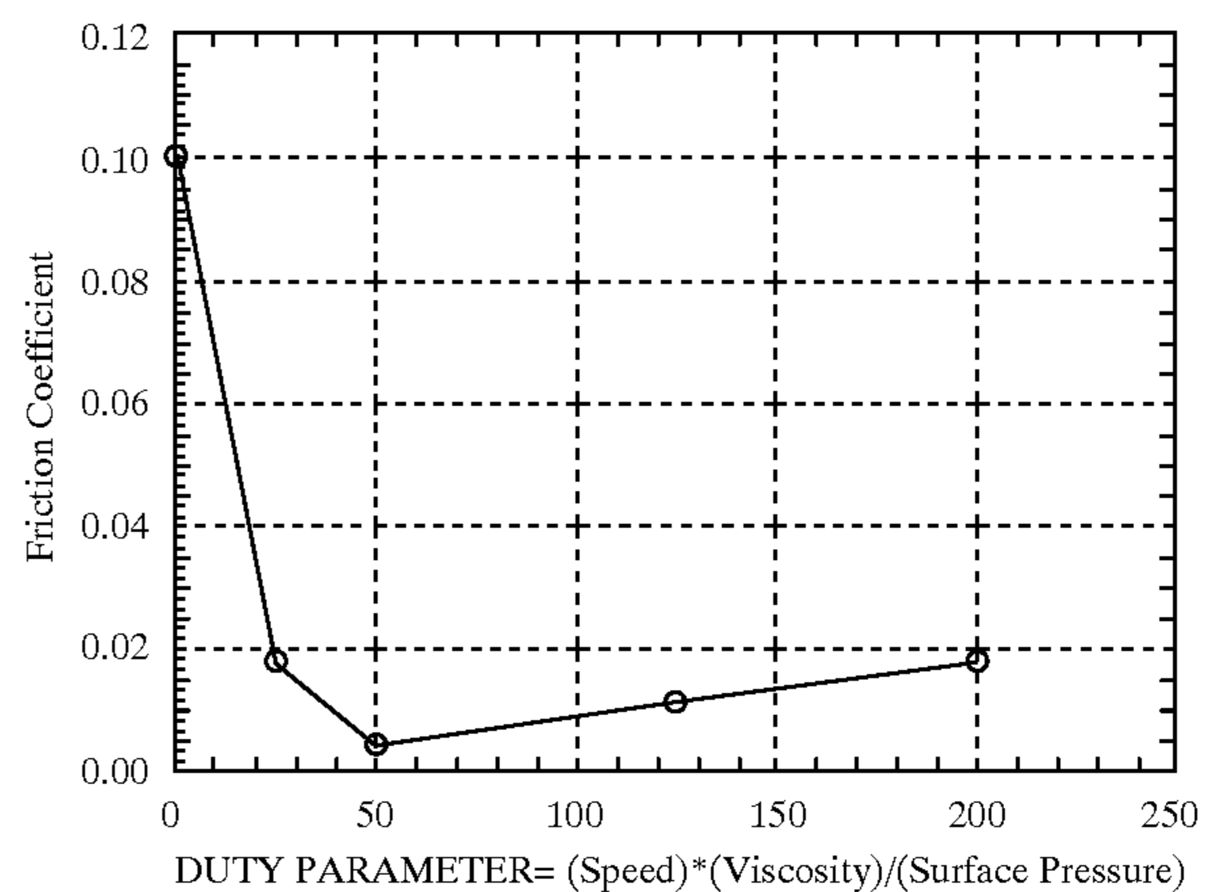
Graph 1. Stribeck diagram
