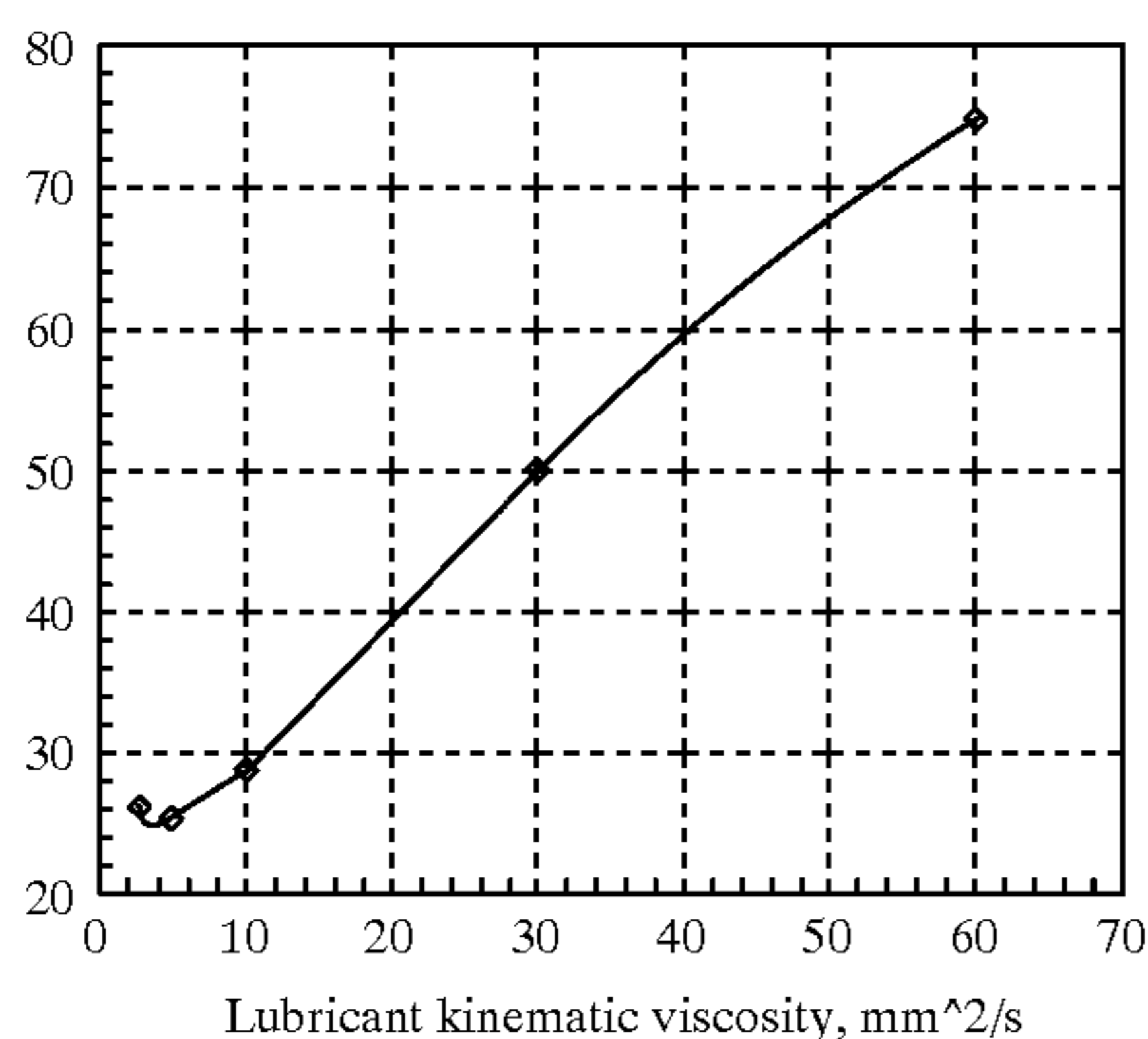
Graph 4. Total friction
