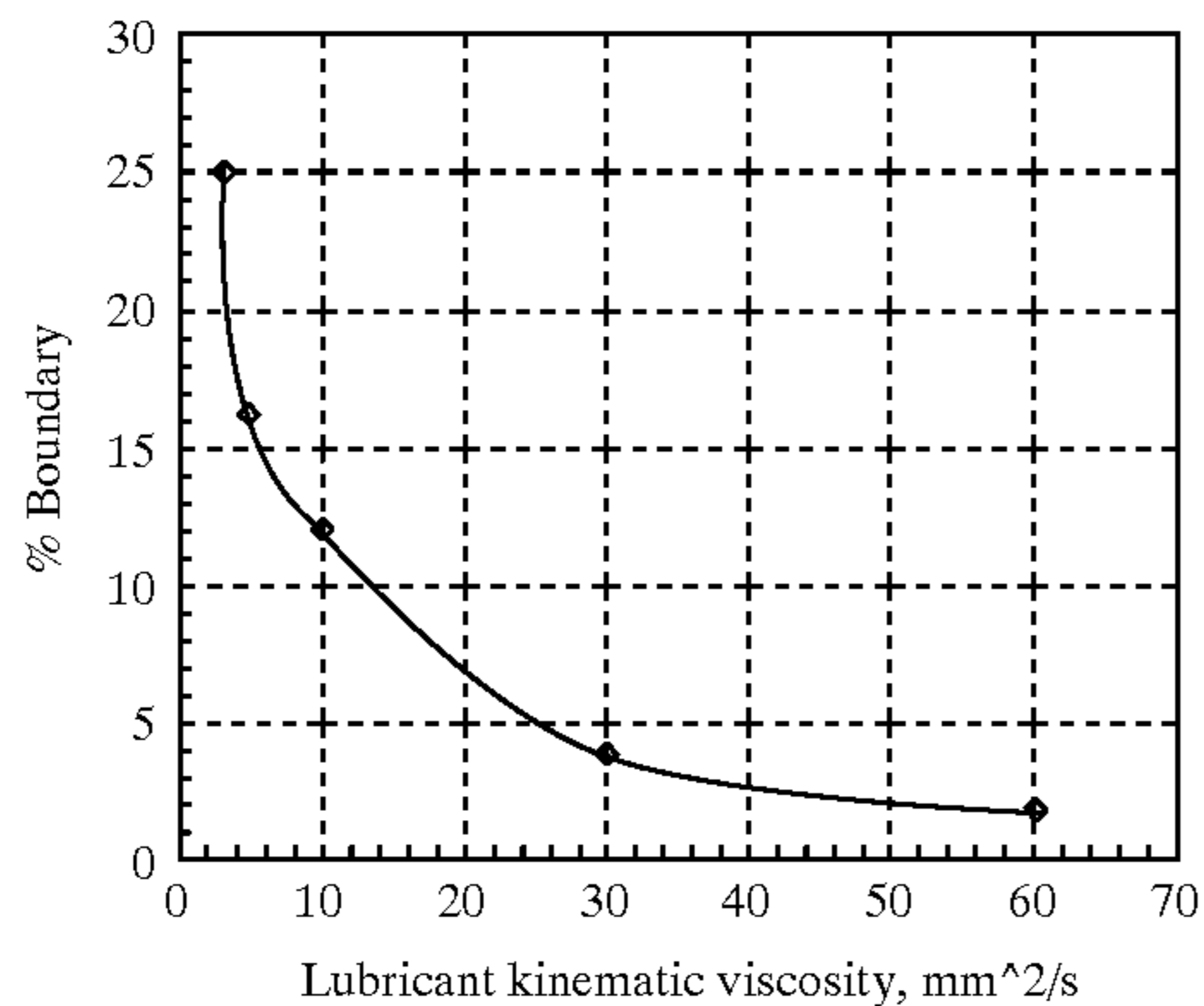
Graph 3. Boundary contribution
