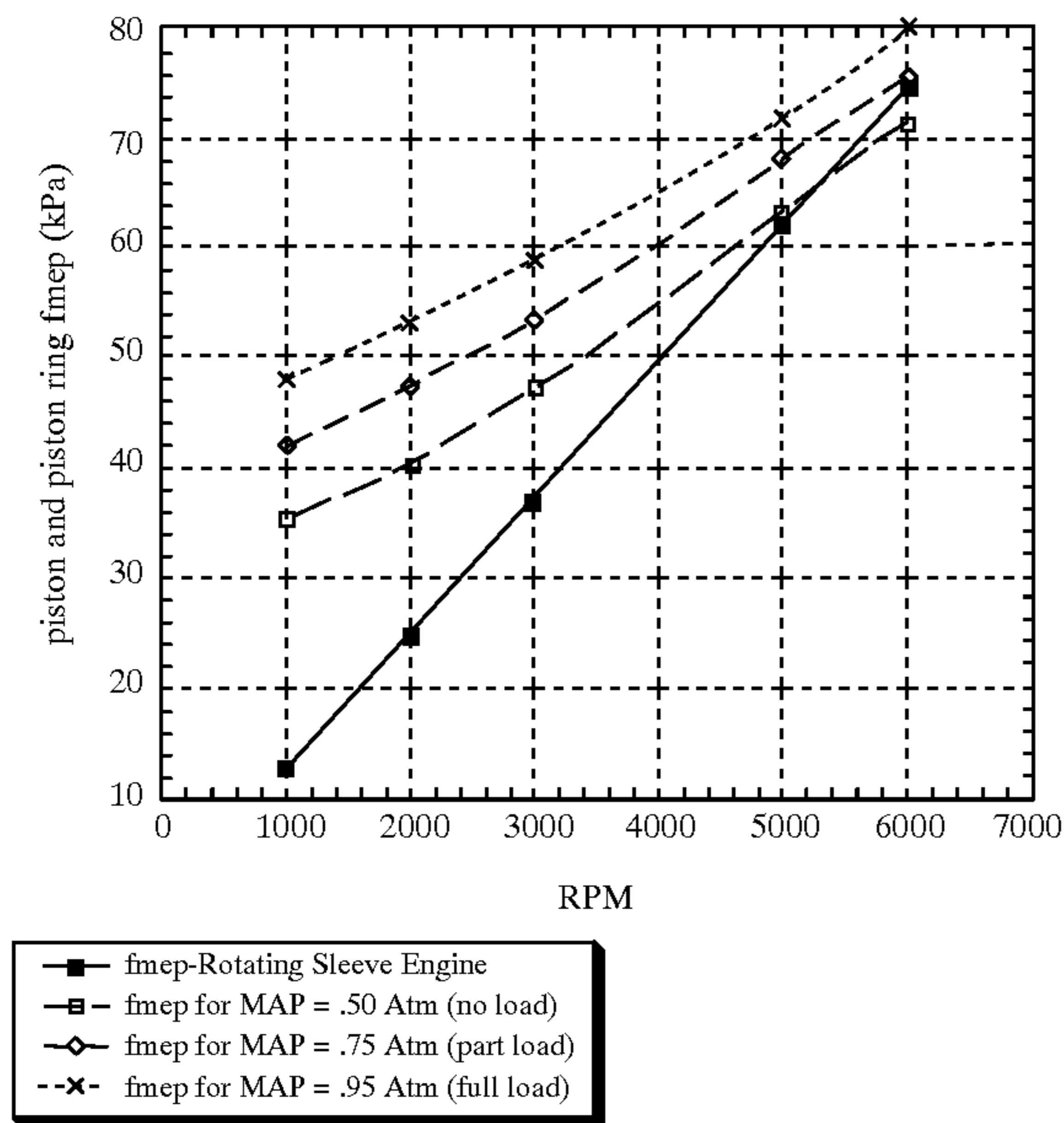
Comparison of fmep for a rotating sleeve engine with reduced sleeve speed with a conventional engine.
