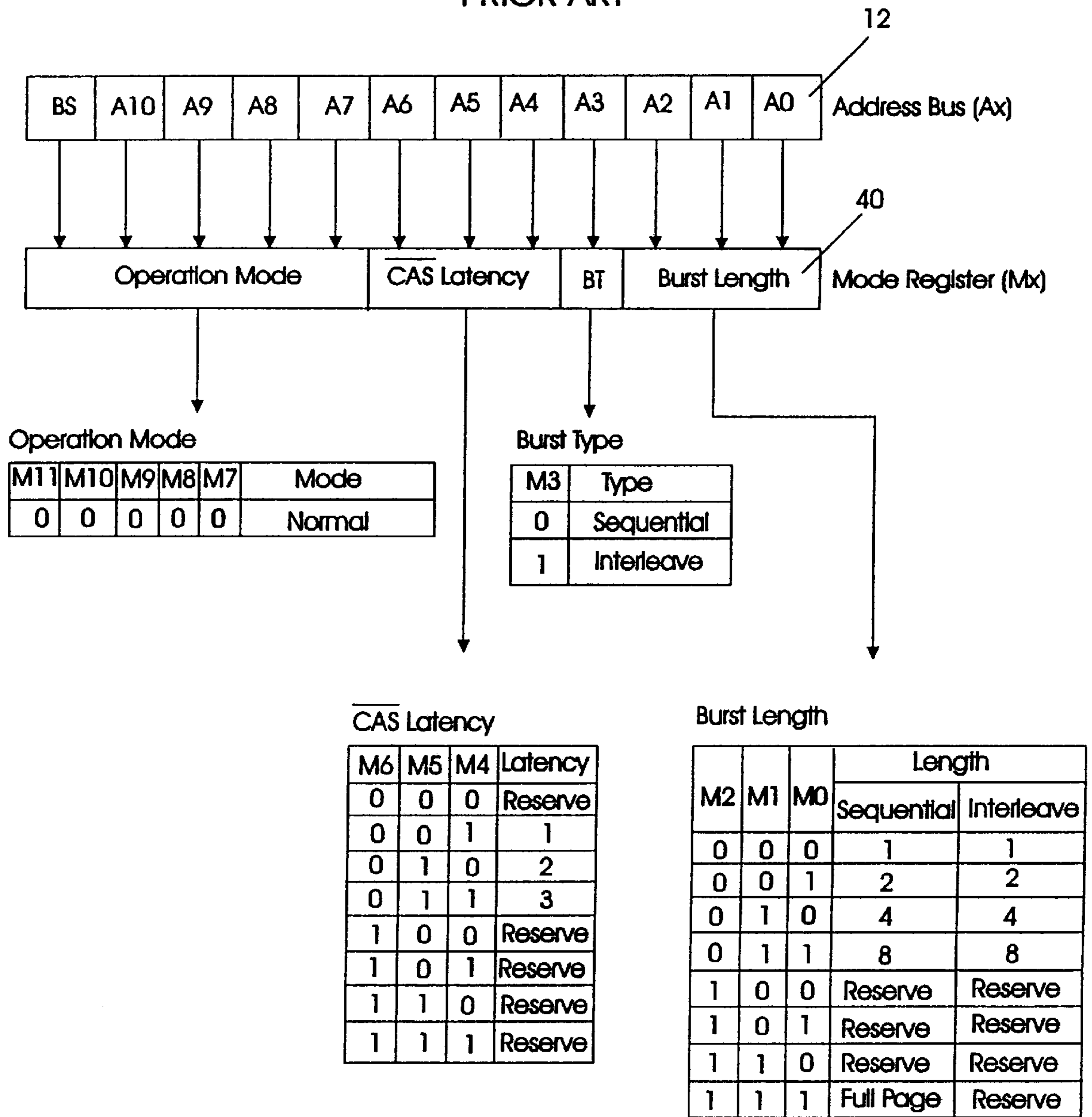
FIG. 2 PRIOR ART
