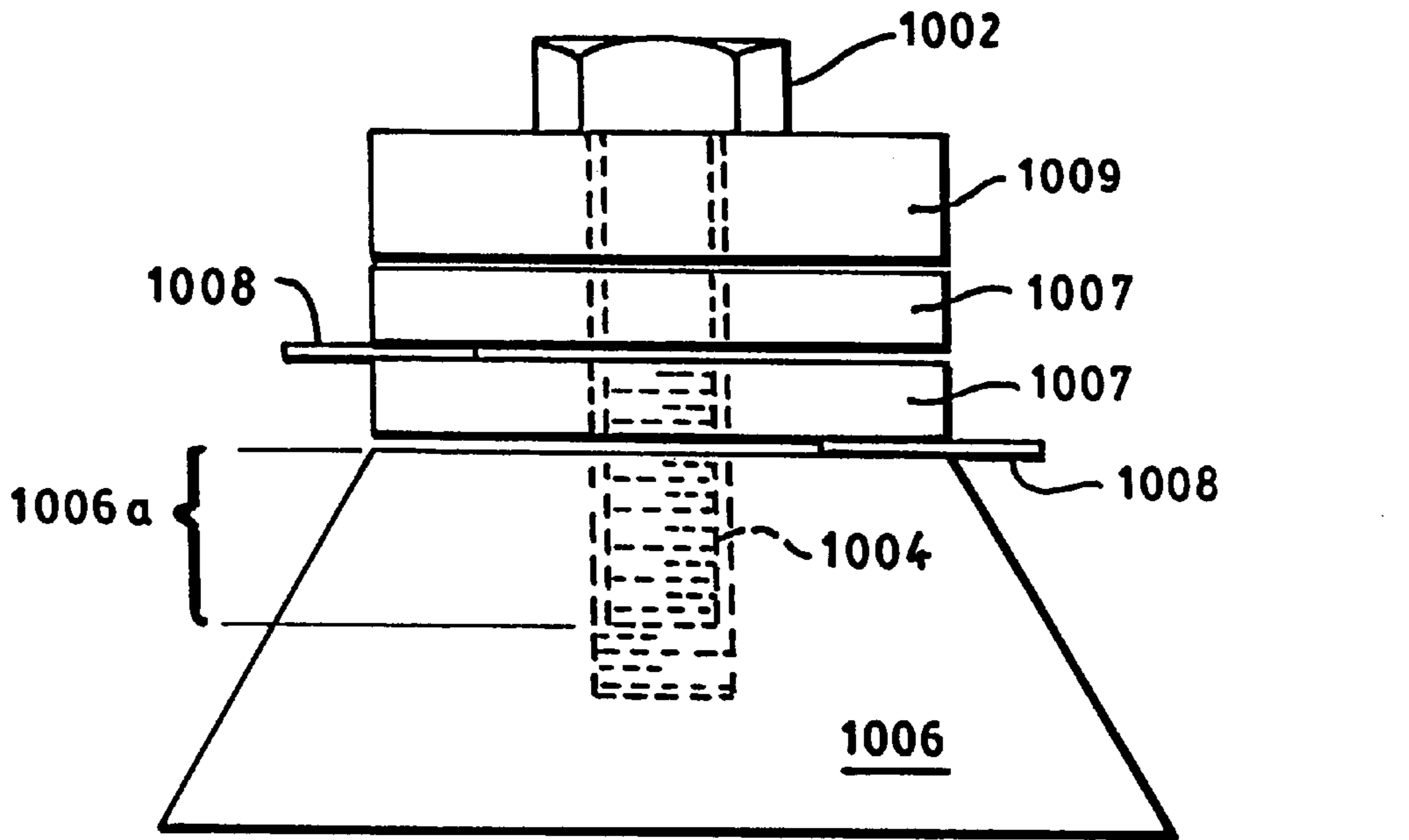
FIG. 51 (PRIOR ART)
