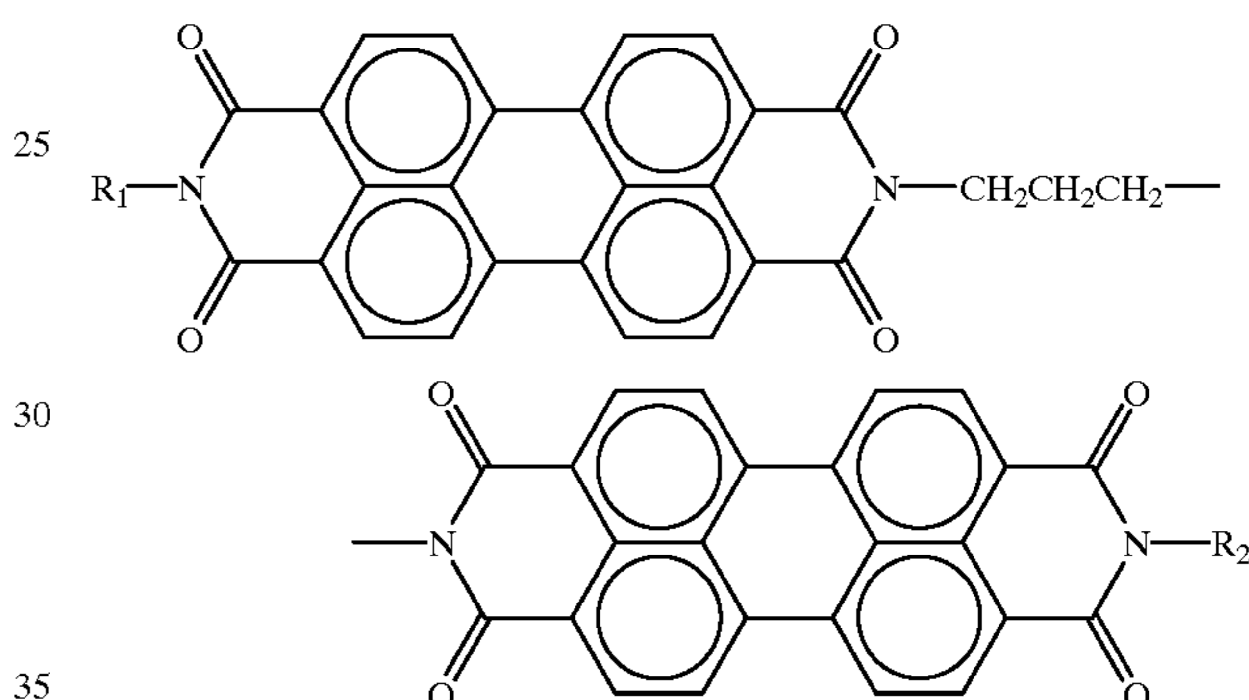
Formula 2
