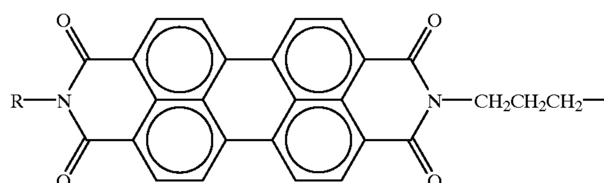
Formula 1
