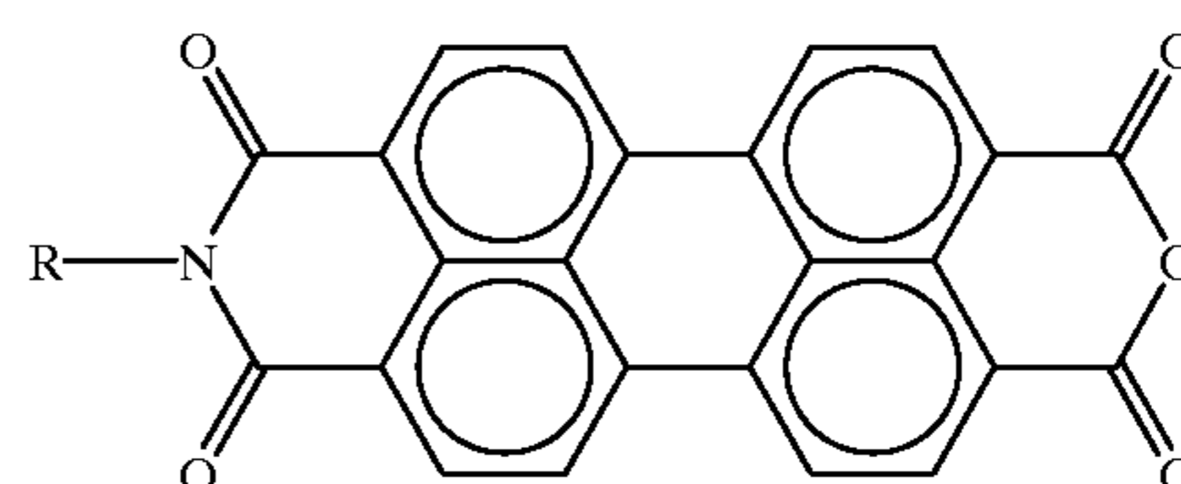
Formula 3
