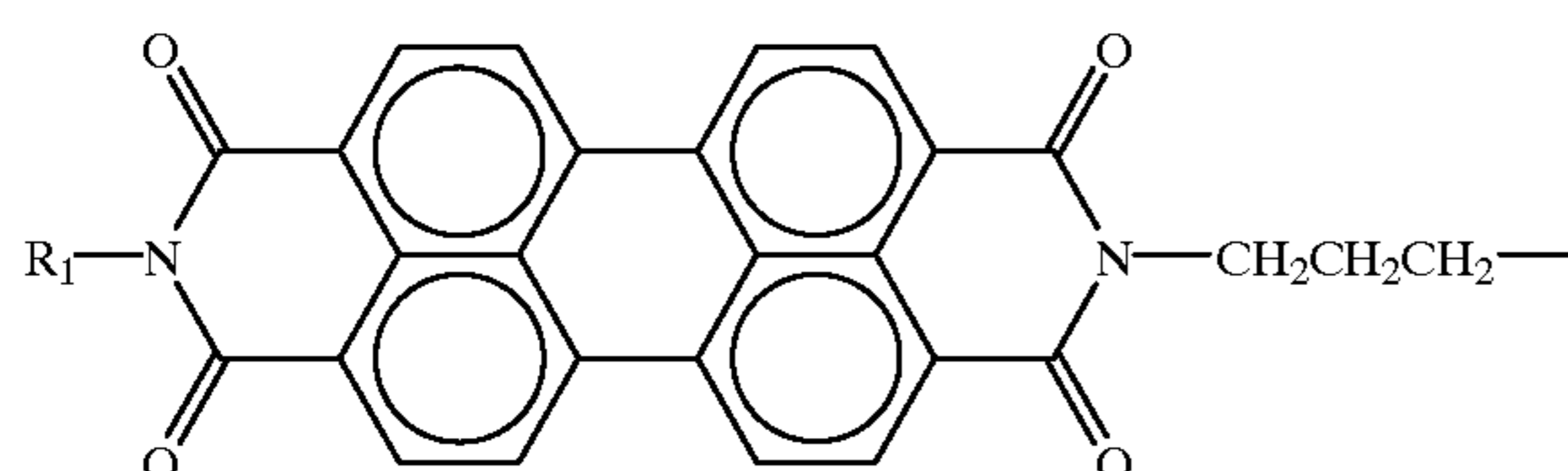
Formula 2
