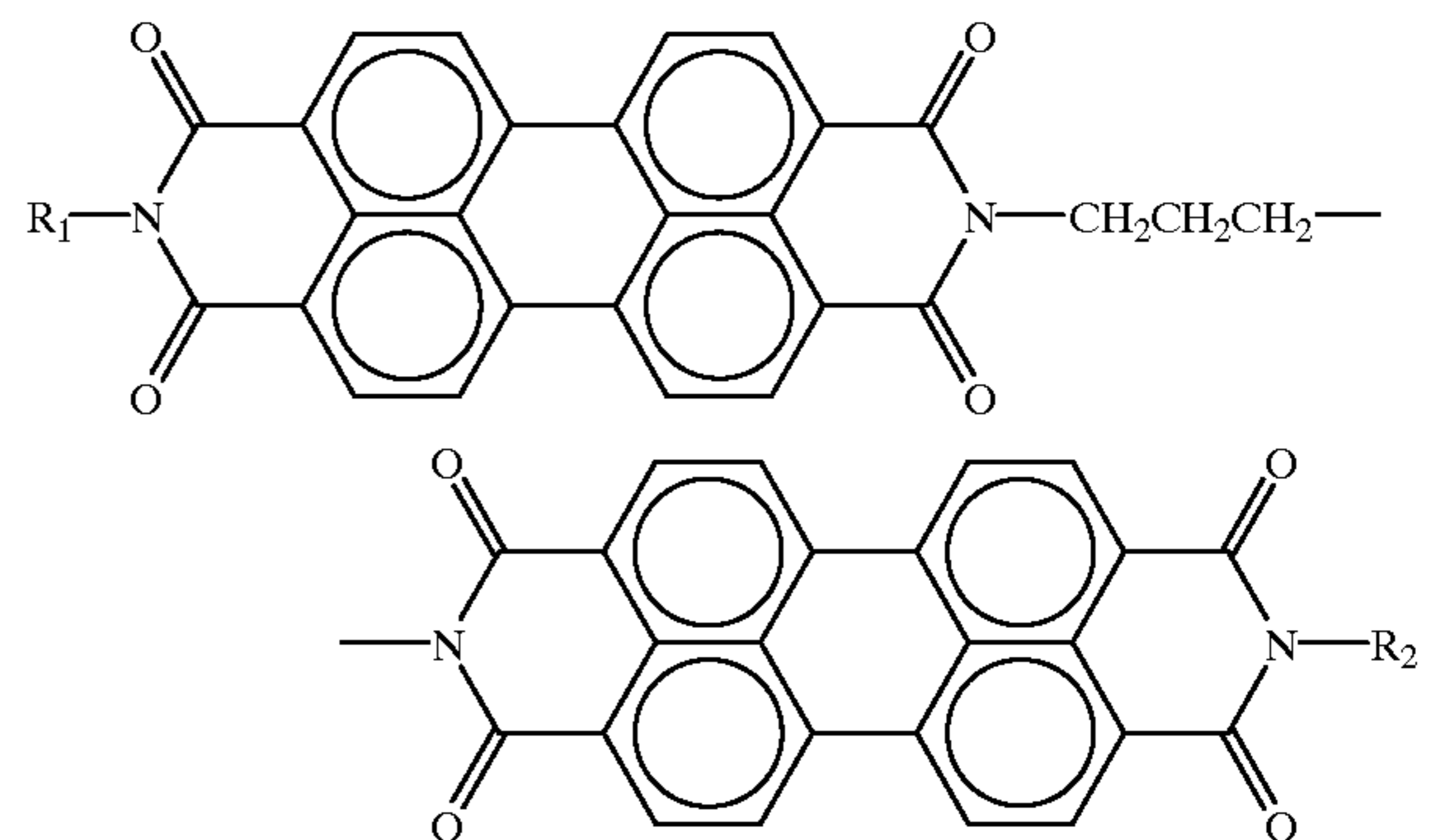
Formula 2
