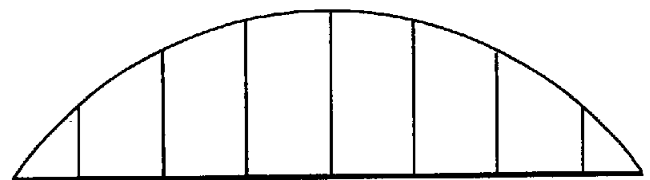
MOMENT DIAGRAM ALONG THE STENT
