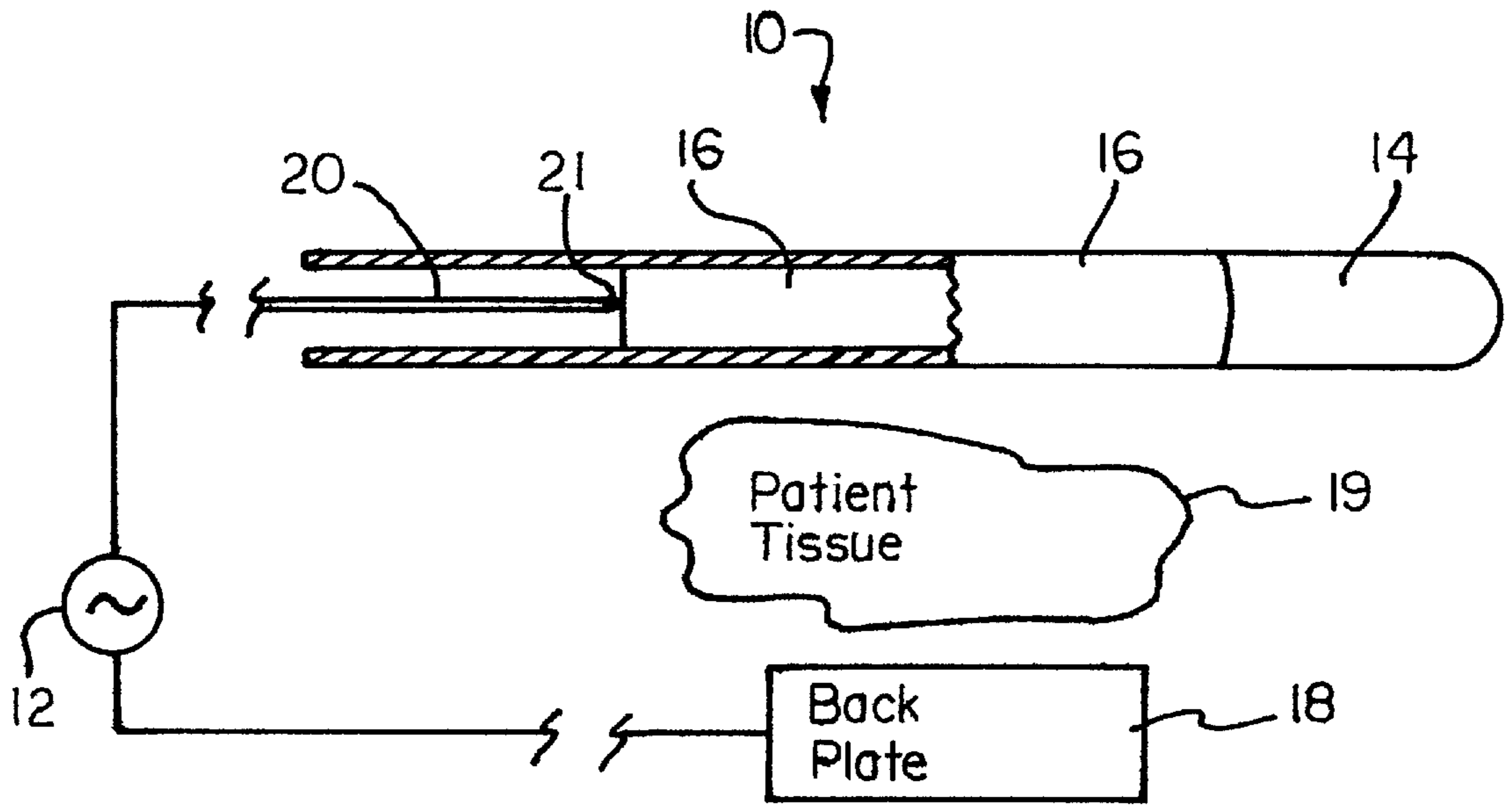
FIG. 1 (Prior Art)
