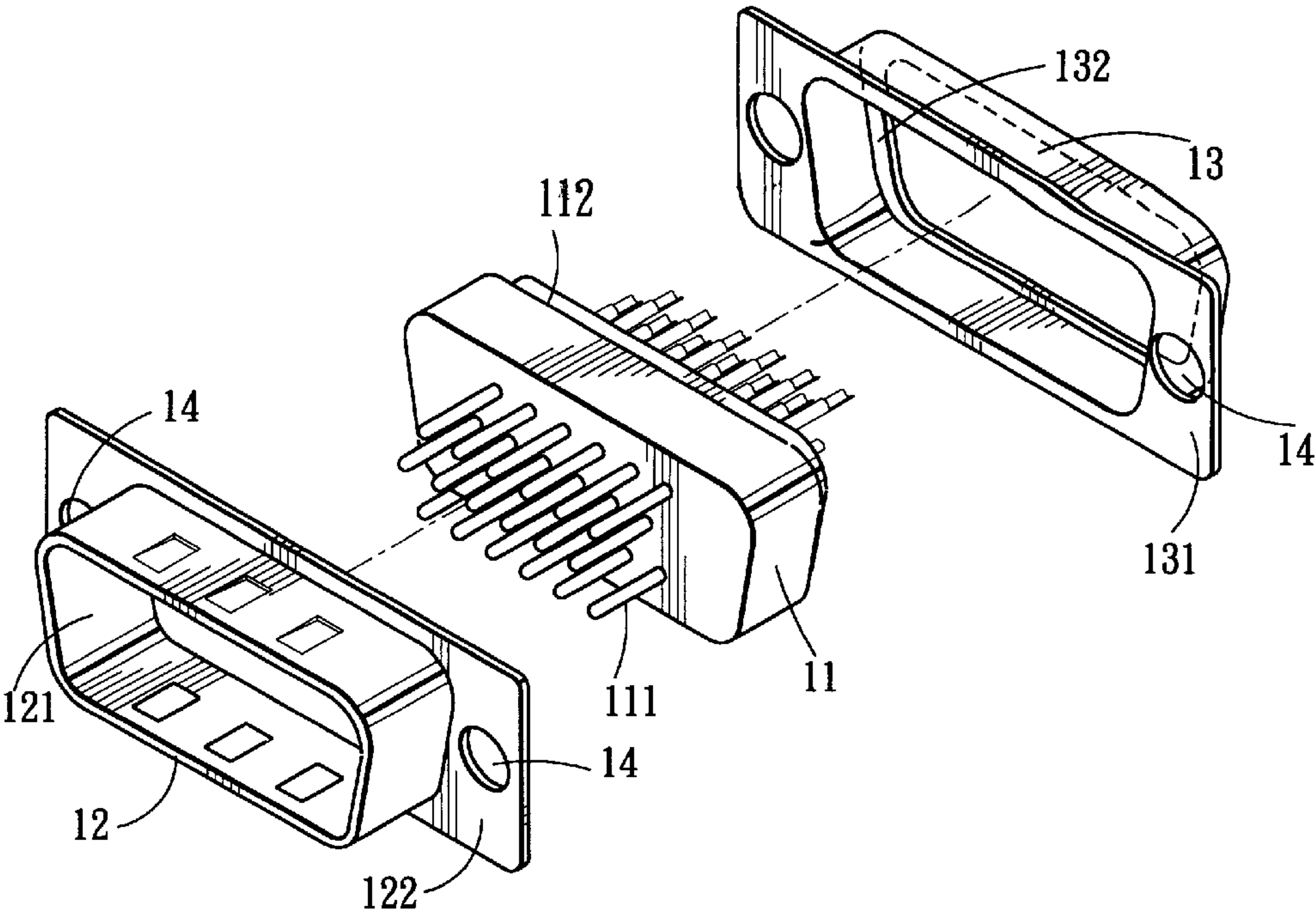
FIG. 1 PRIOR ART
