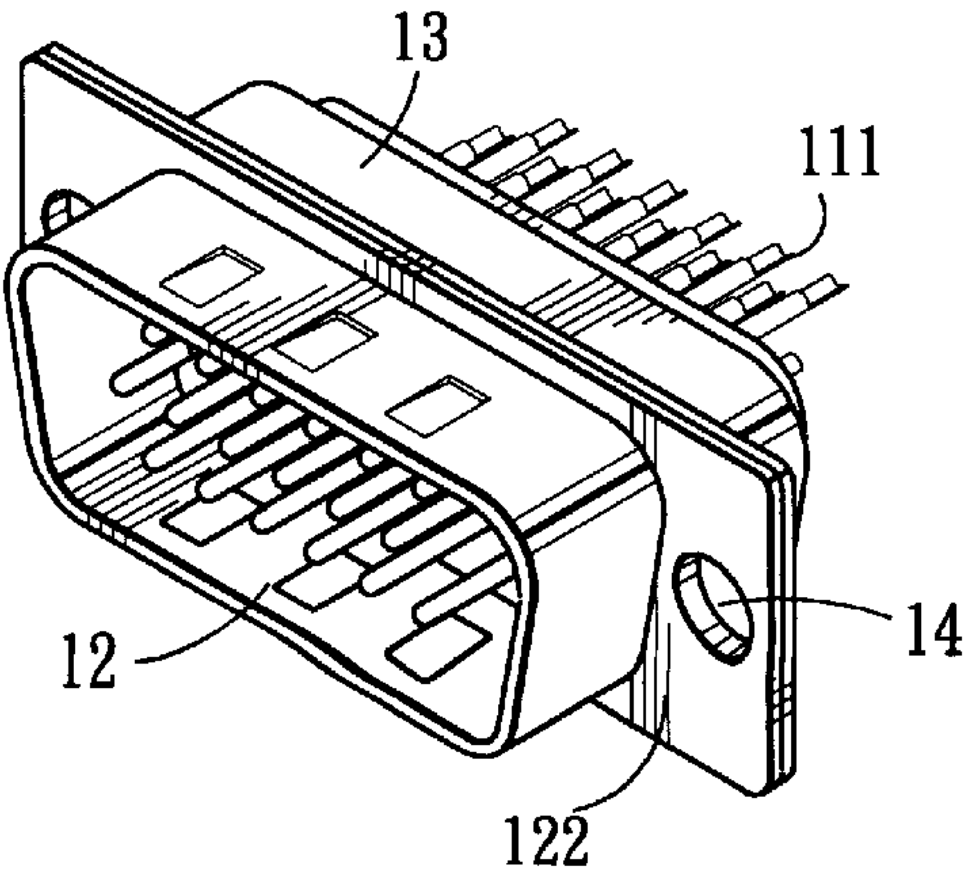
FIG. 2 PRIOR ART
