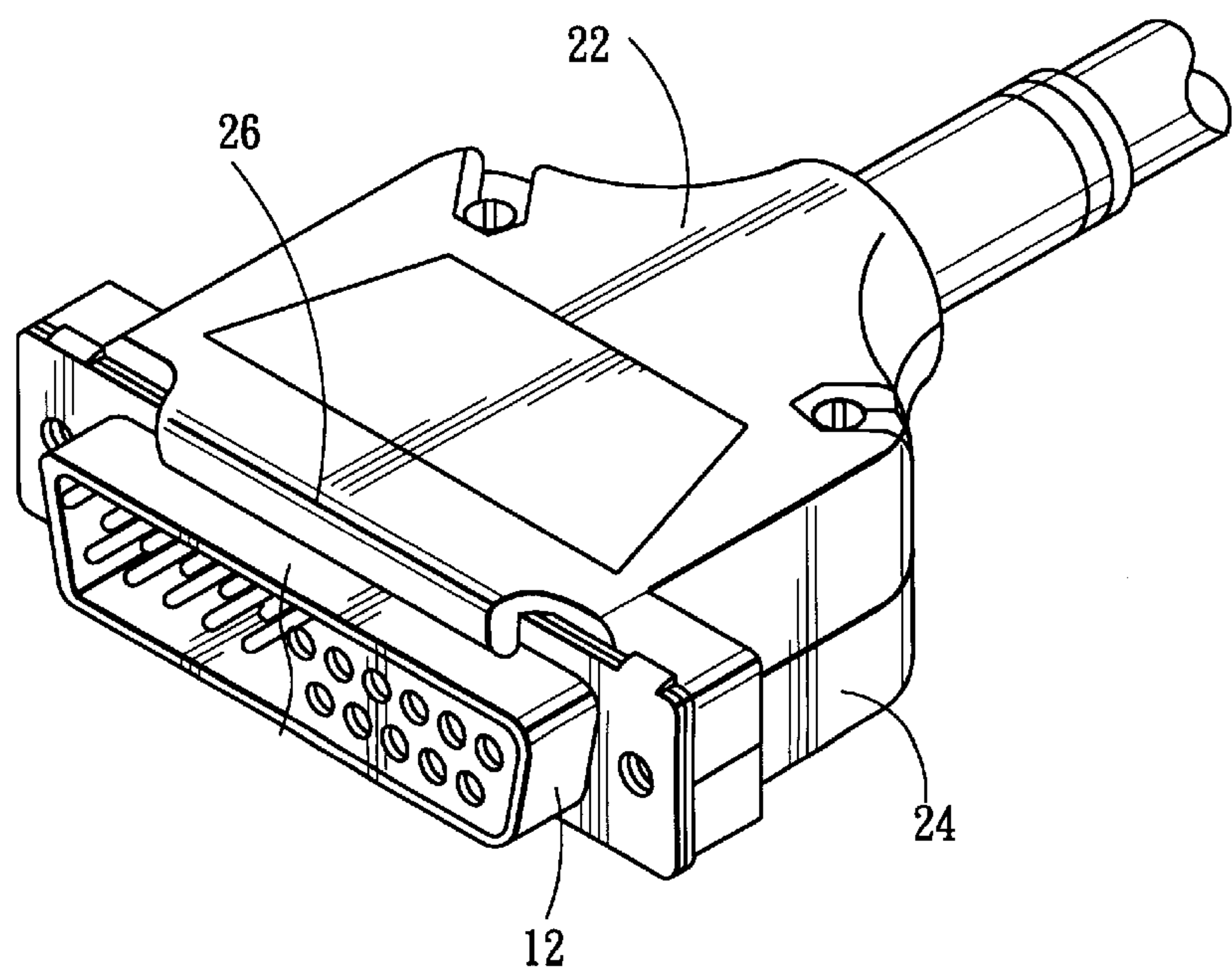
FIG. 8 PRIOR ART
