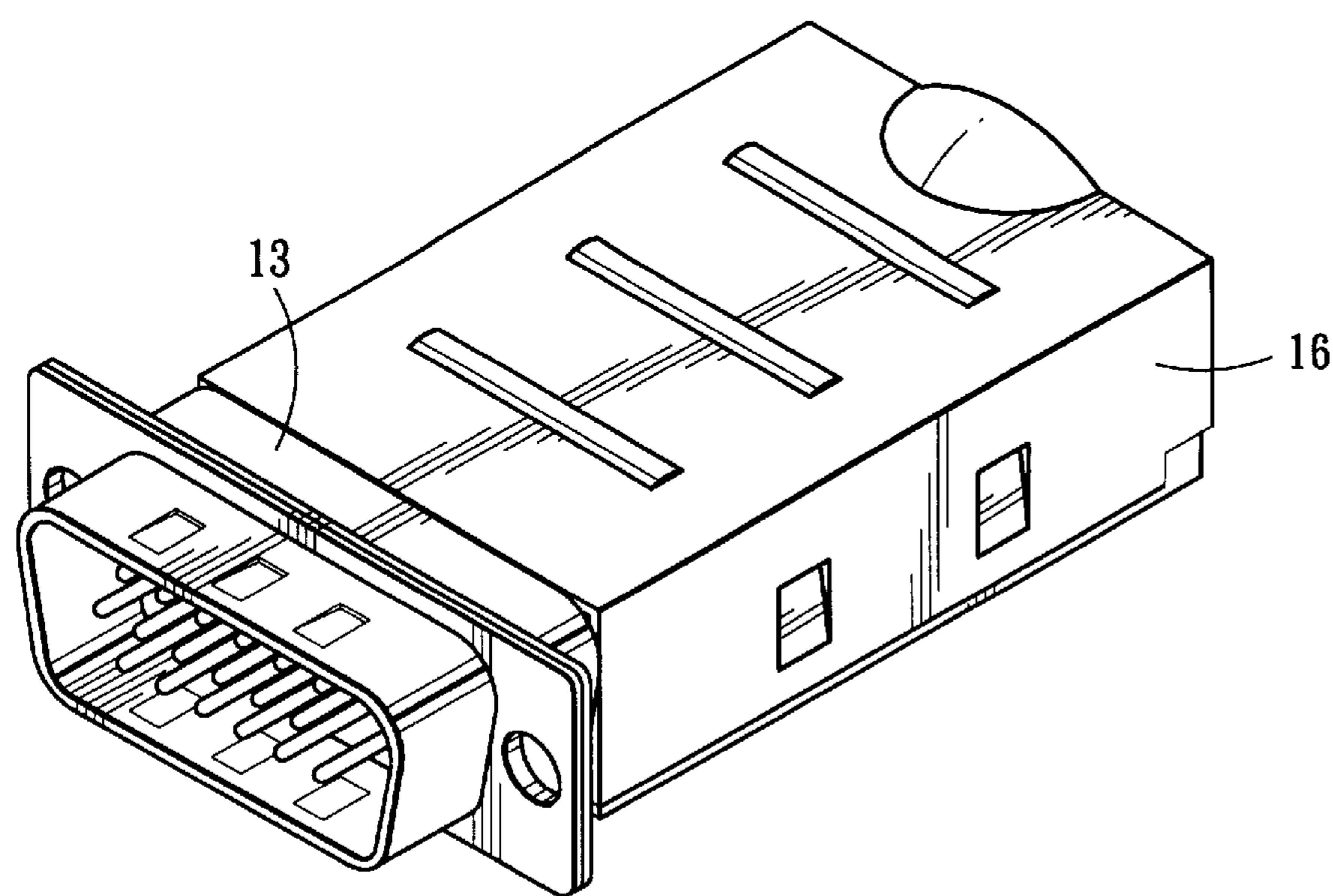
FIG. 6 PRIOR ART
