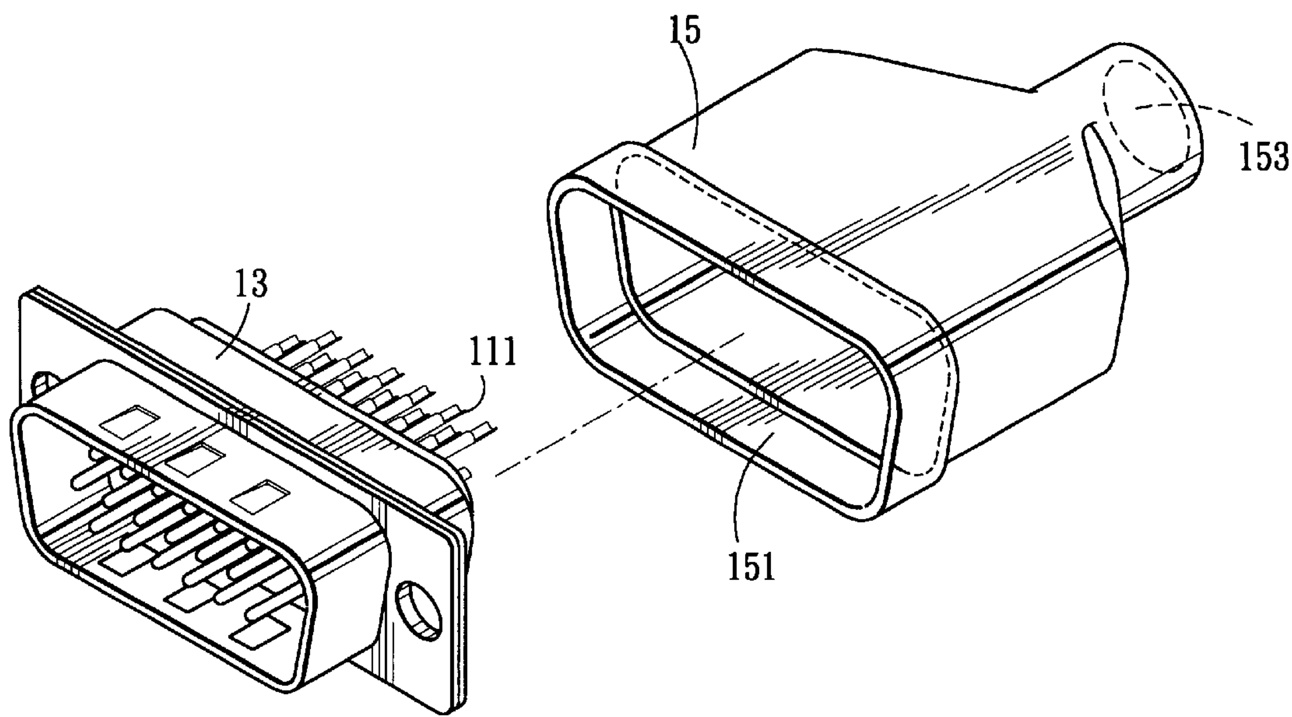
FIG. 3 PRIOR ART
