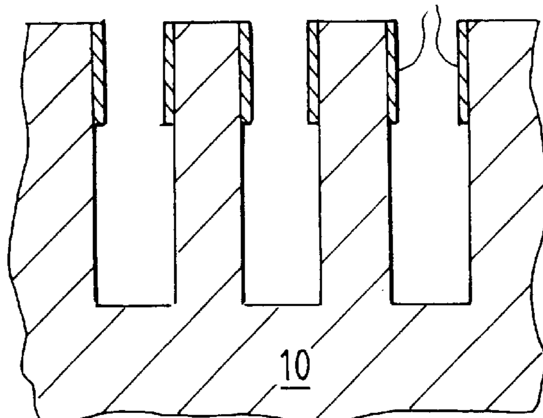
FIG. 3b PRIOR ART 26
