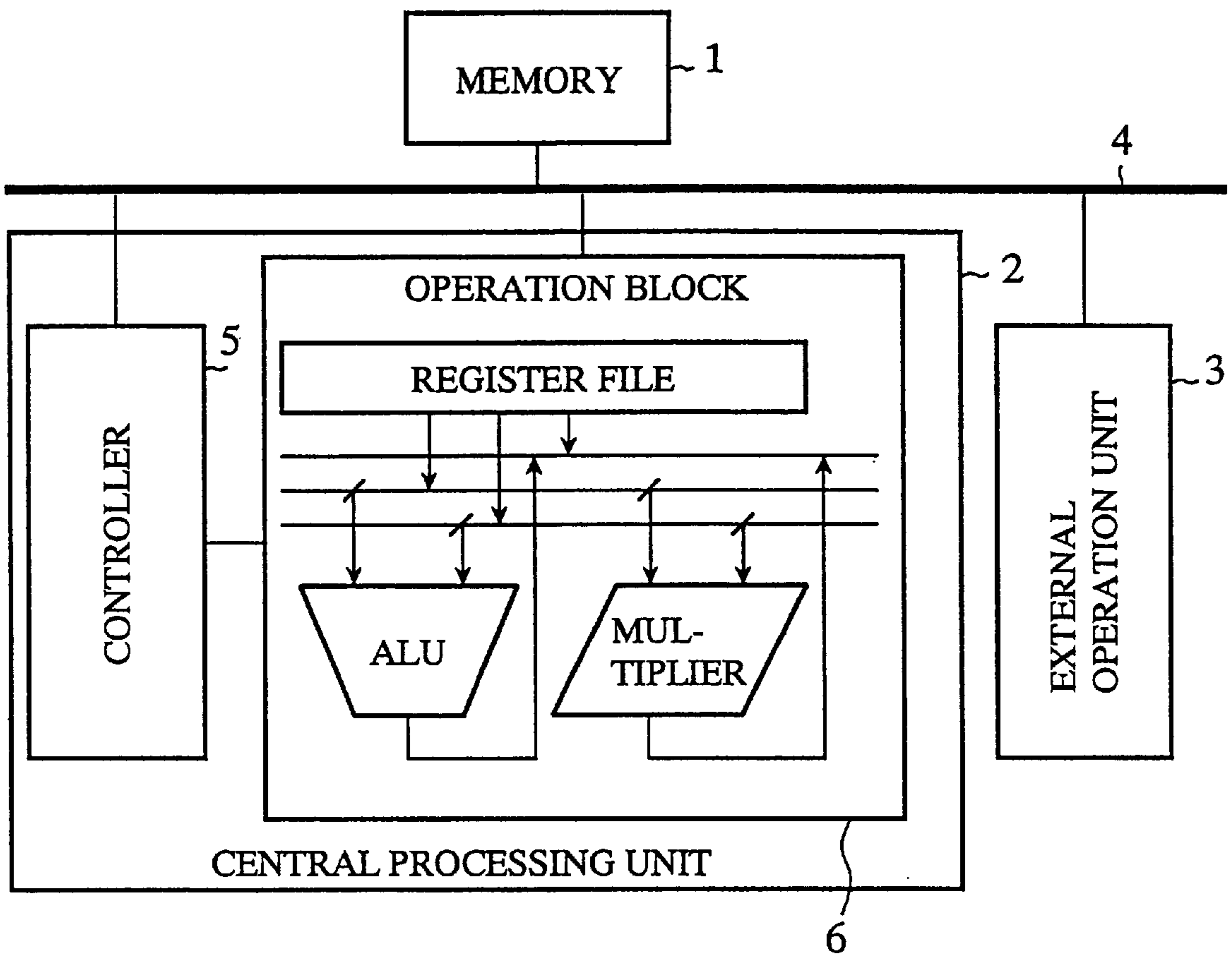
FIG.12 (PRIOR ART)
