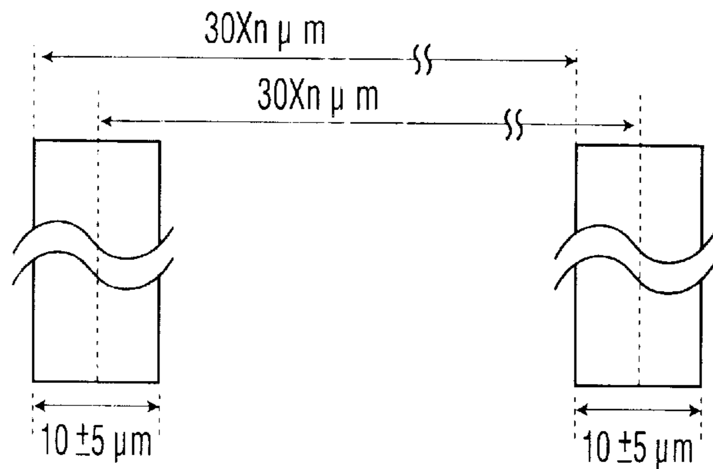
DIMENSIONAL ACCURACY OF SLIT (AT r=22.2\text{mm} )
