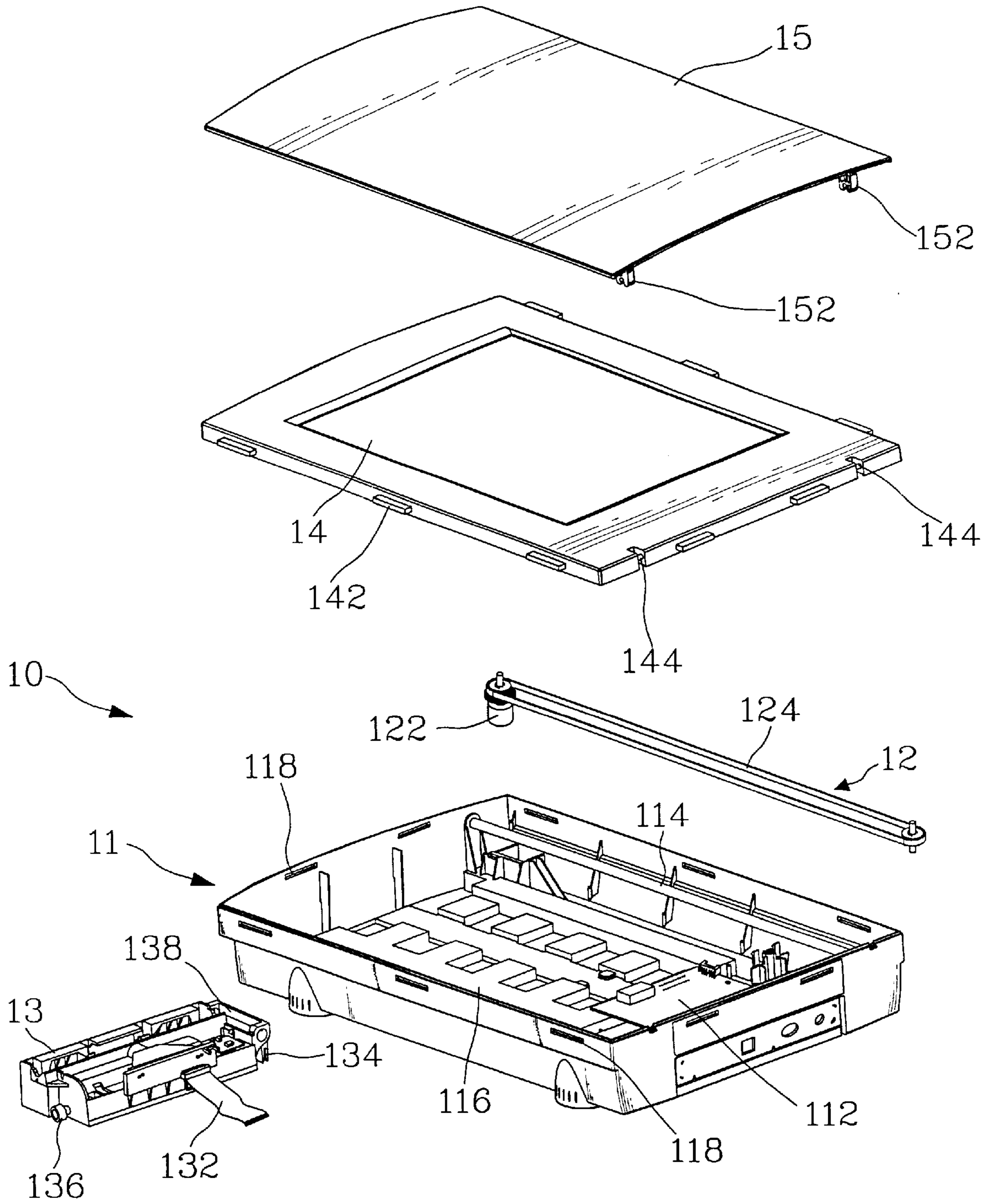
FIG. 1 (PRIOR ART)
