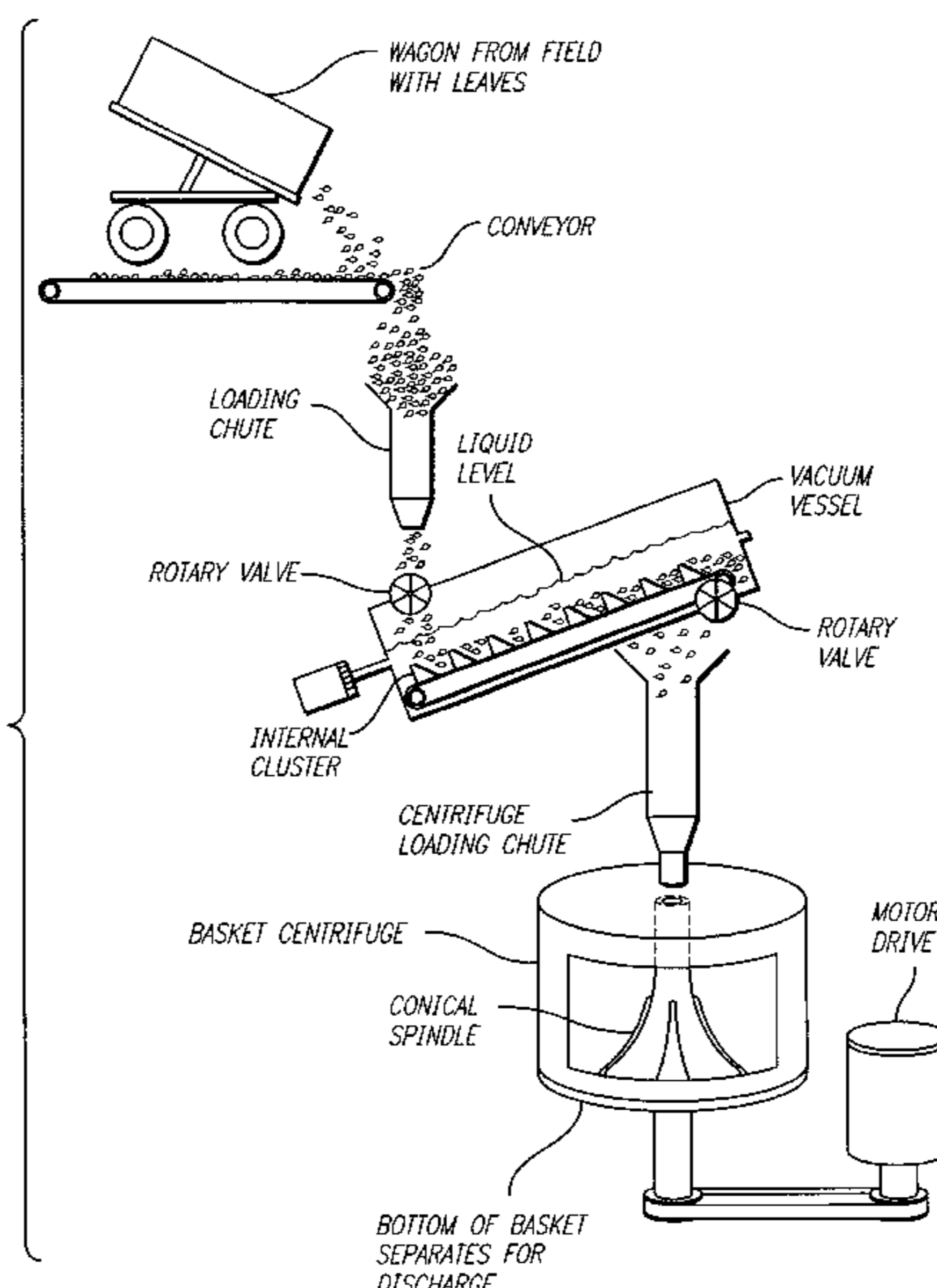
CONTINUOUS VACUUM INFILTRATION
