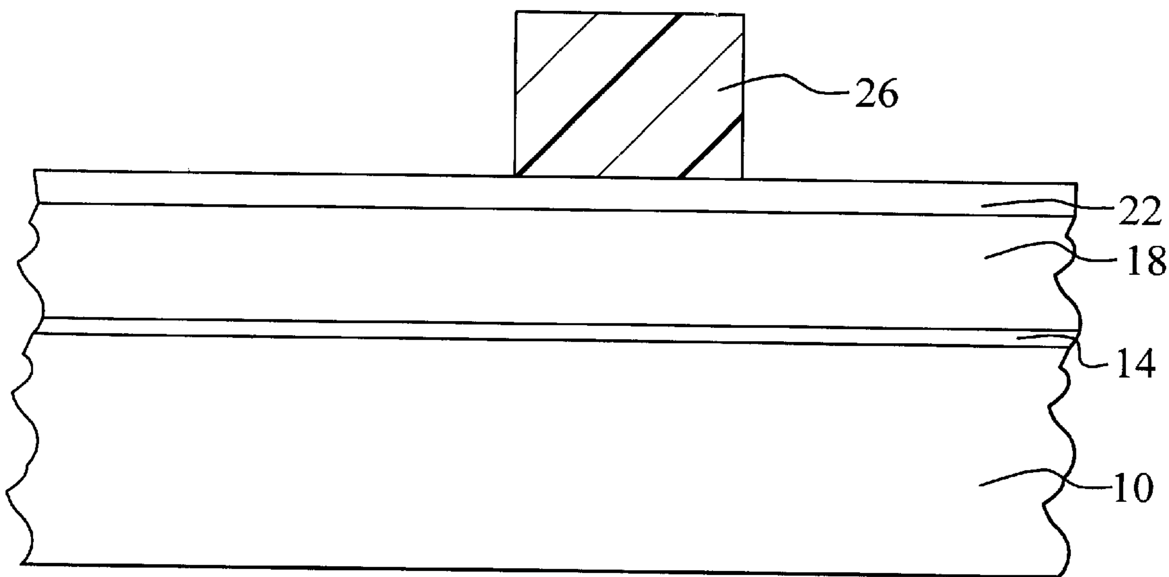
FIG. 1 Prior Art
