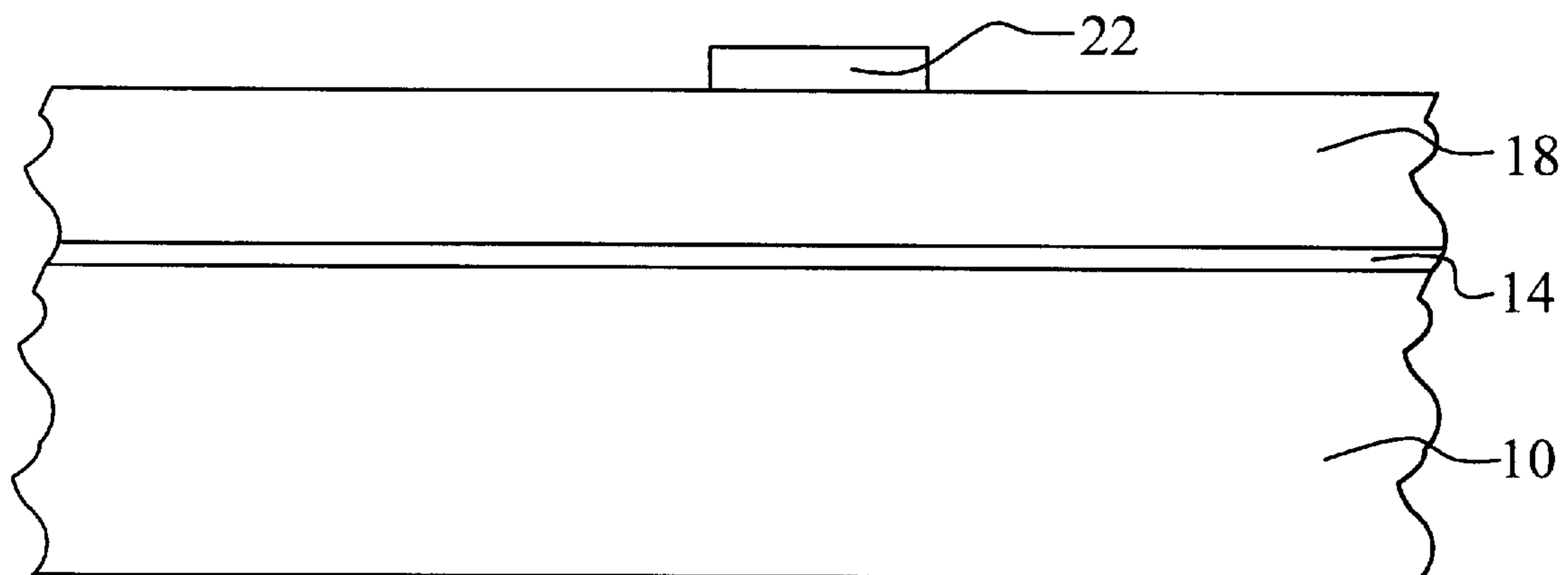
FIG. 4 Prior Art
