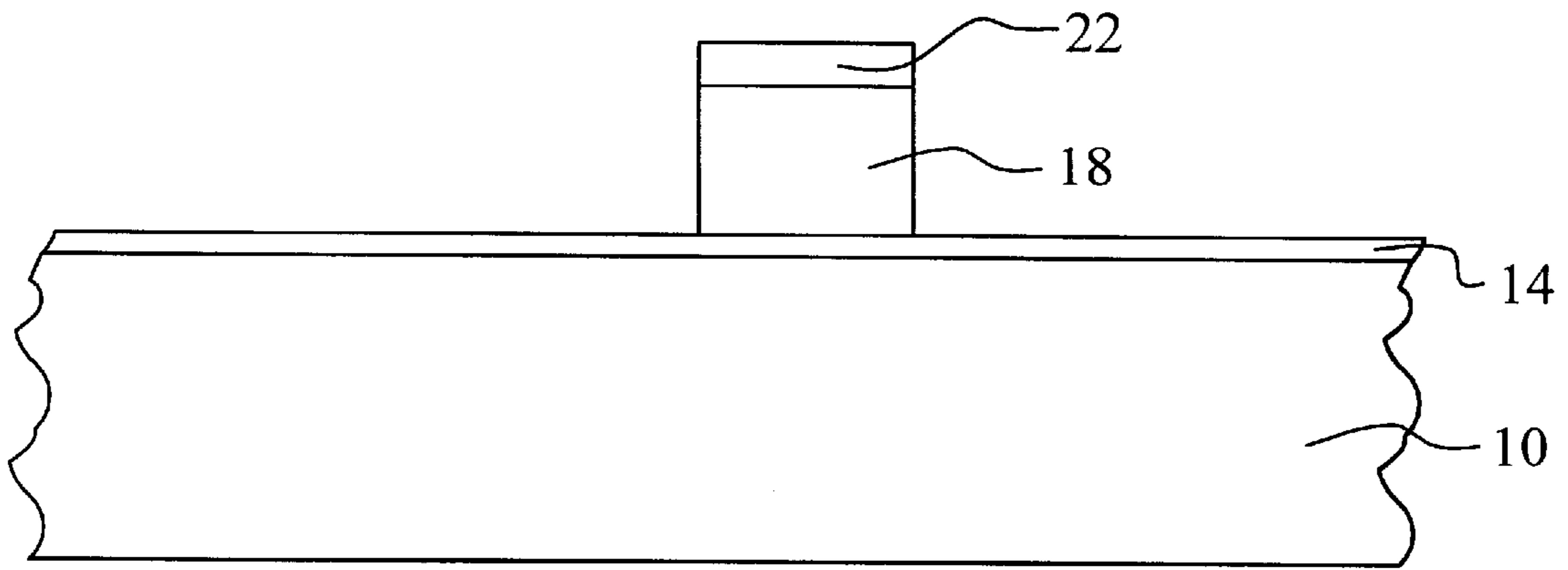
FIG. 5 Prior Art
