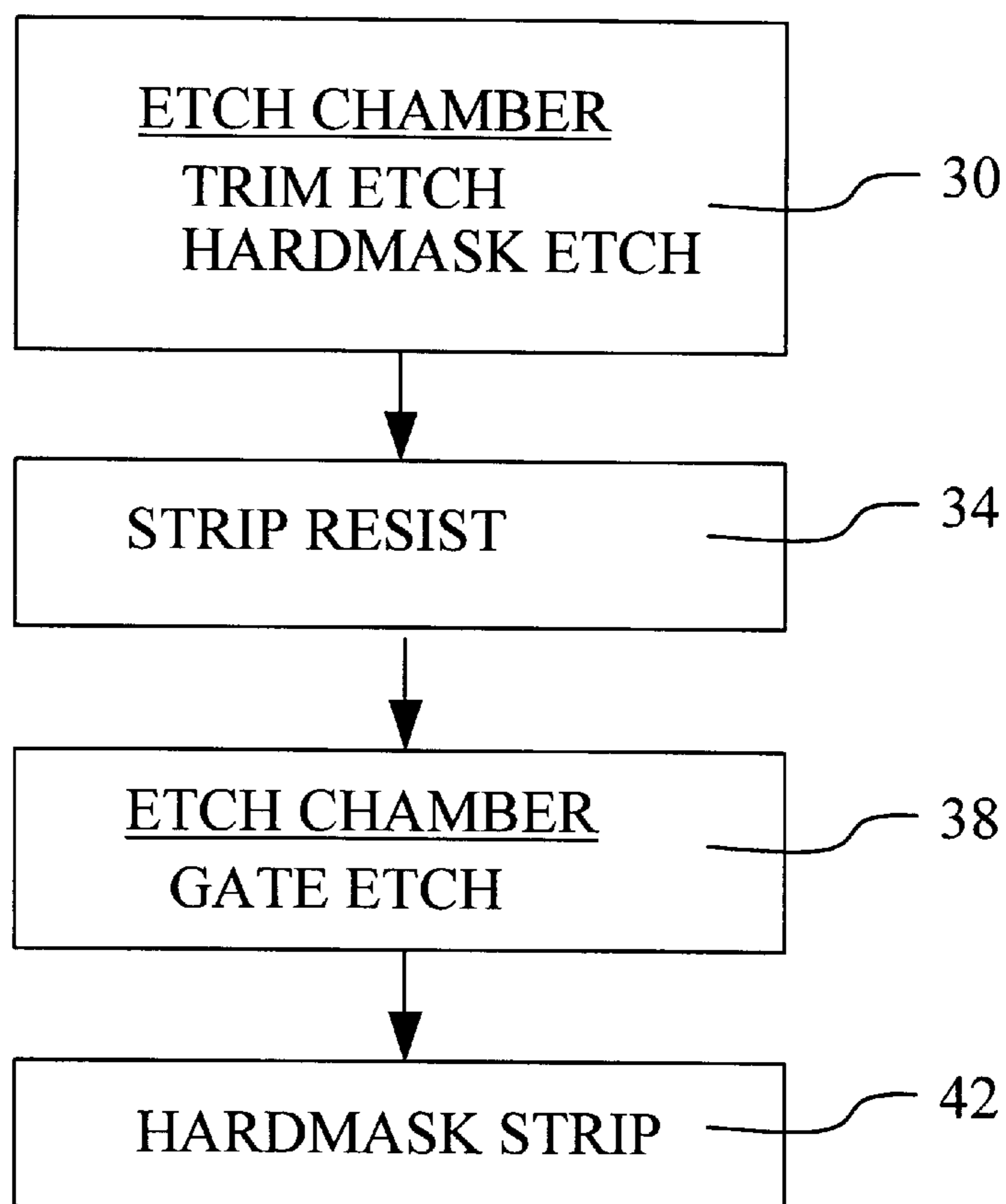
FIG. 7 Prior Art
