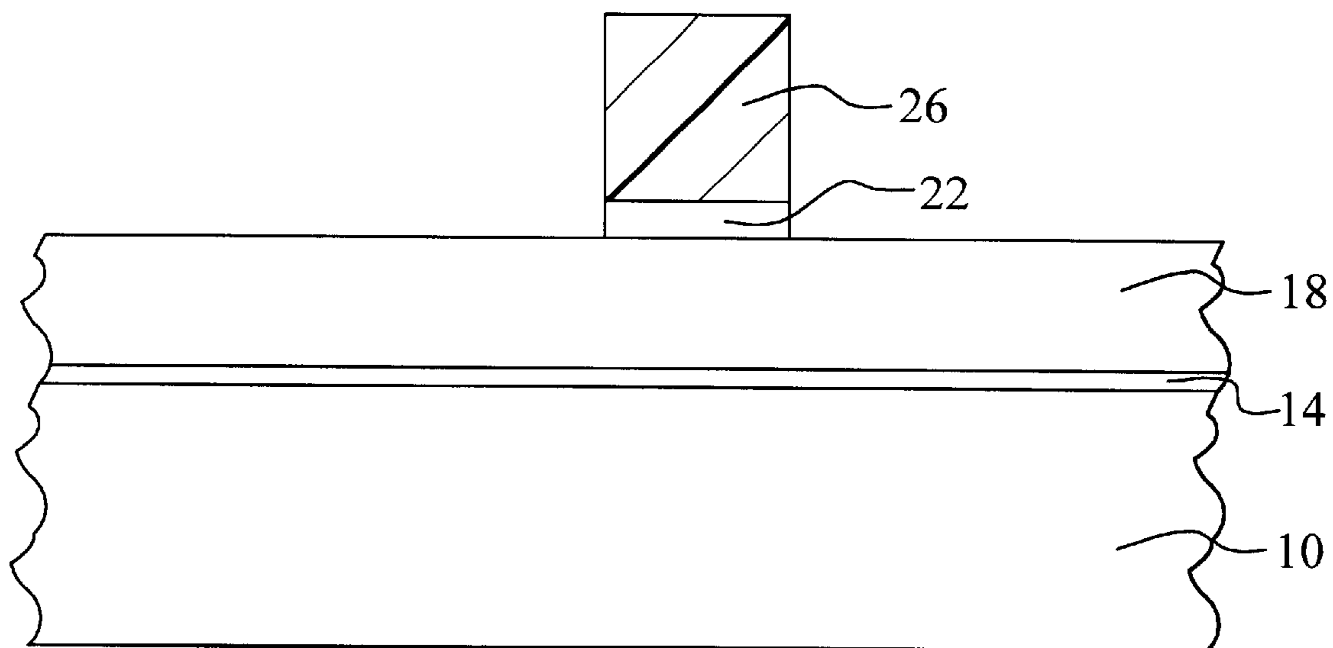
FIG. 3 Prior Art
