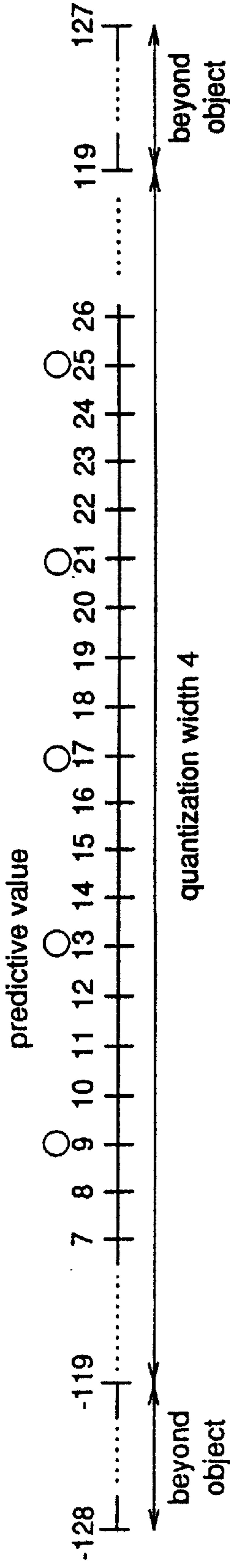
Fig.32 (a) linear quantization representative value
