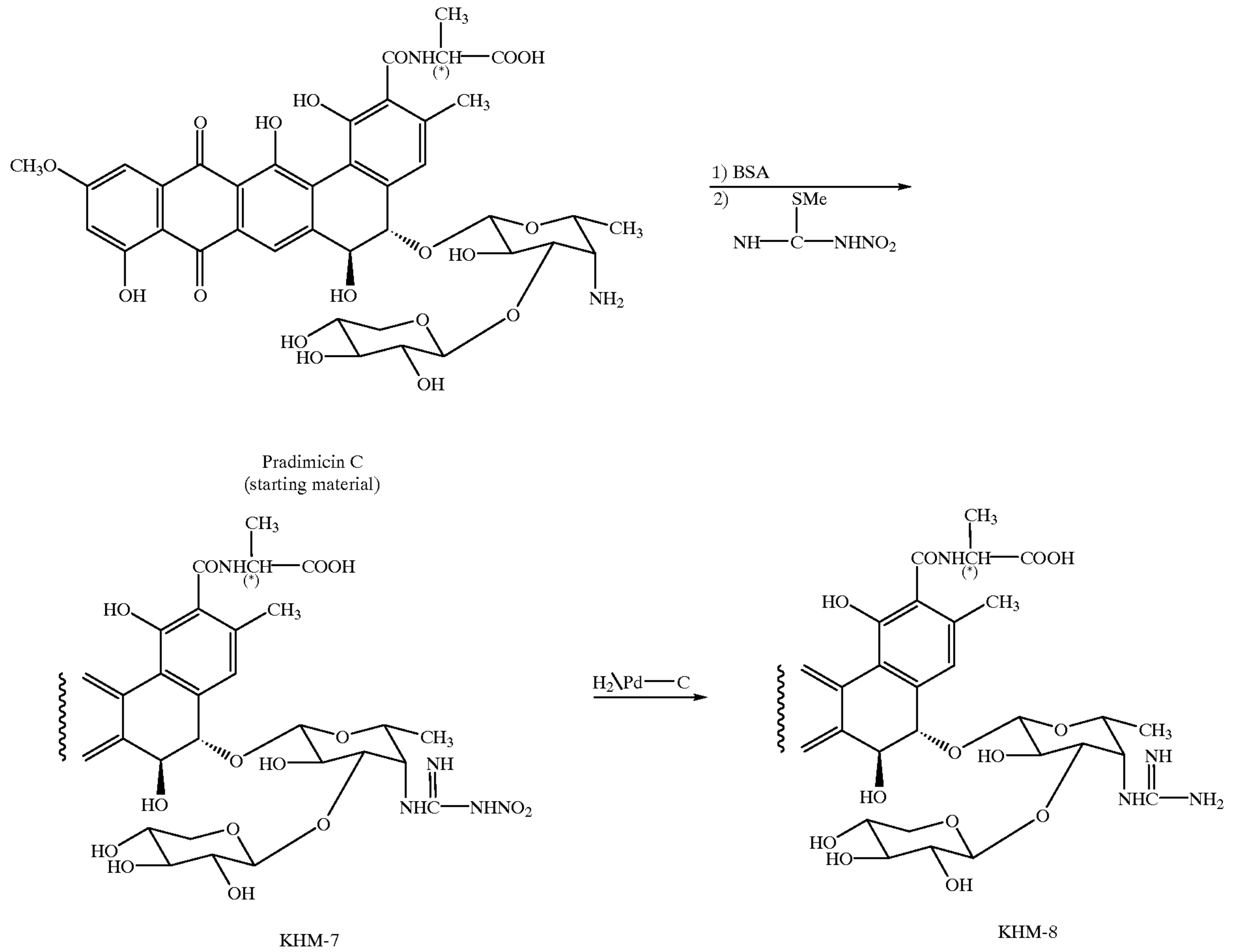
Scheme 2
