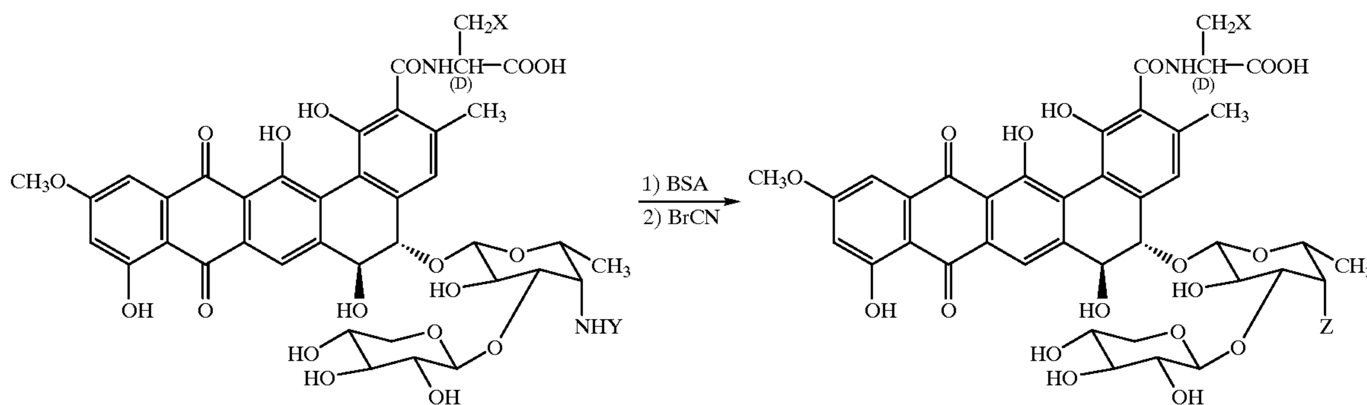
Scheme 1
