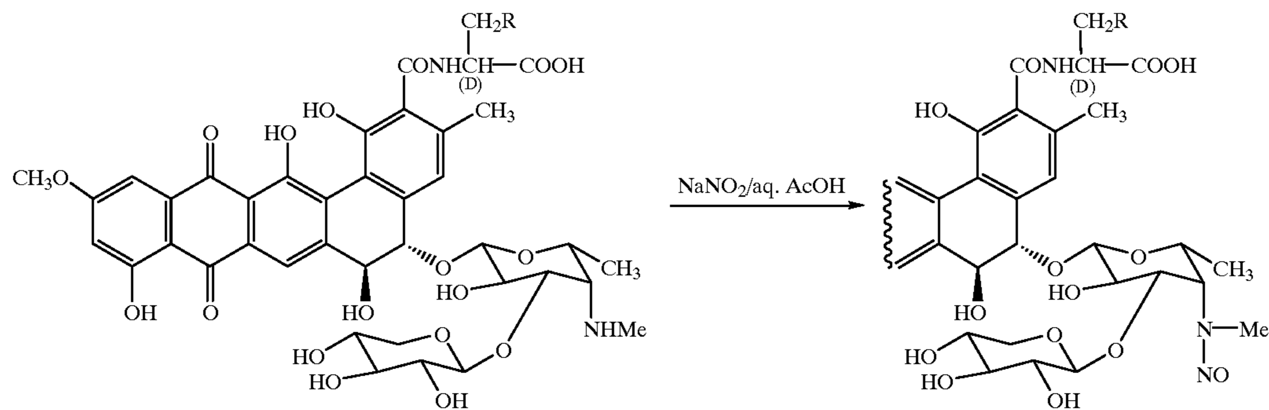
Scheme 4
