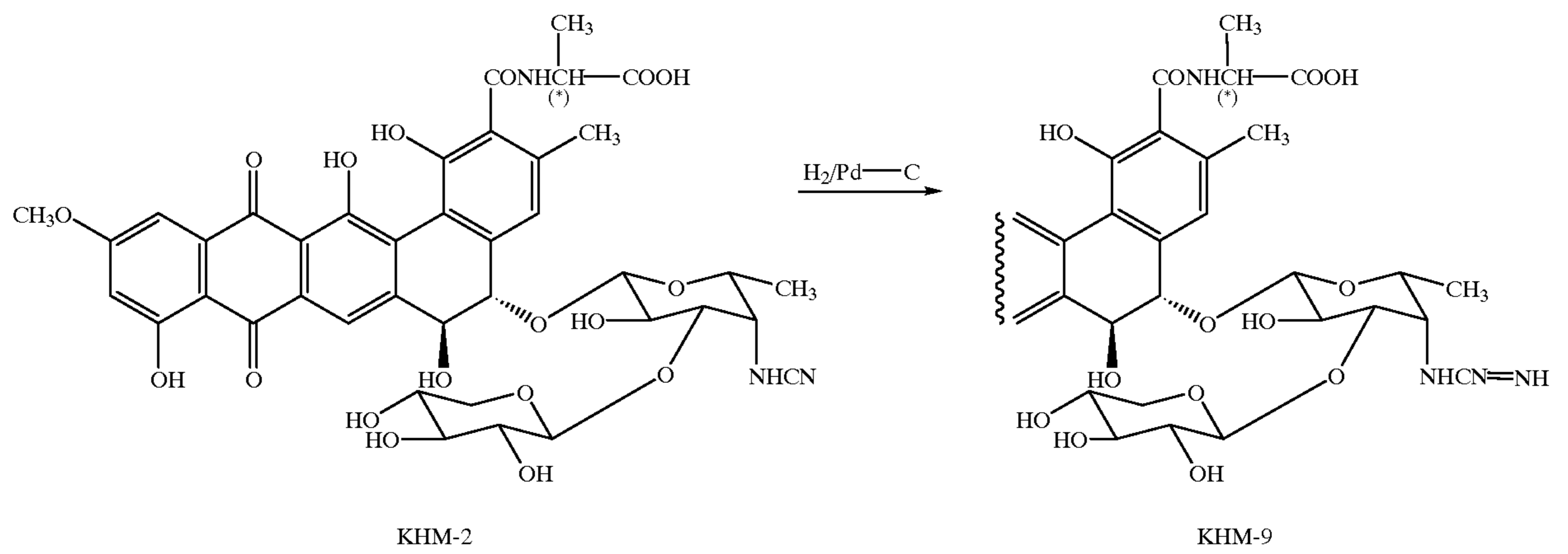
Scheme 3
