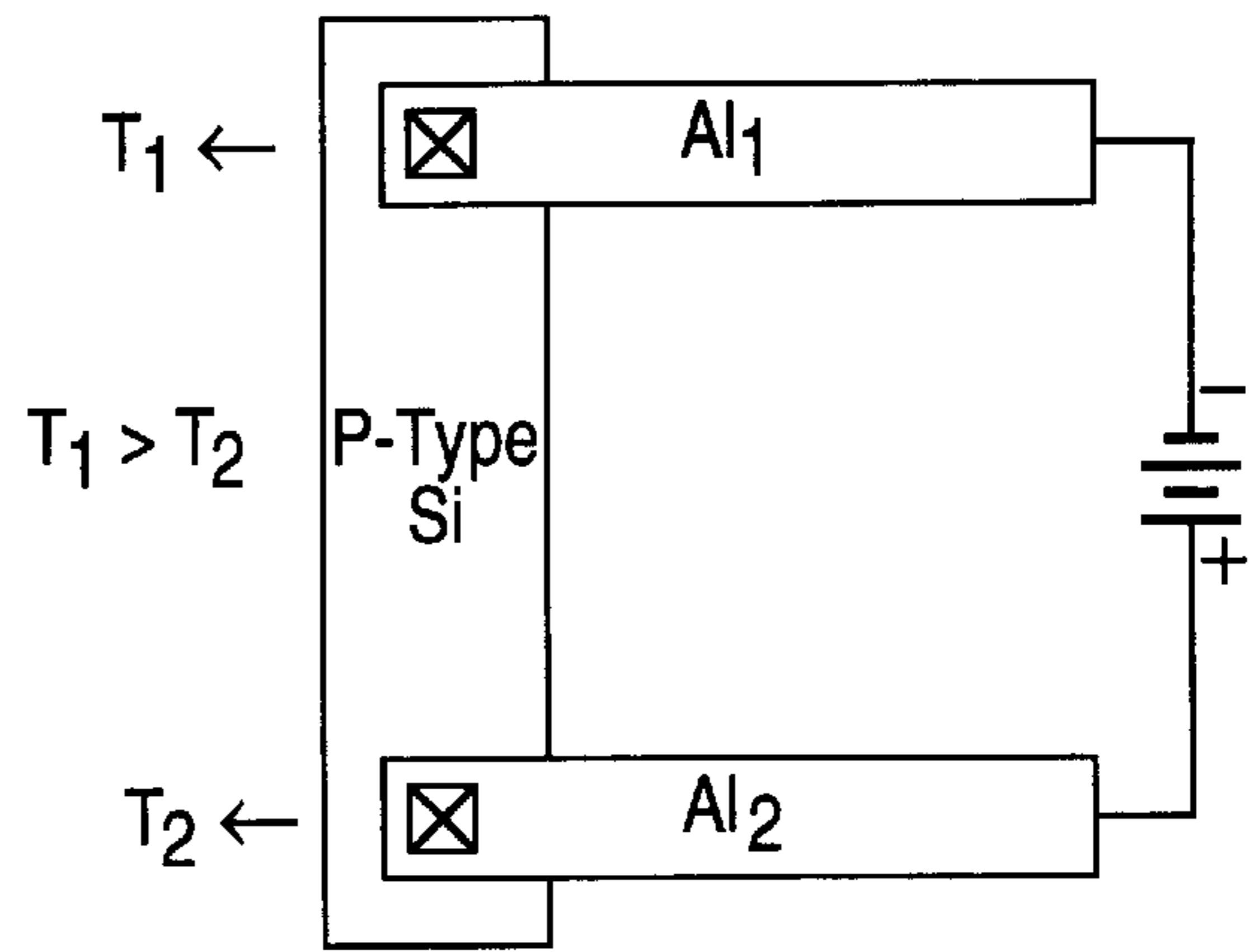
FIG. 2 (PRIOR ART)
