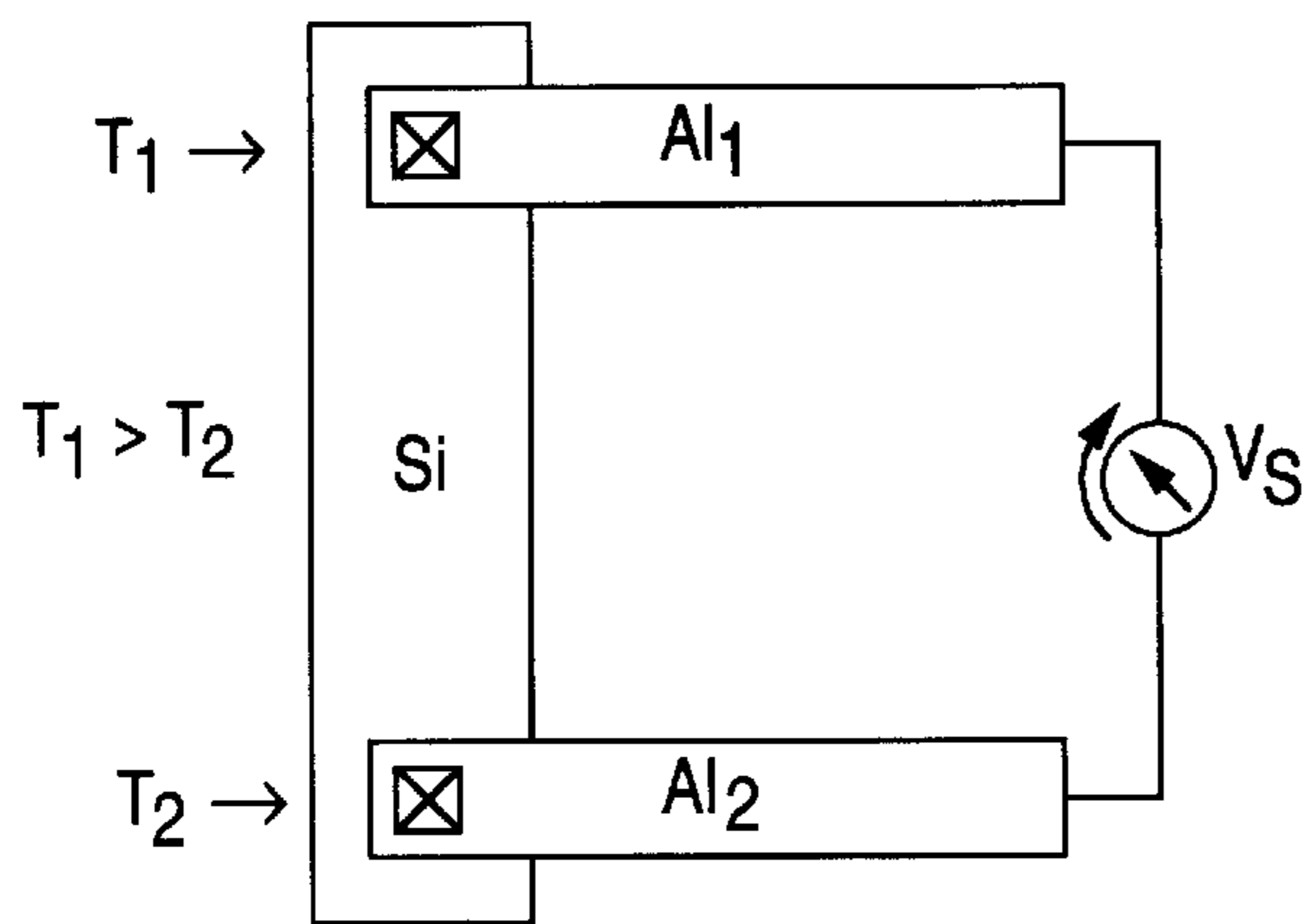
FIG. 1 (PRIOR ART)
