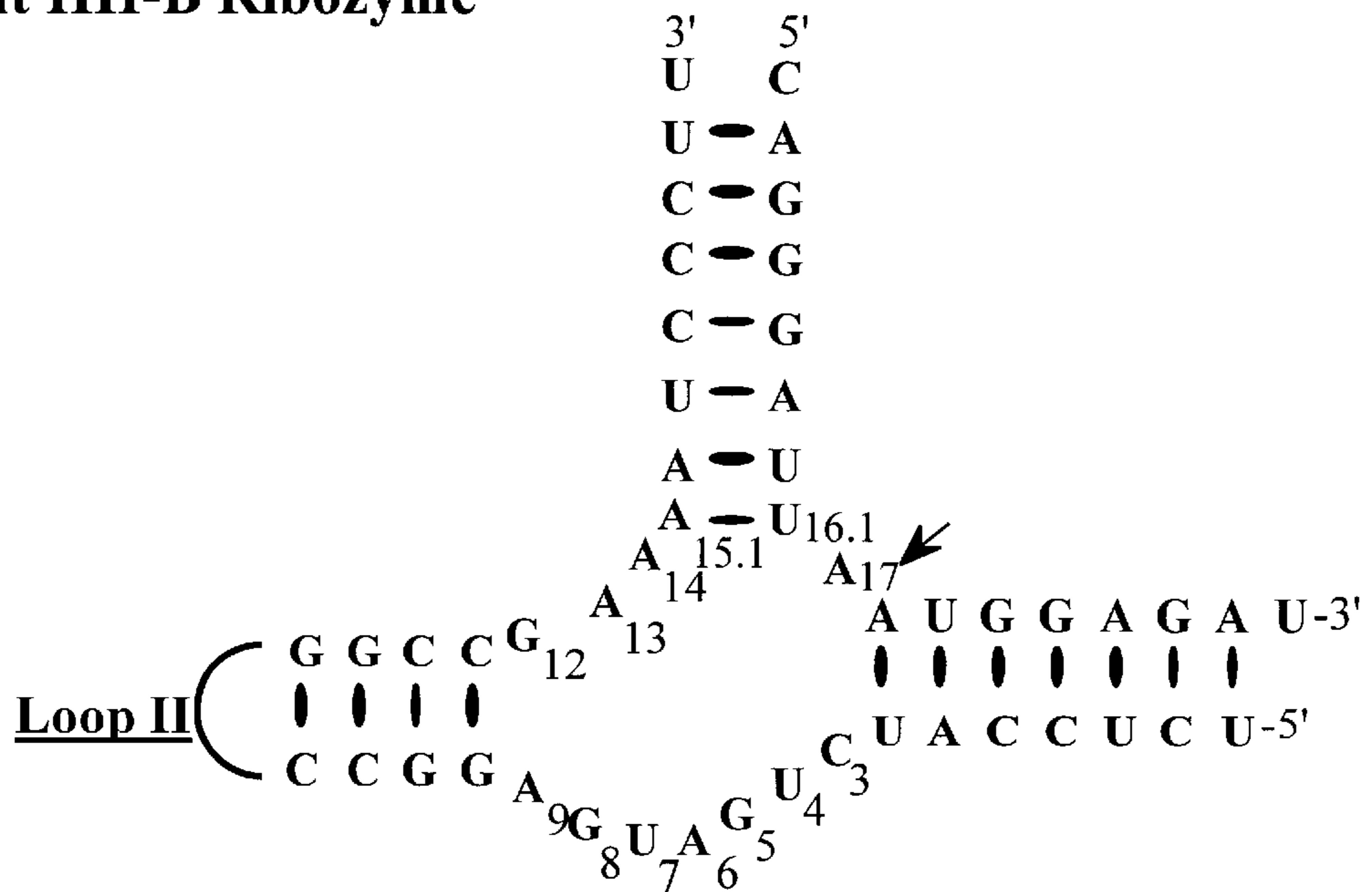
Figure 16: RNA Cleavage by Loop II
