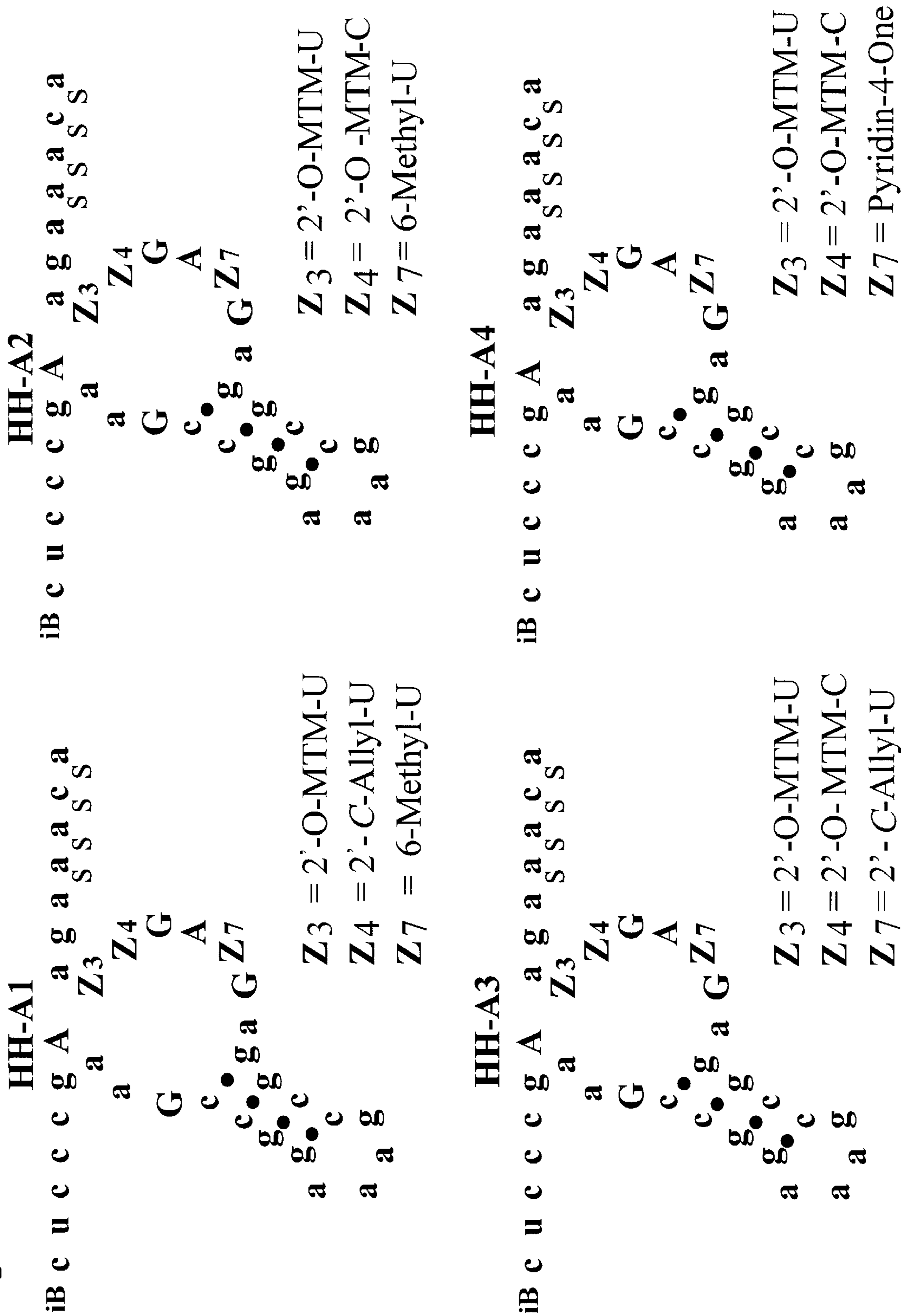
Figure 11A: HH-A Variants
