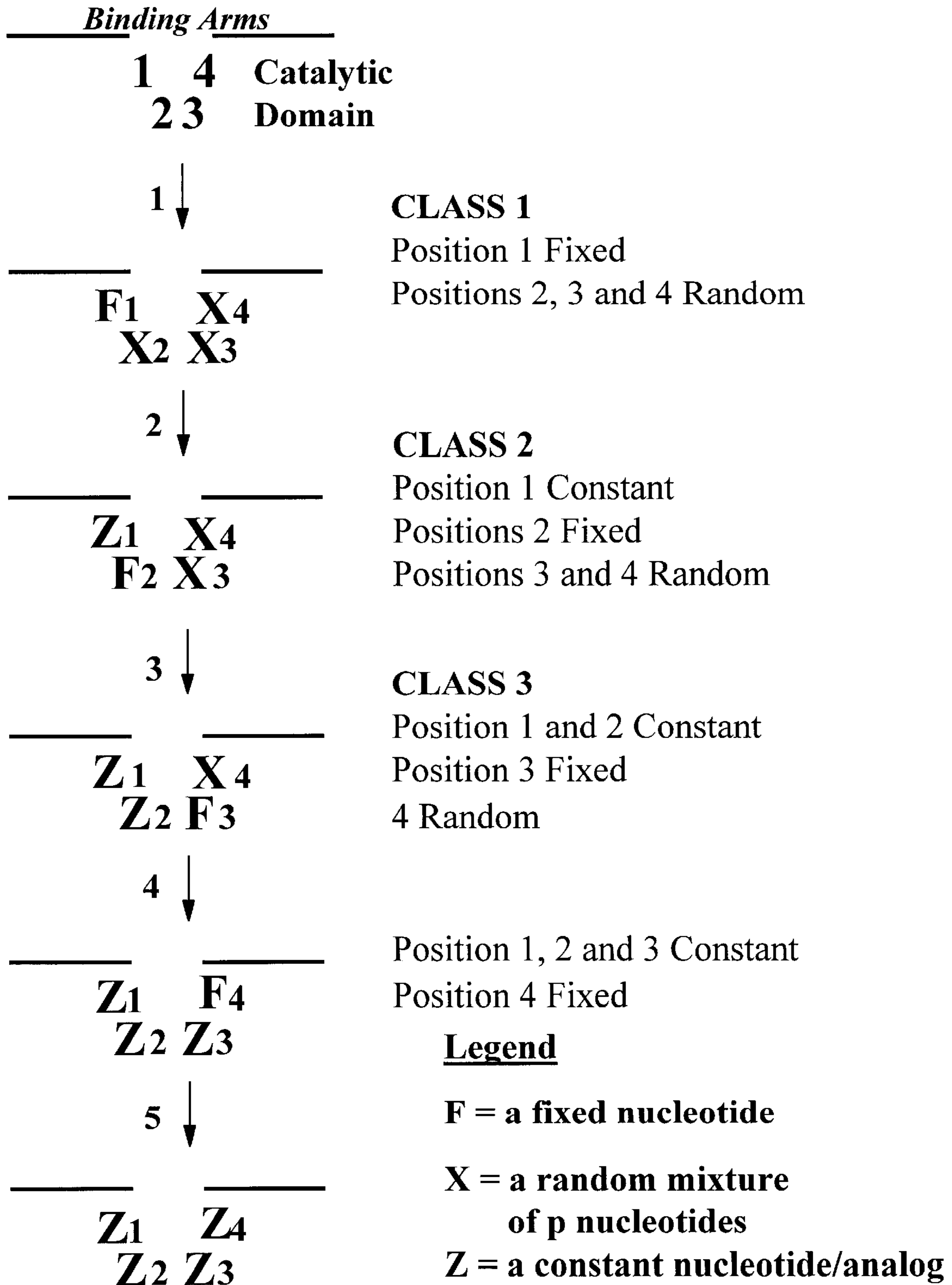
Figure 18: Screening for Ribozyme Catalytic Domains
