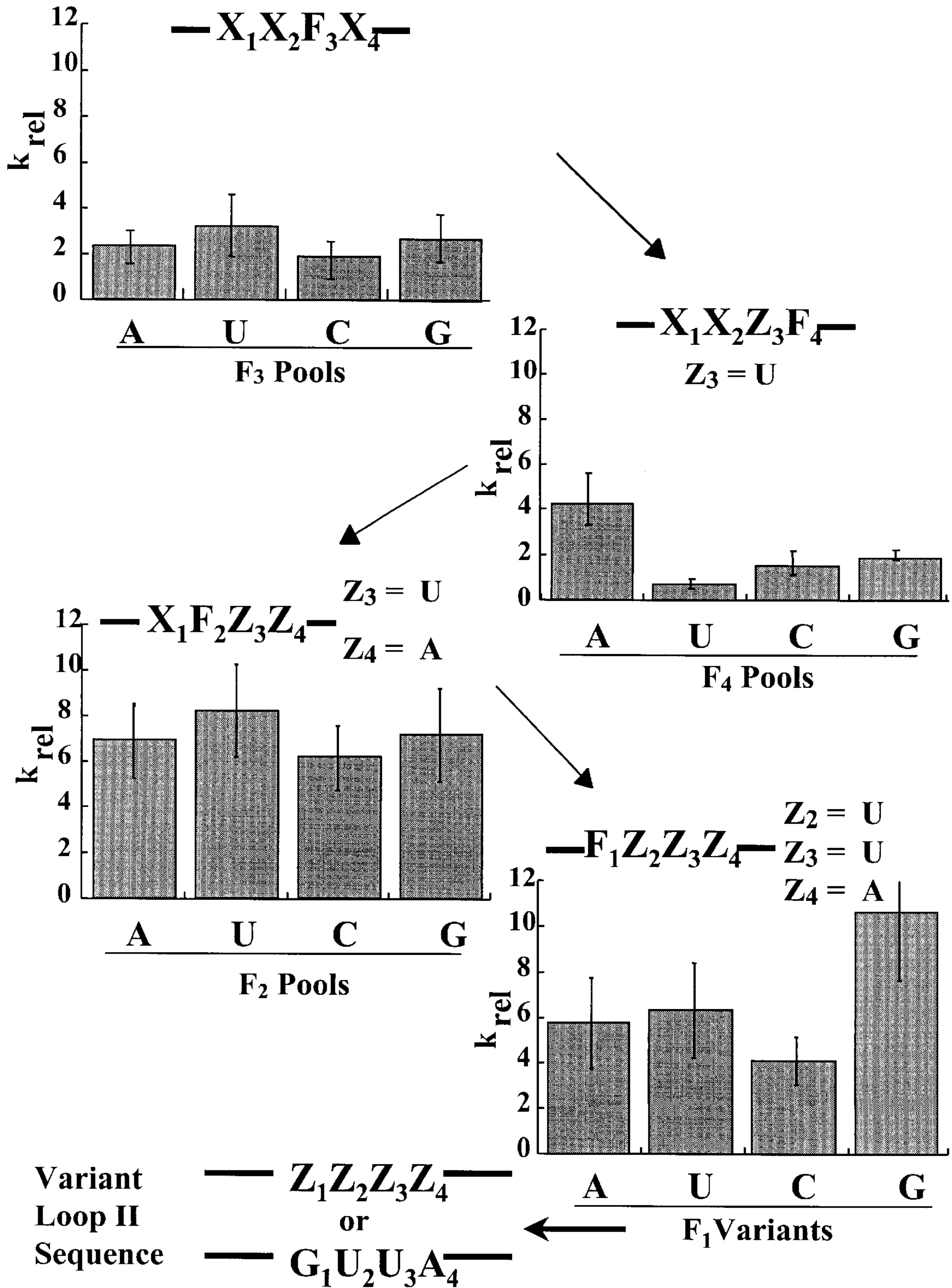
Figure 15: Activity of HH-B Variant Ribozymes
