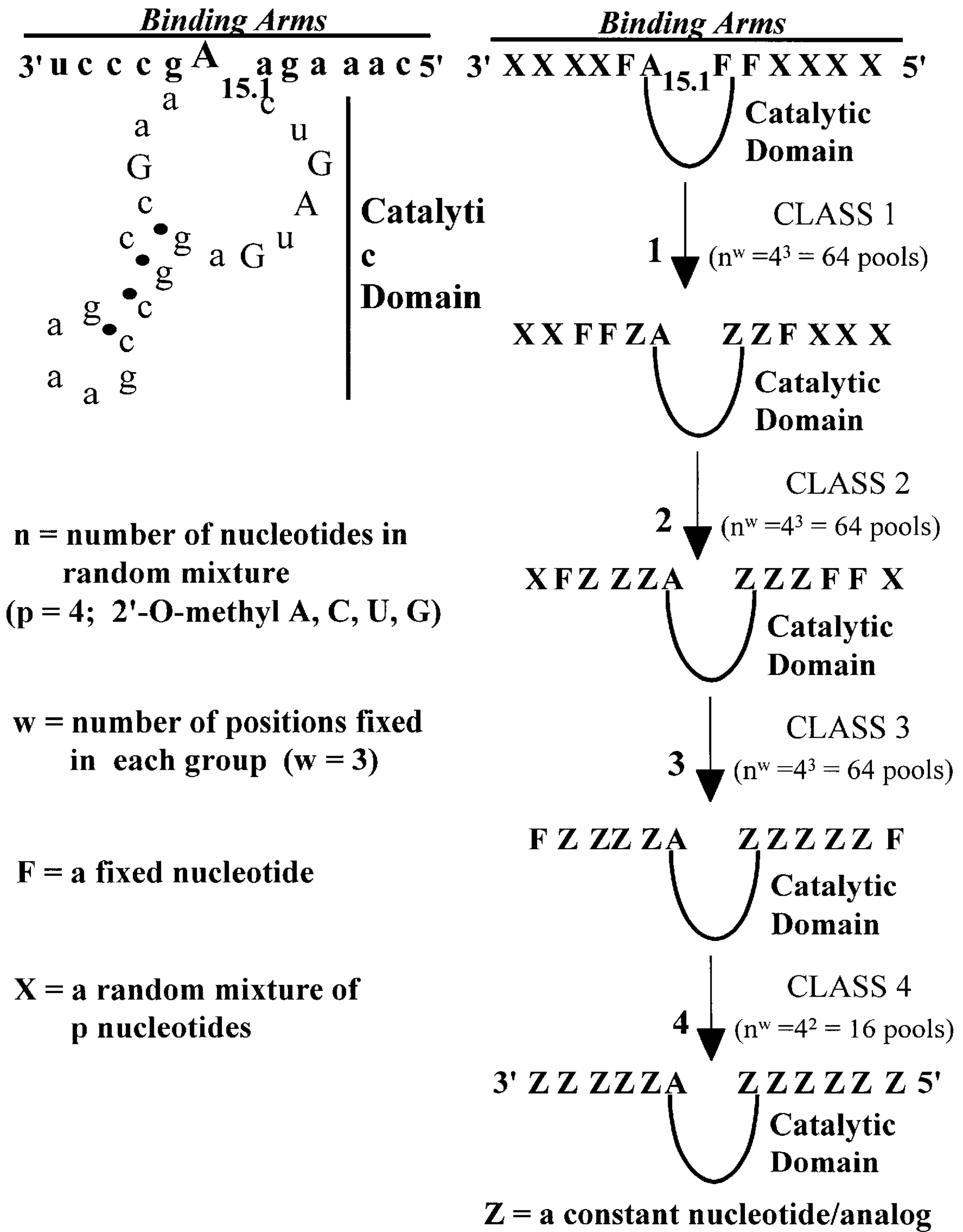
Figure 17: Screening for Ribozyme Binding Arm Sequence Variants-Target Discovery Hammerhead Ribozyme Model System
