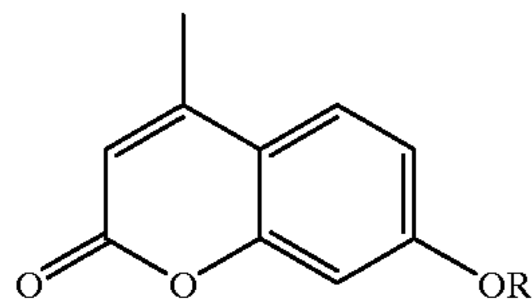
4-methyl umbelliferone wherein R =
