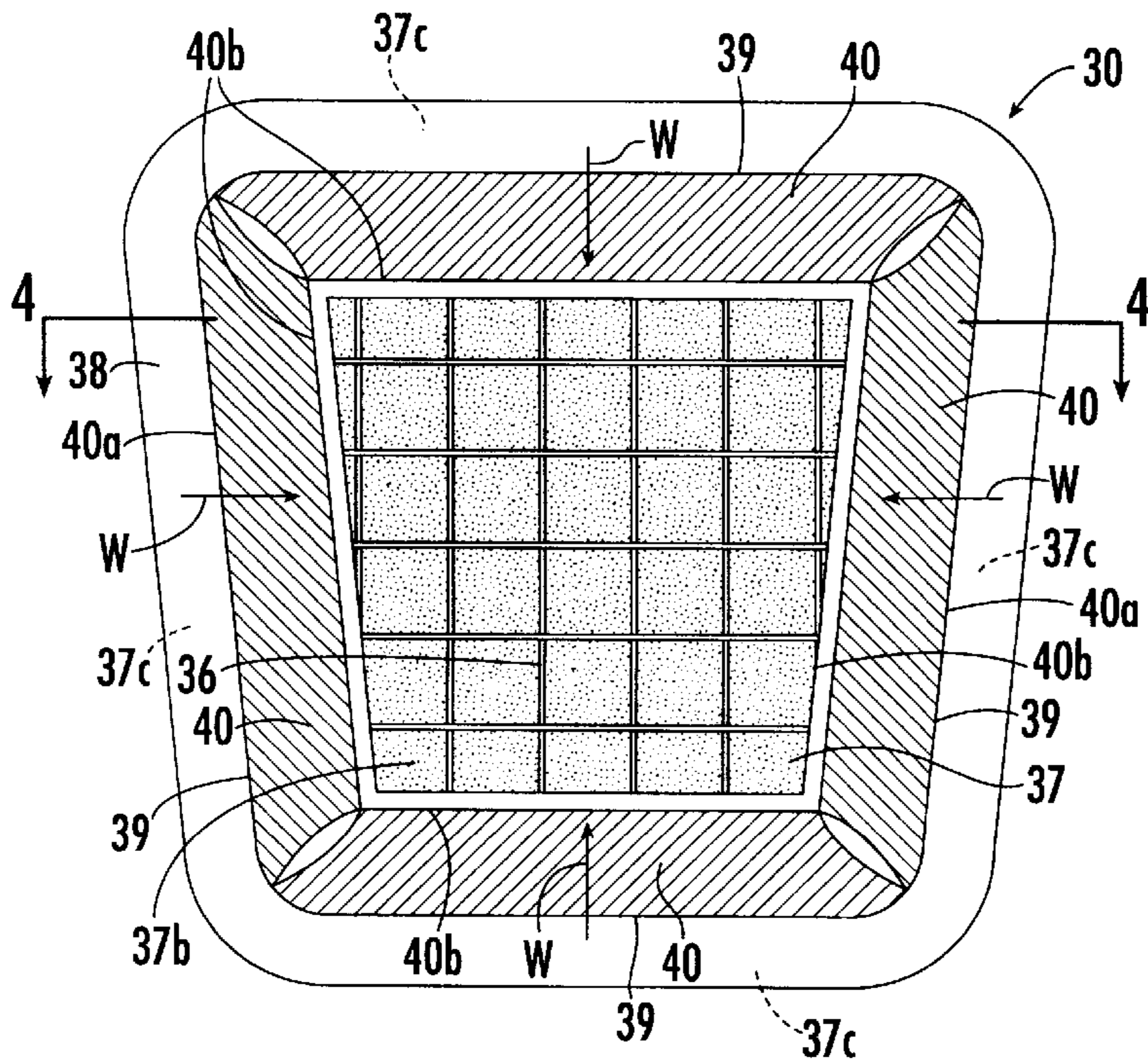
FIG. 2. (PRIOR ART)
