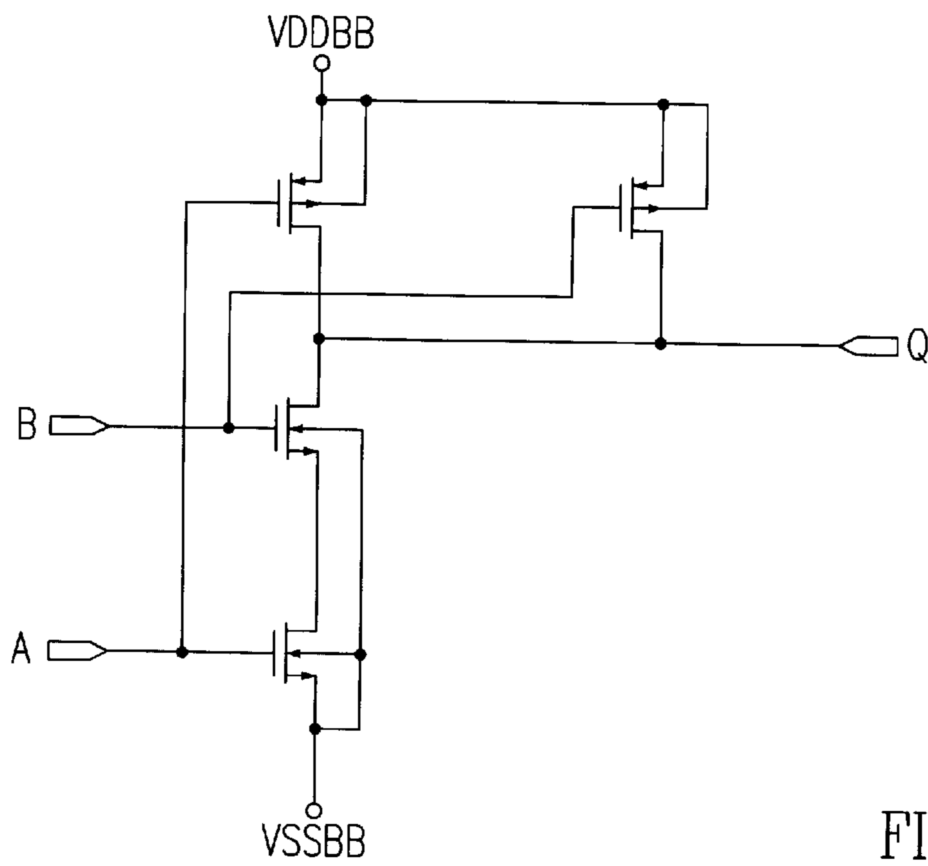
NAND2
