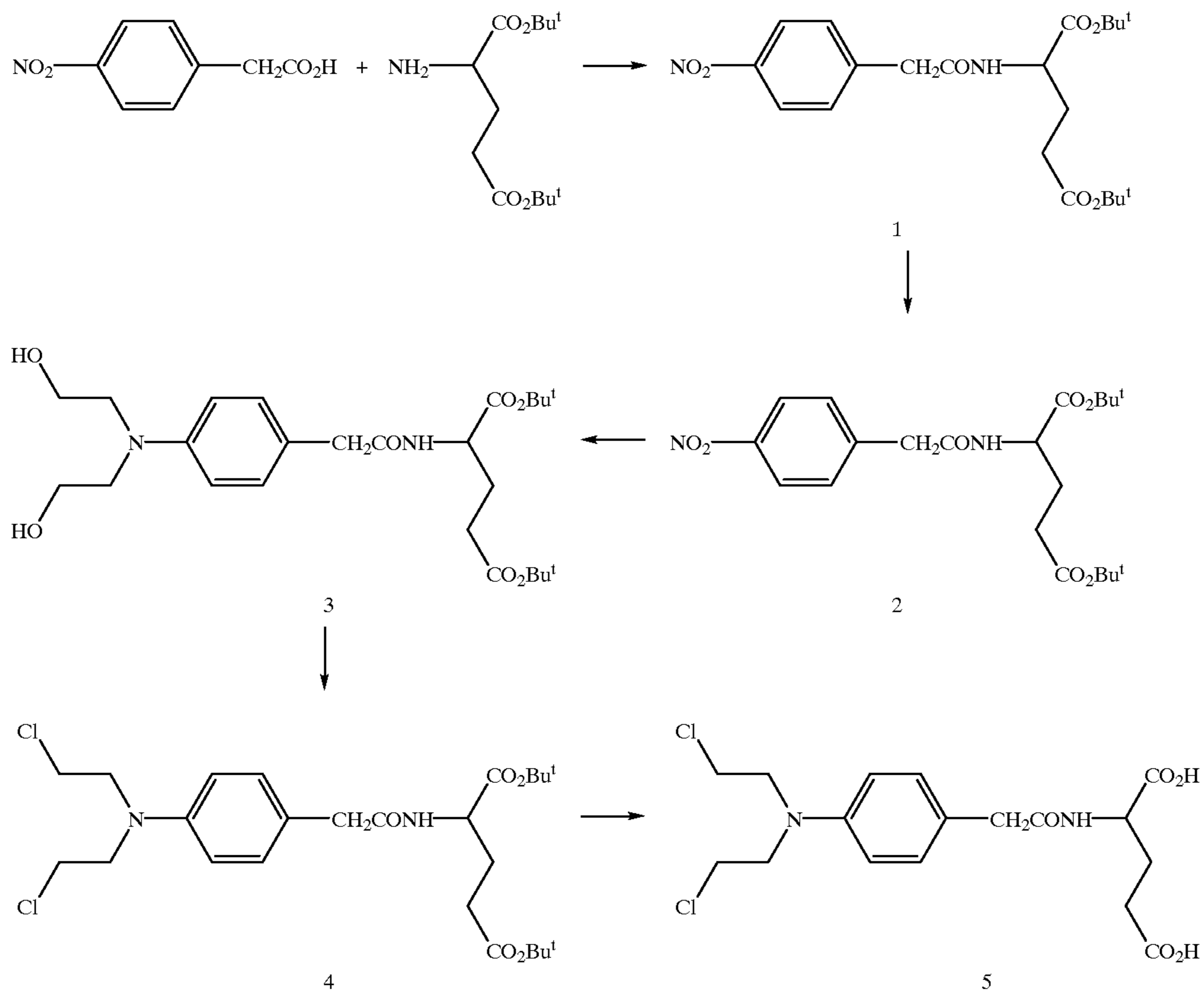
SCHEME 8
