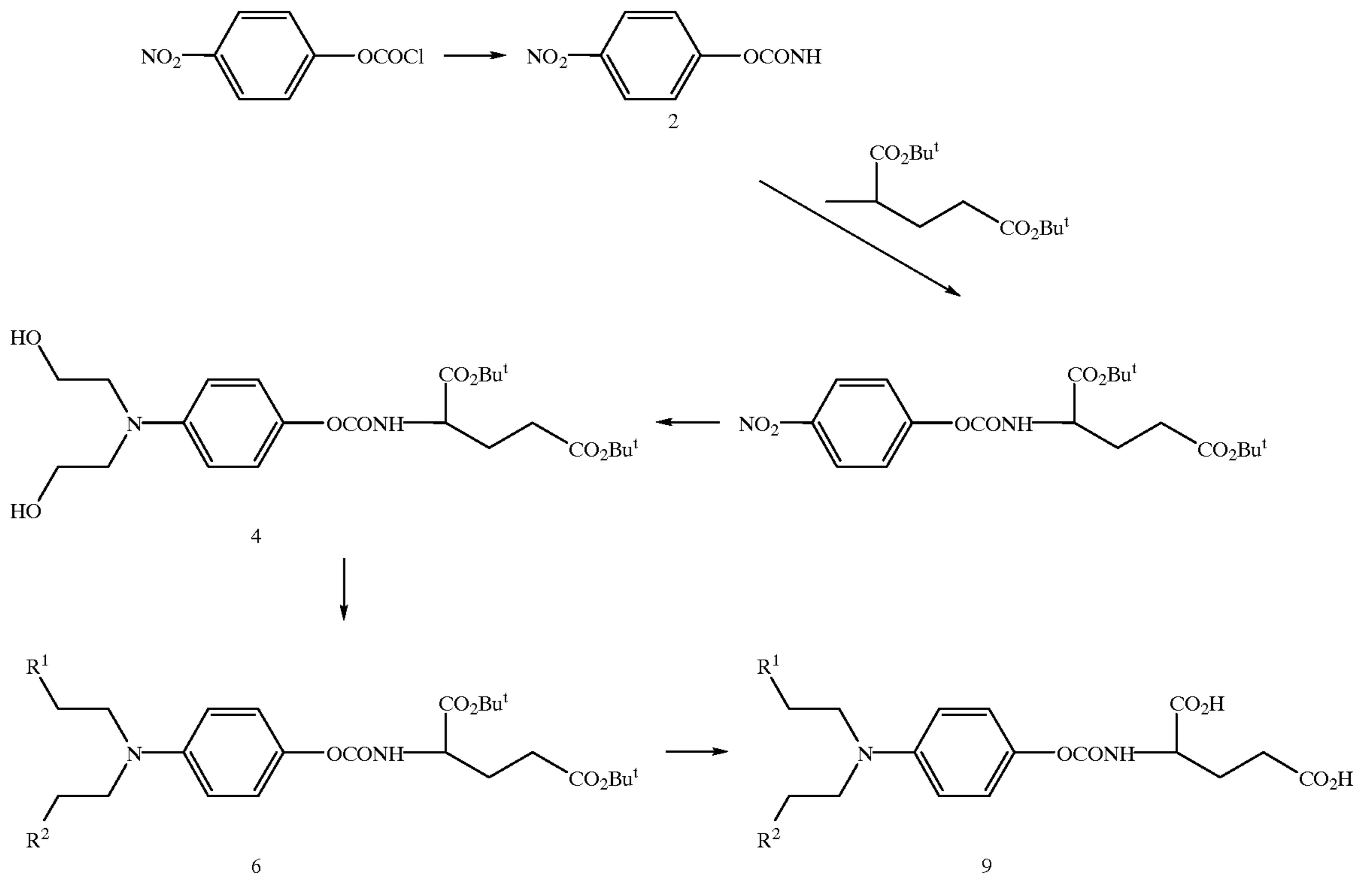
SCHEME 4
