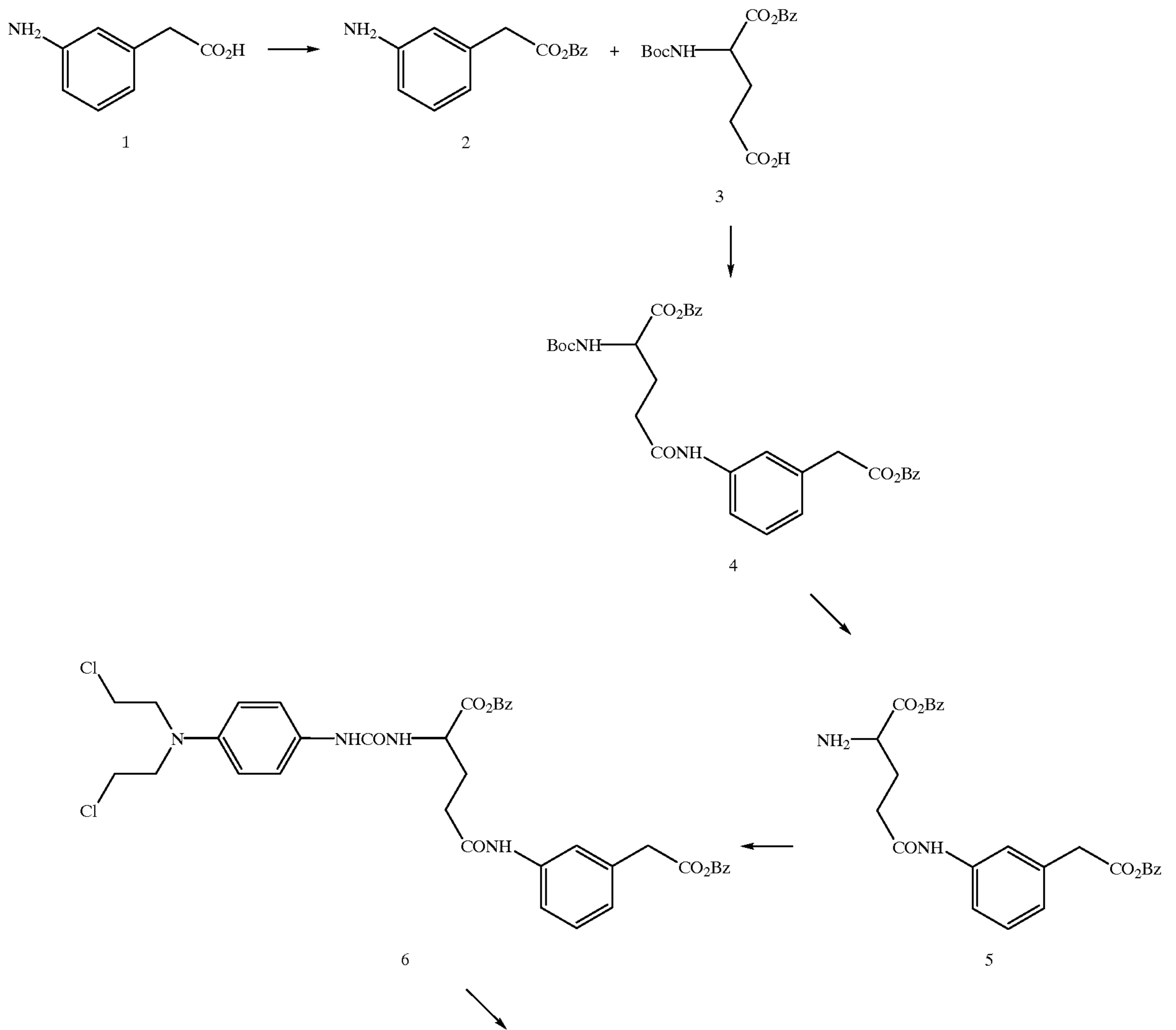
Scheme 11
