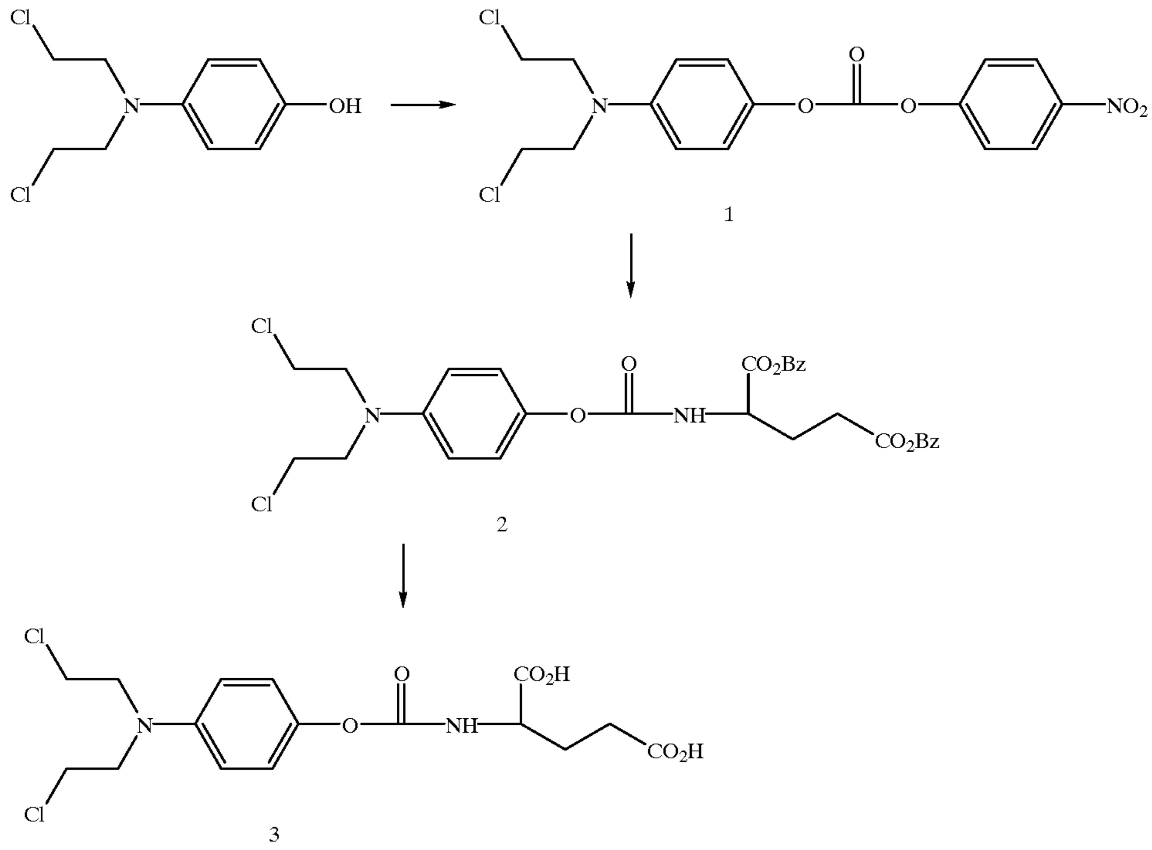
SCHEME 1
