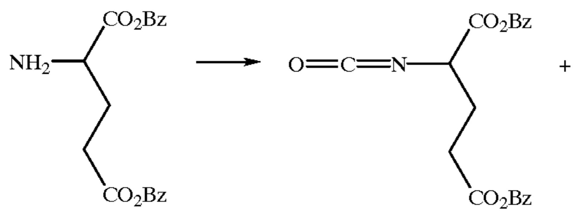
Scheme 10
