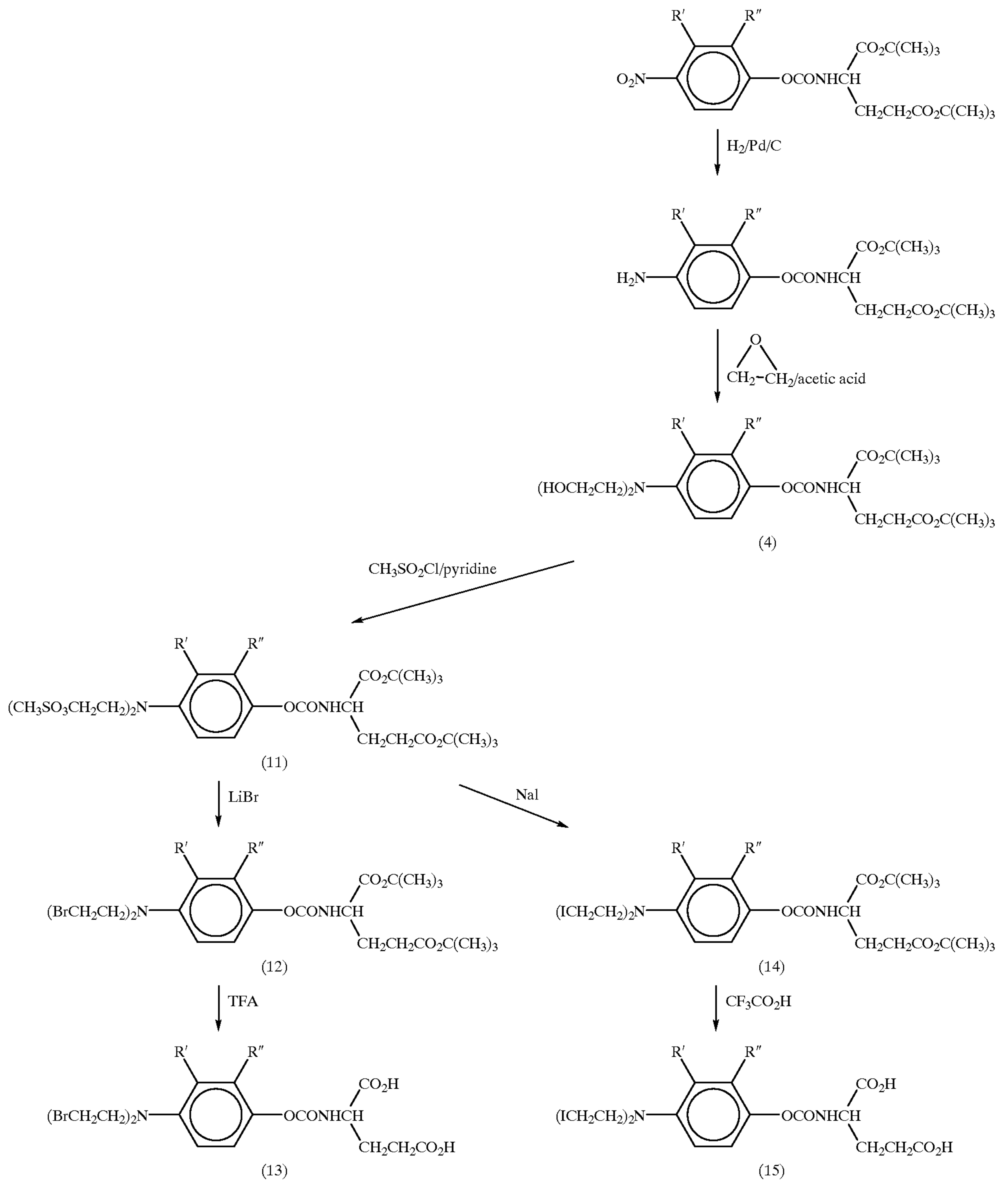
SCHEME 9
