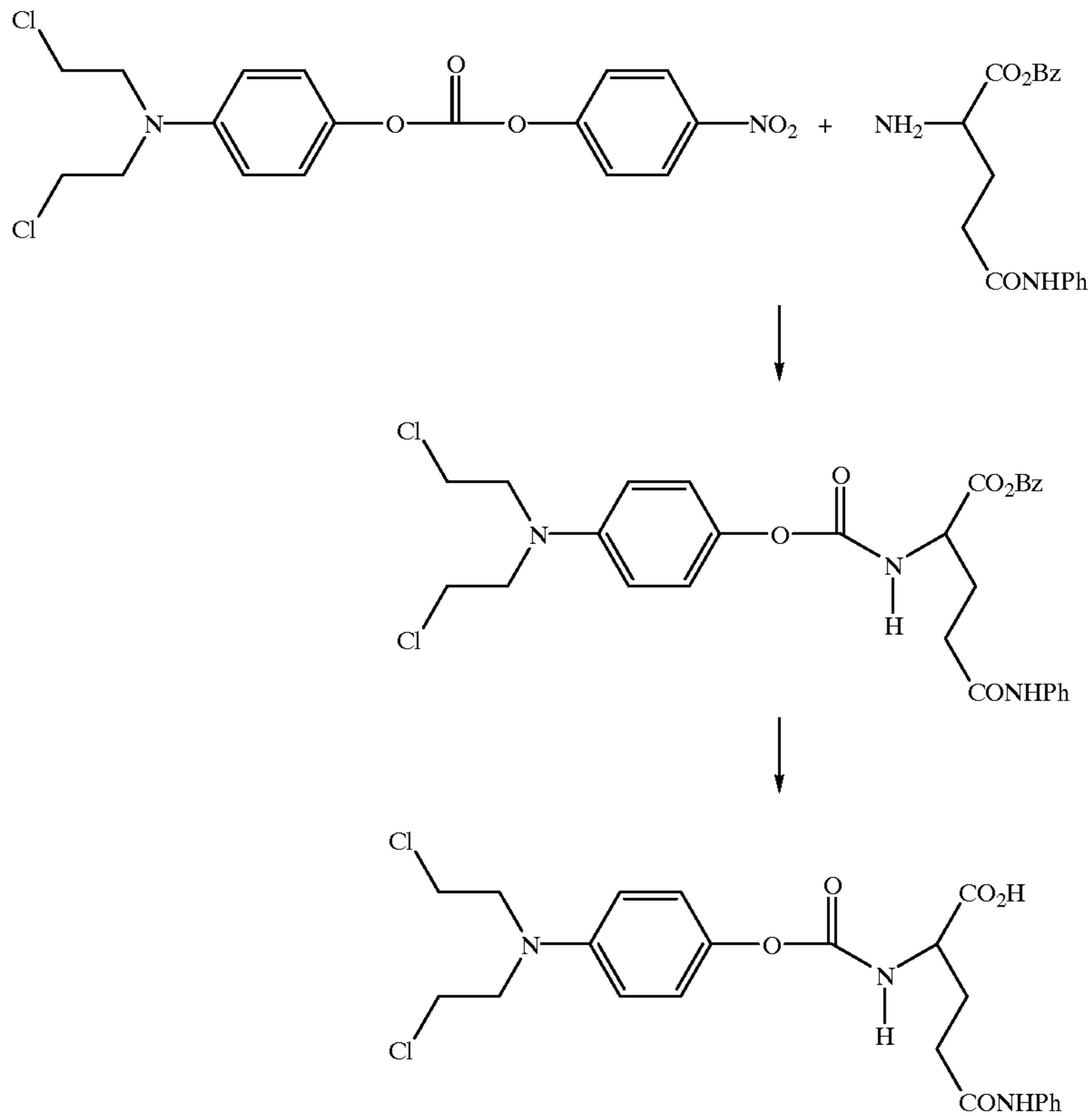
SCHEME 6
