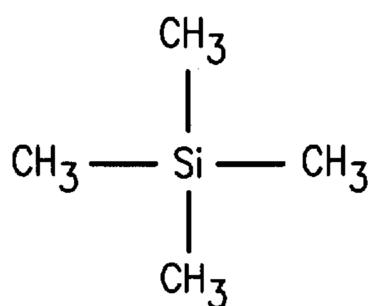
TMS
