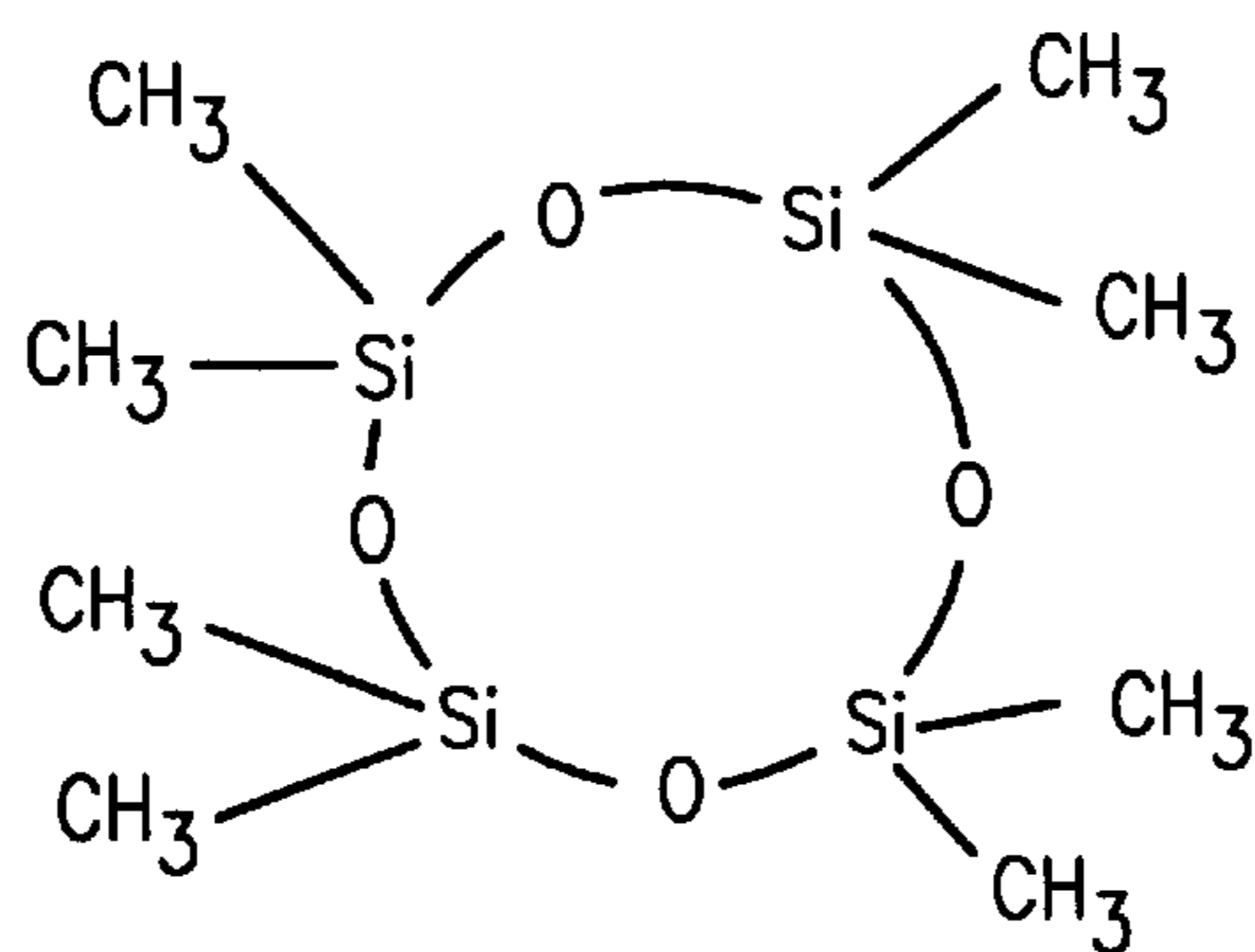
OMCTS
