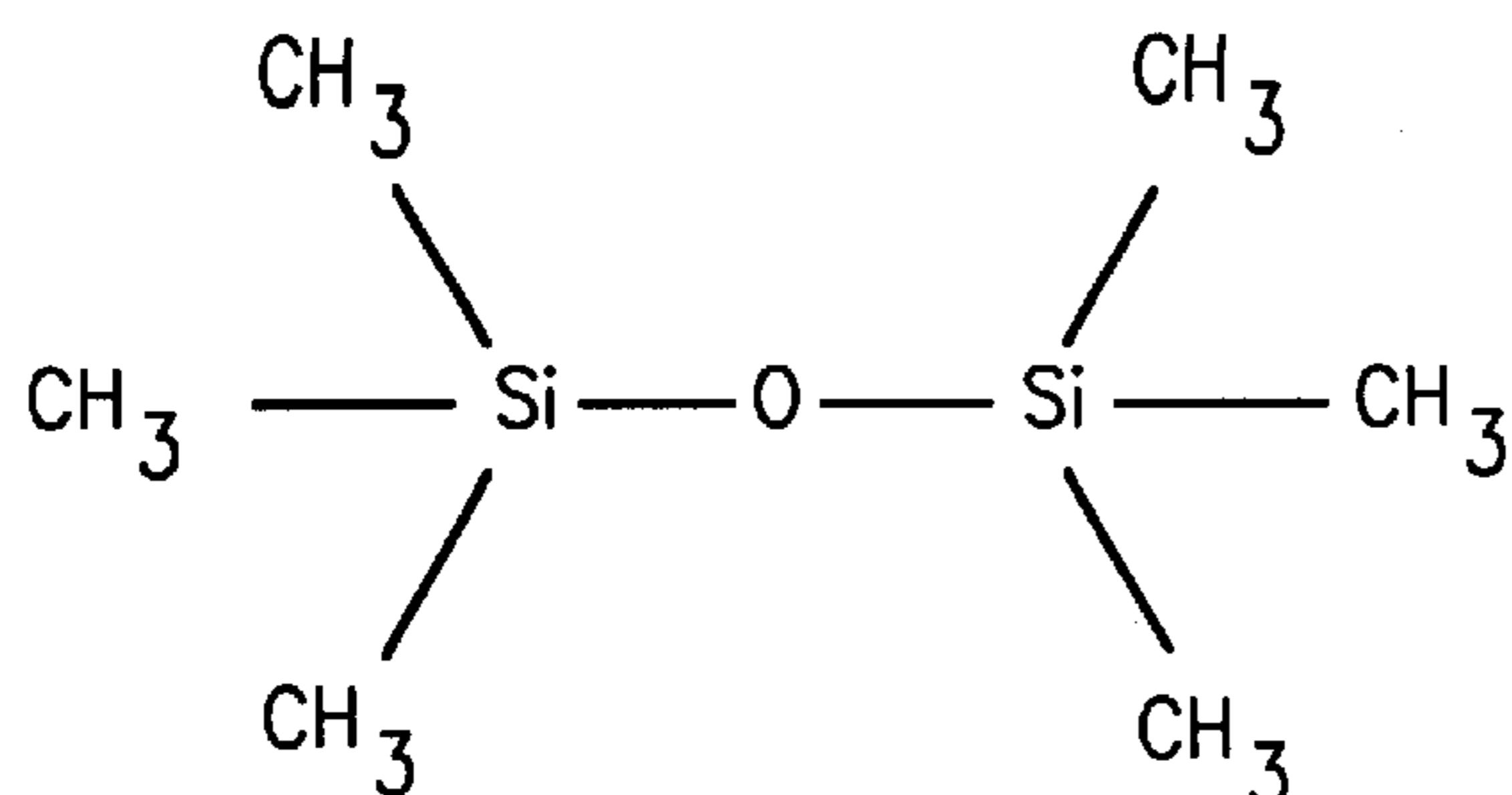
HMDSO
