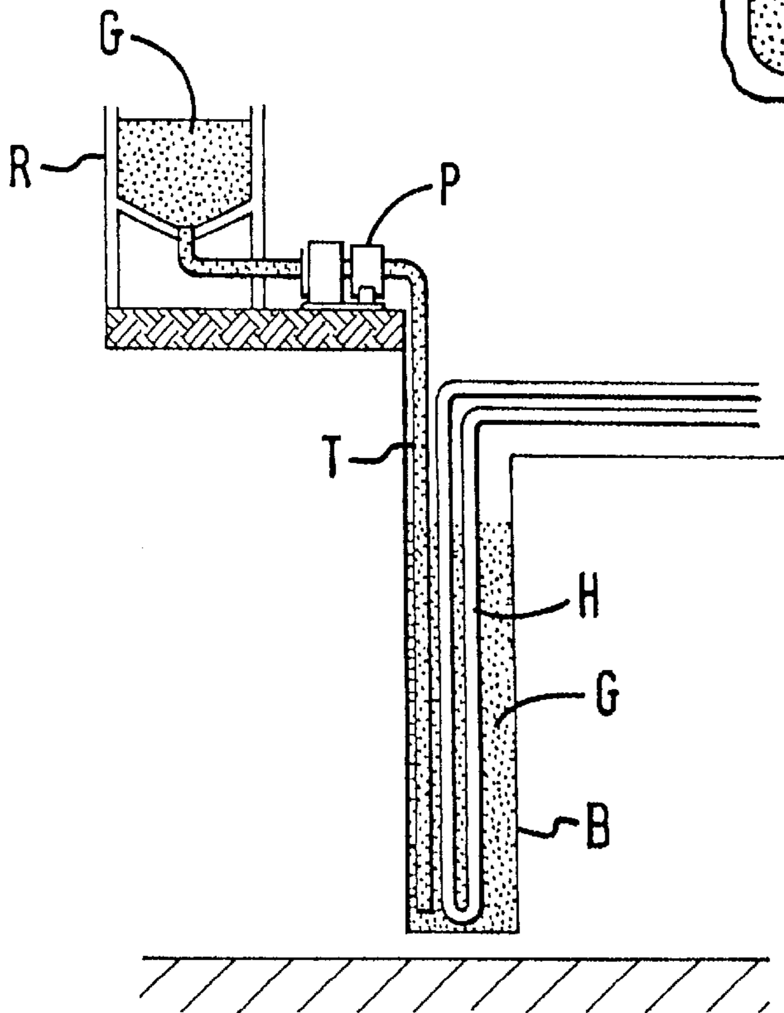
FIG. 2 Prior Art
