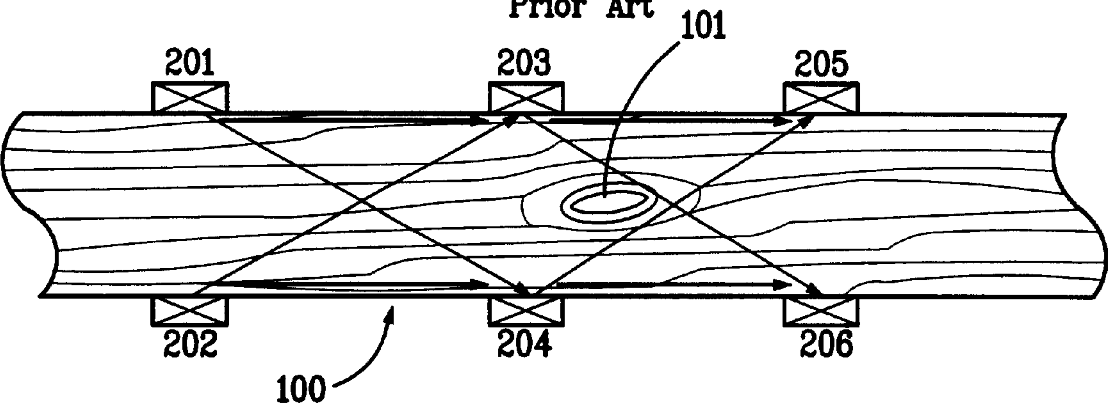
FIG. 2 Prior Art
