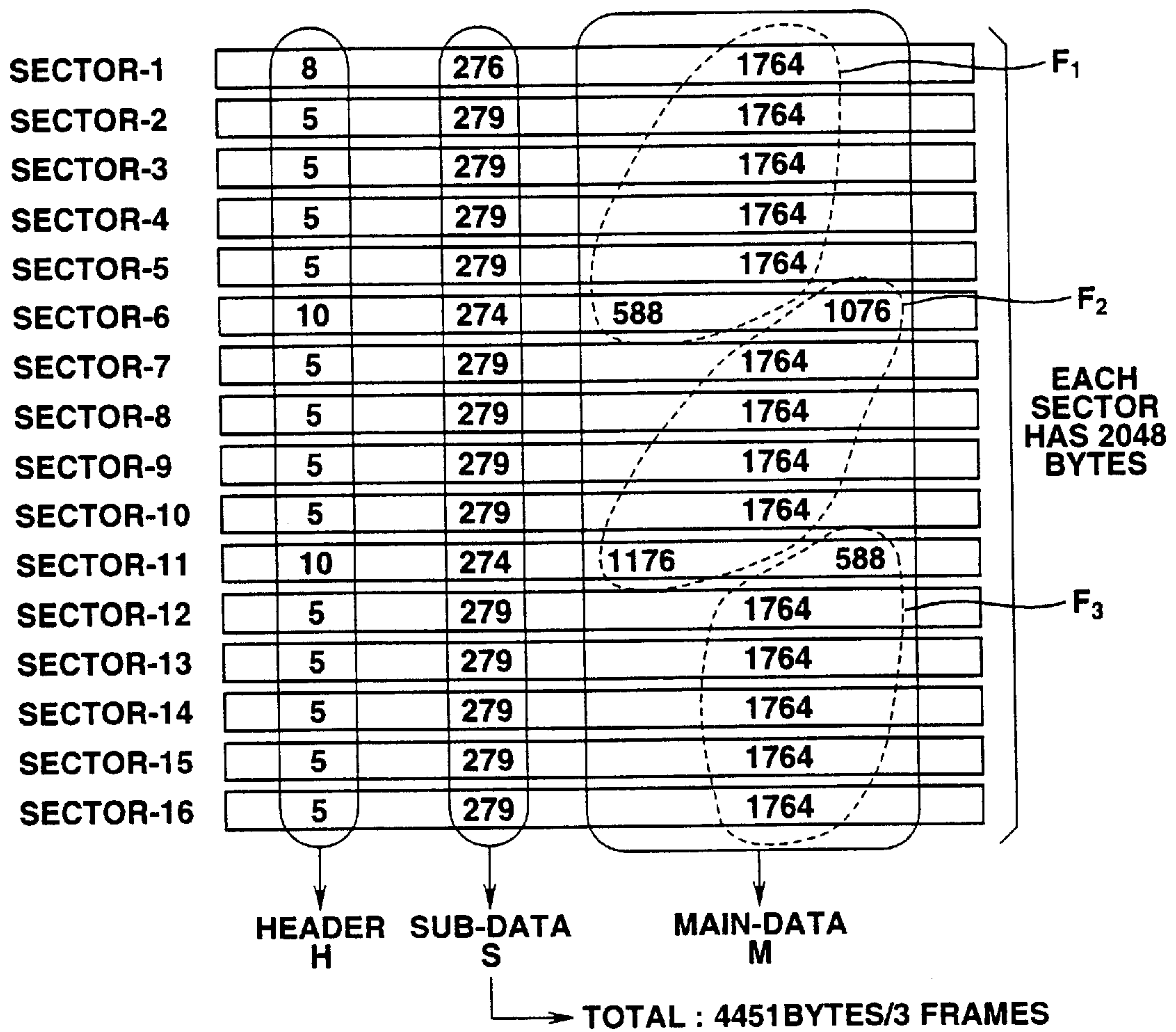
RECORDING 3-FRAME DATA IN 16 SECTORS (EXTENSION MODE)
