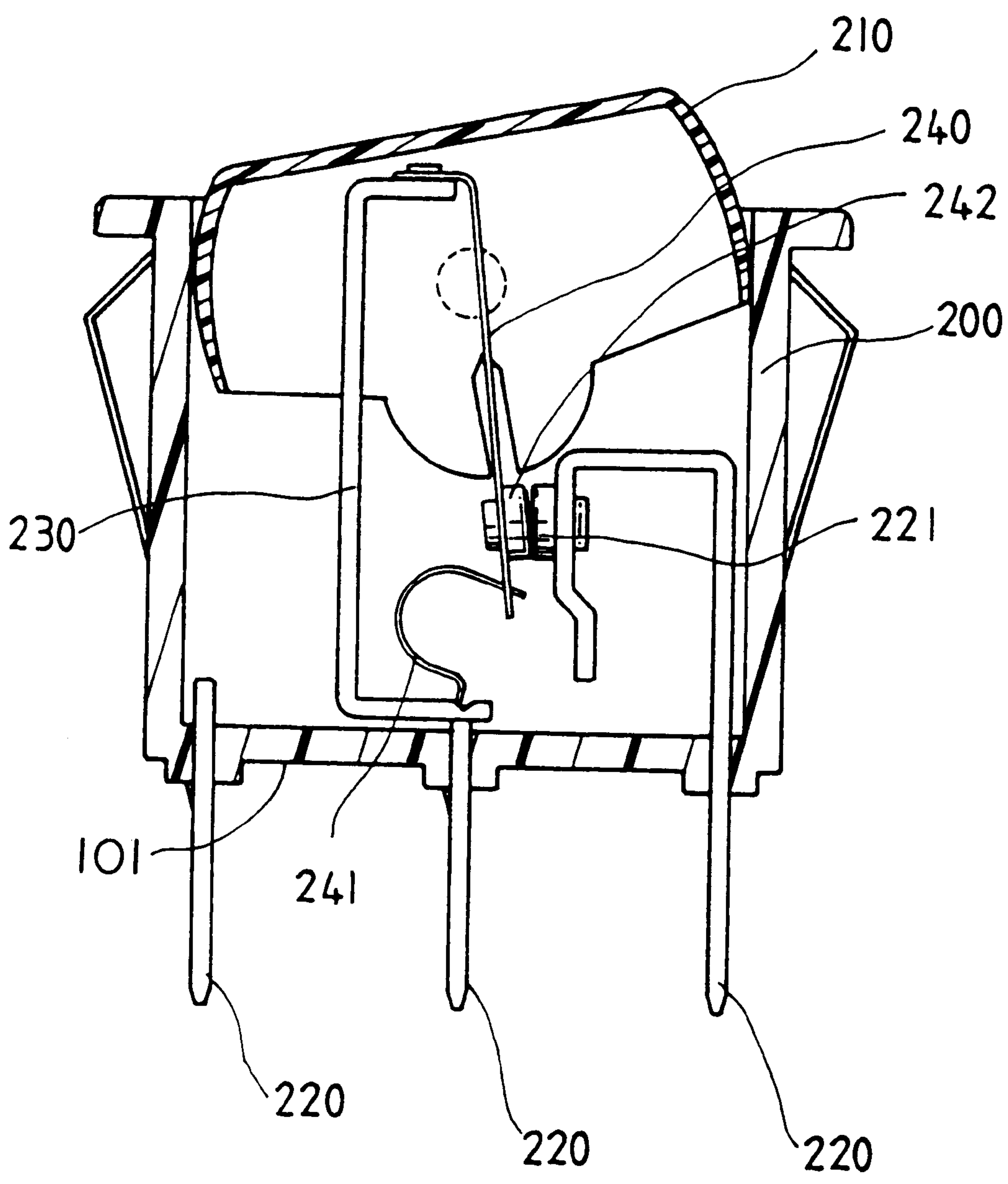
Fig. 2 PRIOR ART
