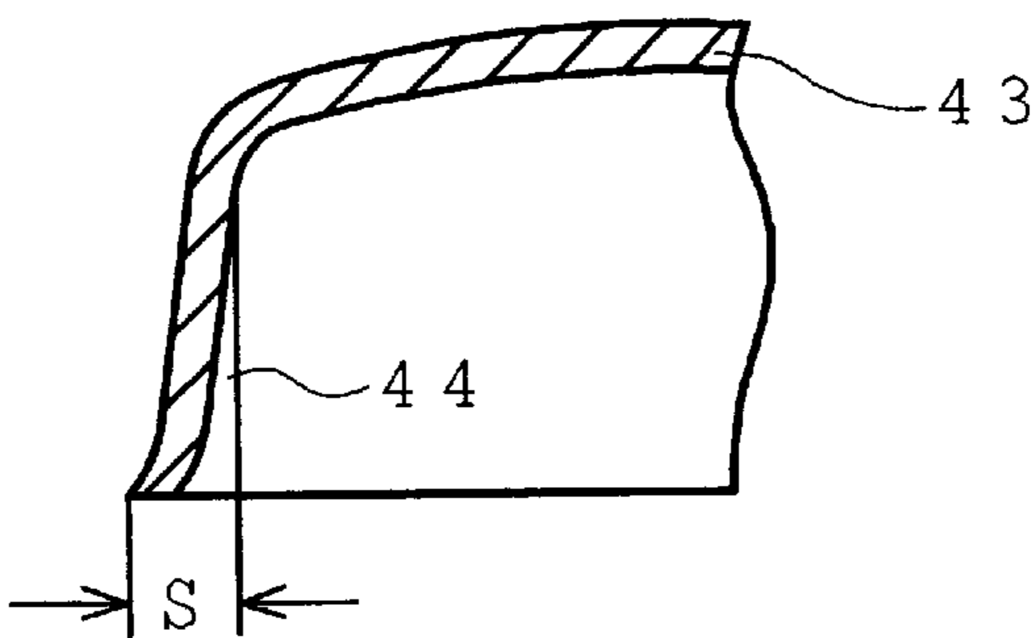
FIG. 4C (PRIOR ART)
