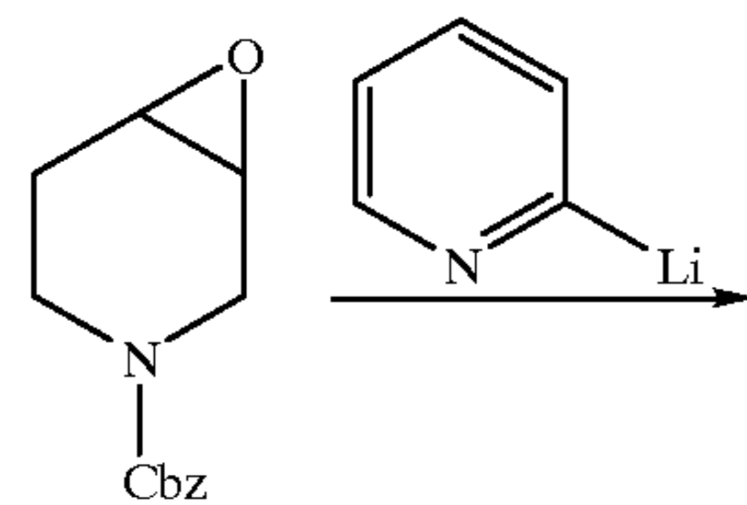
Scheme 4B: Possible Synthetic schemes for precursors
