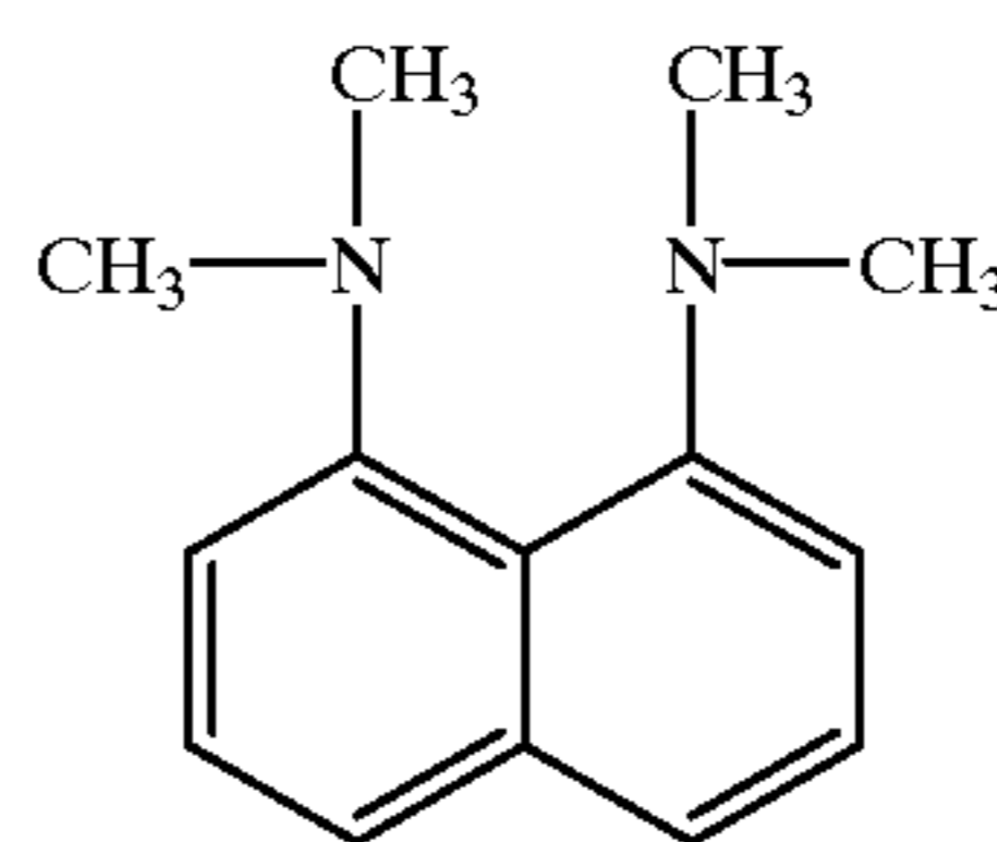
proton sponge
