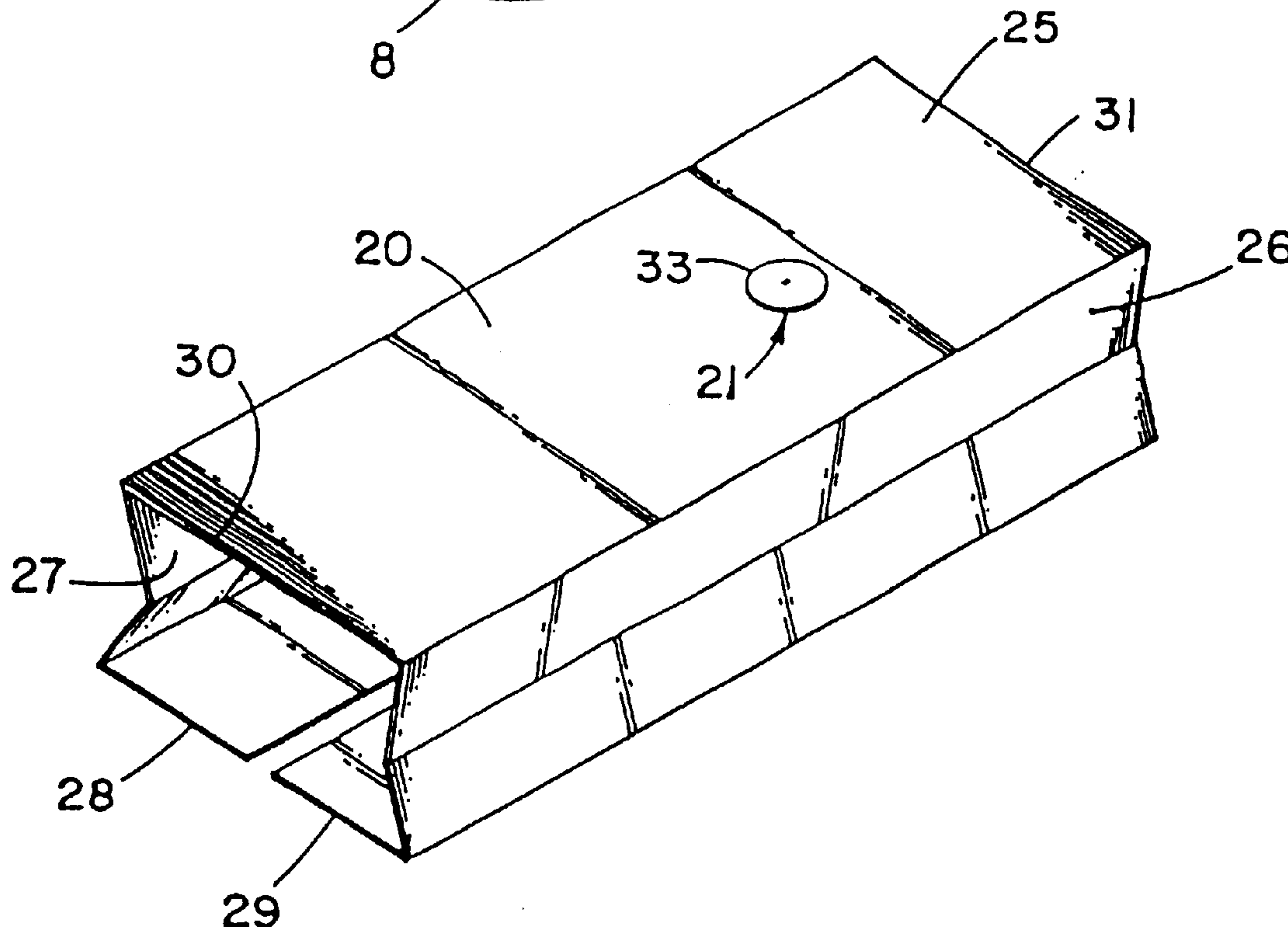
FIG. 2 (PRIOR ART)
