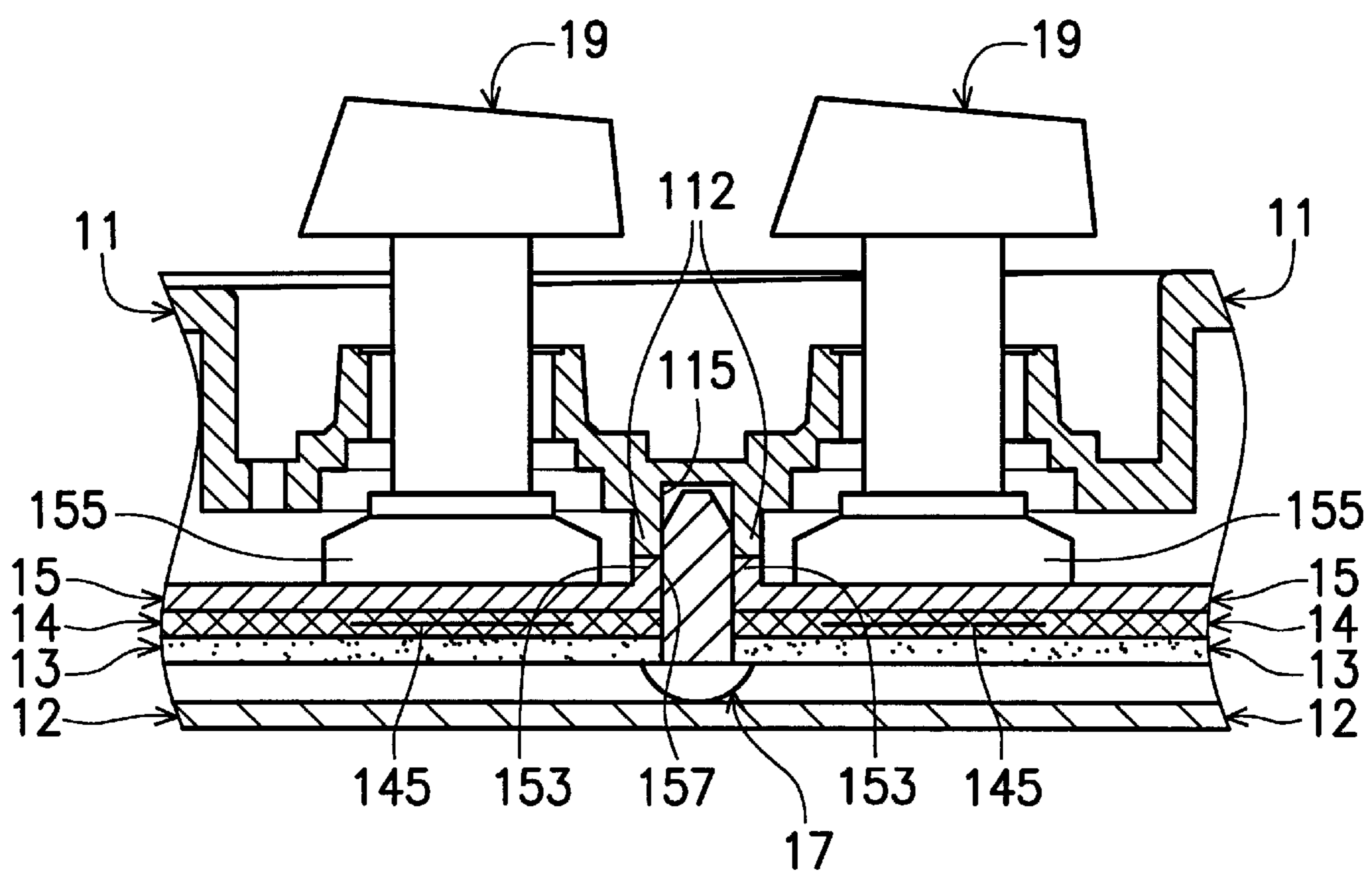
FIG. 4 (PRIOR ART)
