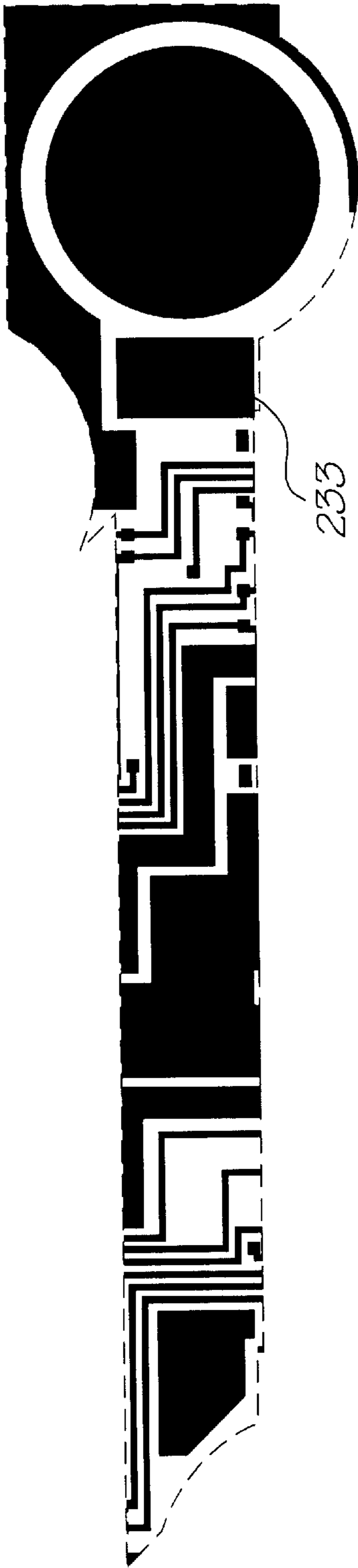
Metal 2 mask
