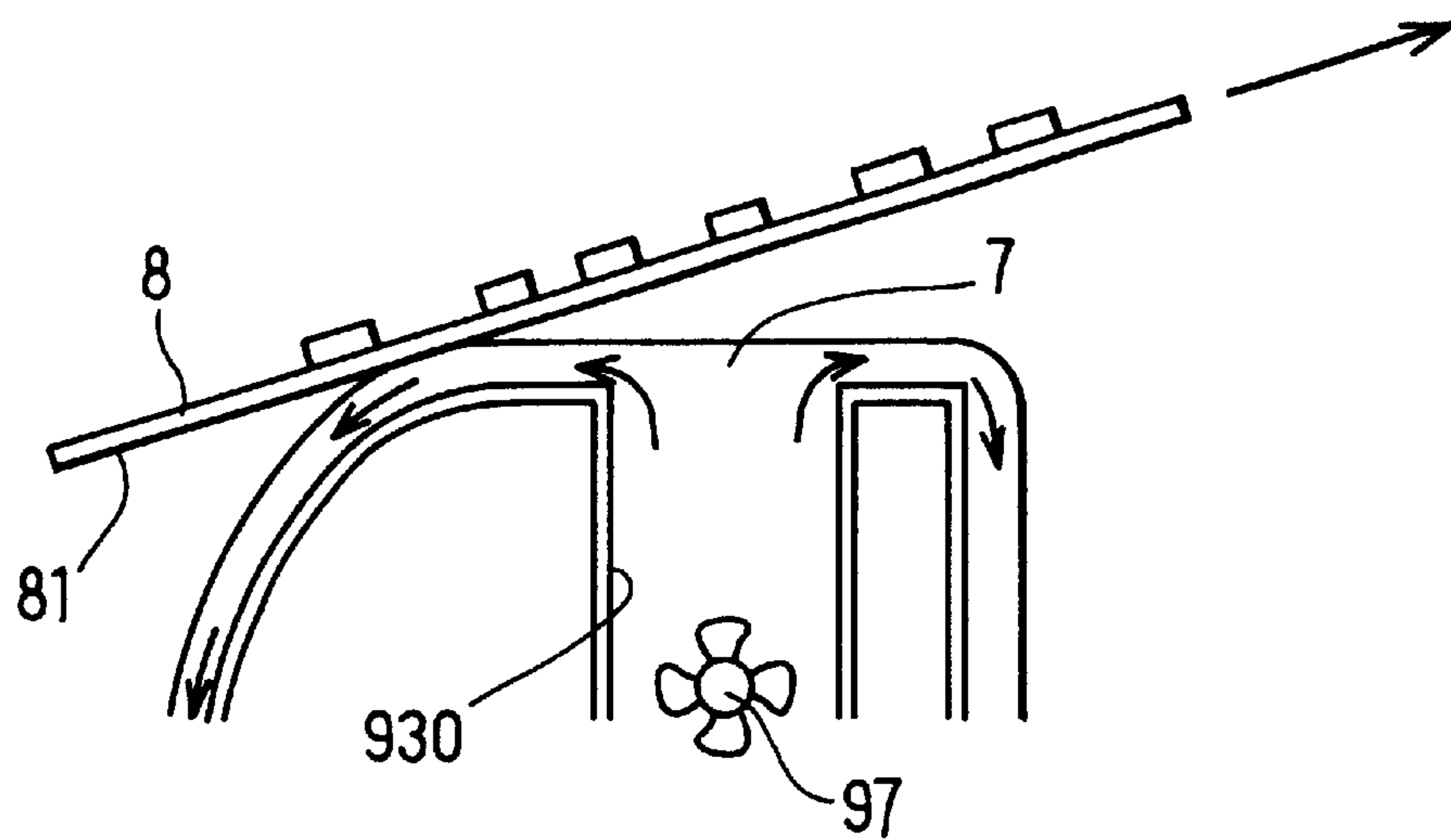
FIG. 12 PRIOR ART
