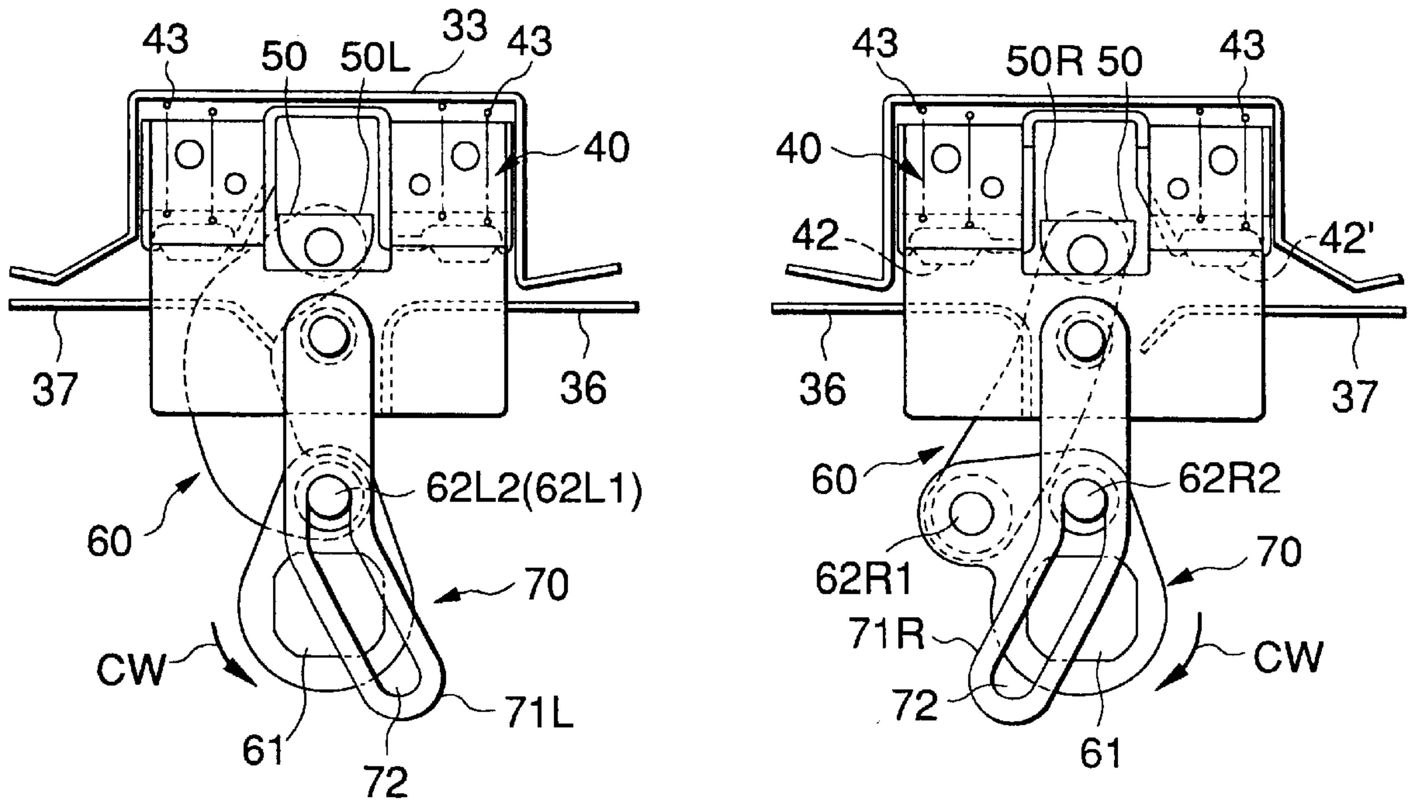
FIG.30(a) (STANDBY STATE) FIG.30(b)
