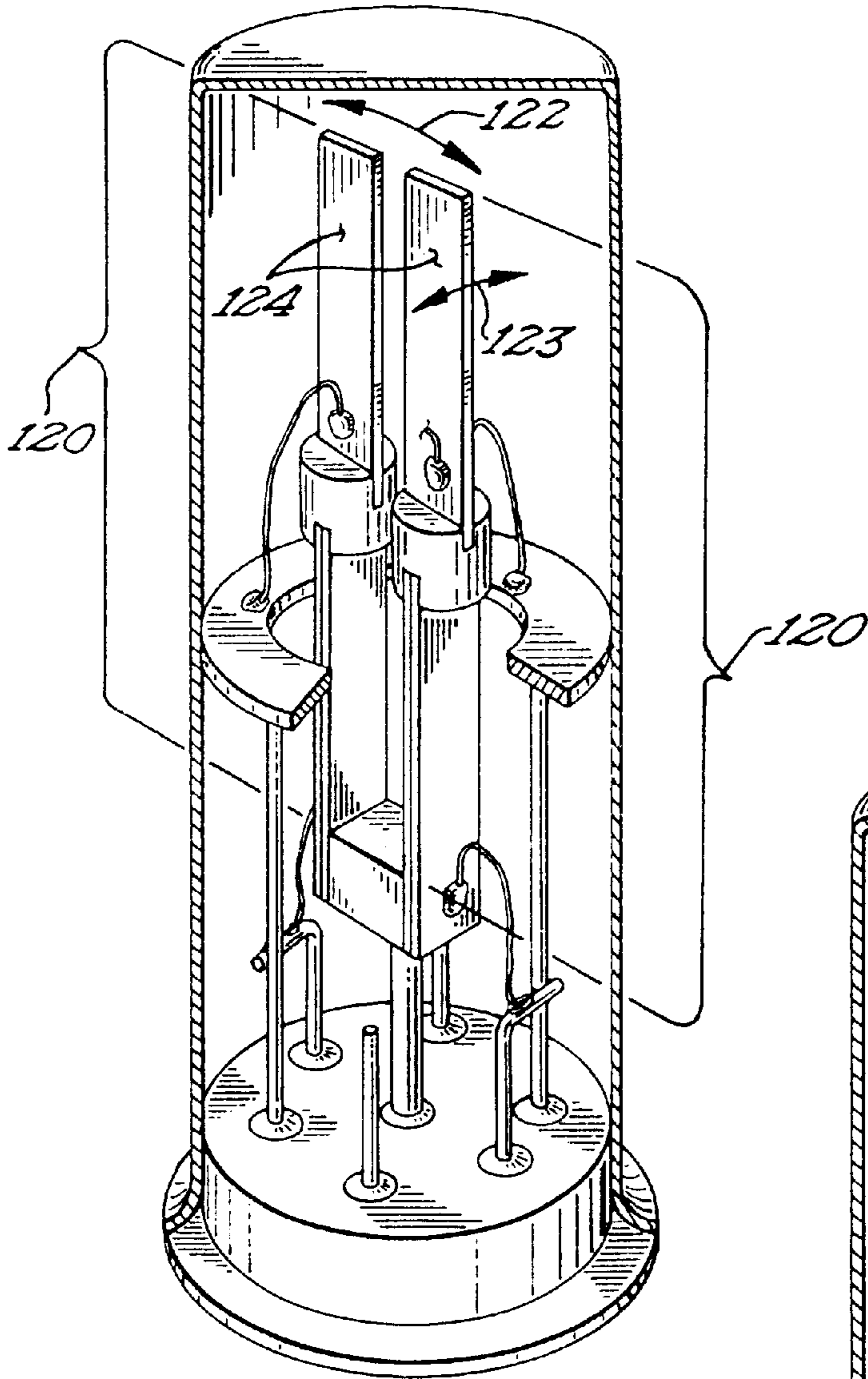
Fig 18 PRIOR ART
