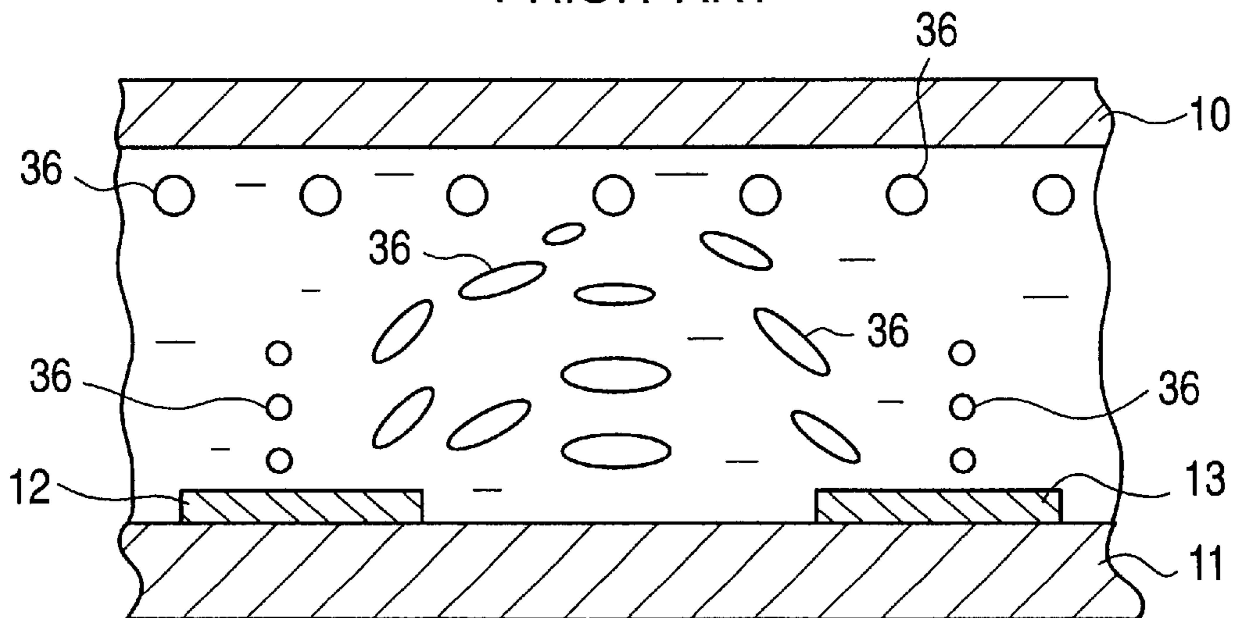
FIG. 10 PRIOR ART
