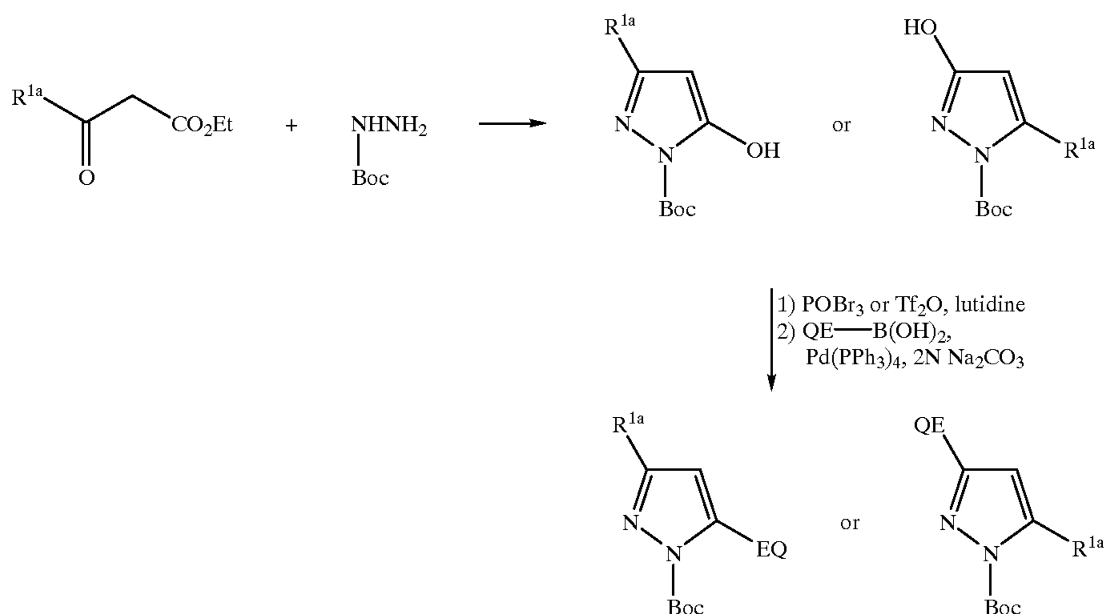
Scheme 26
