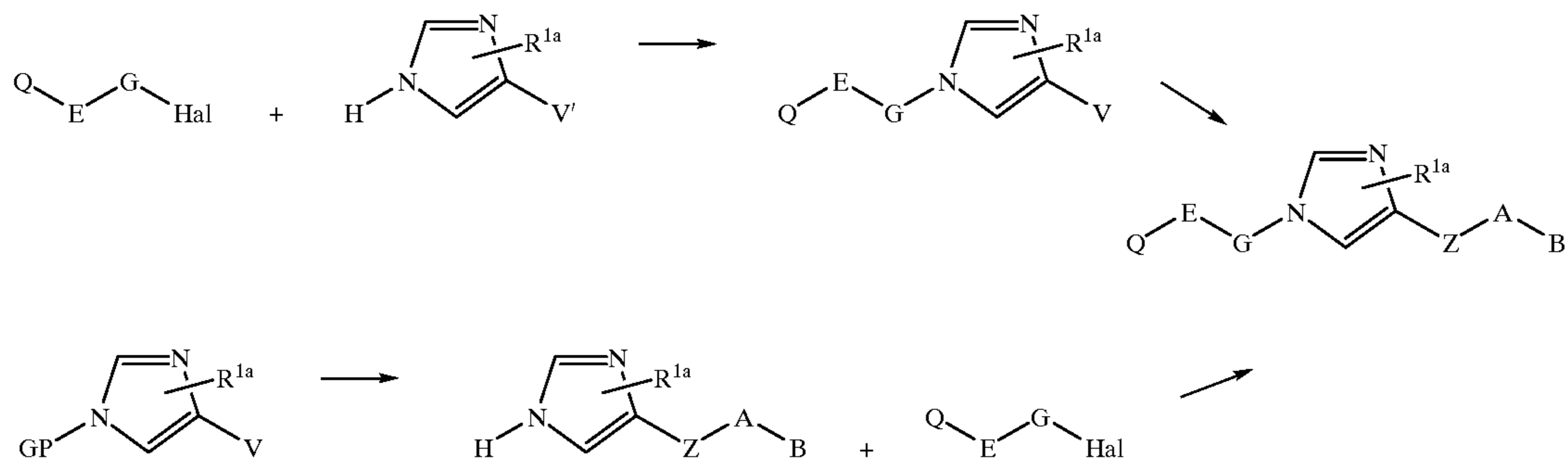
Scheme 10
