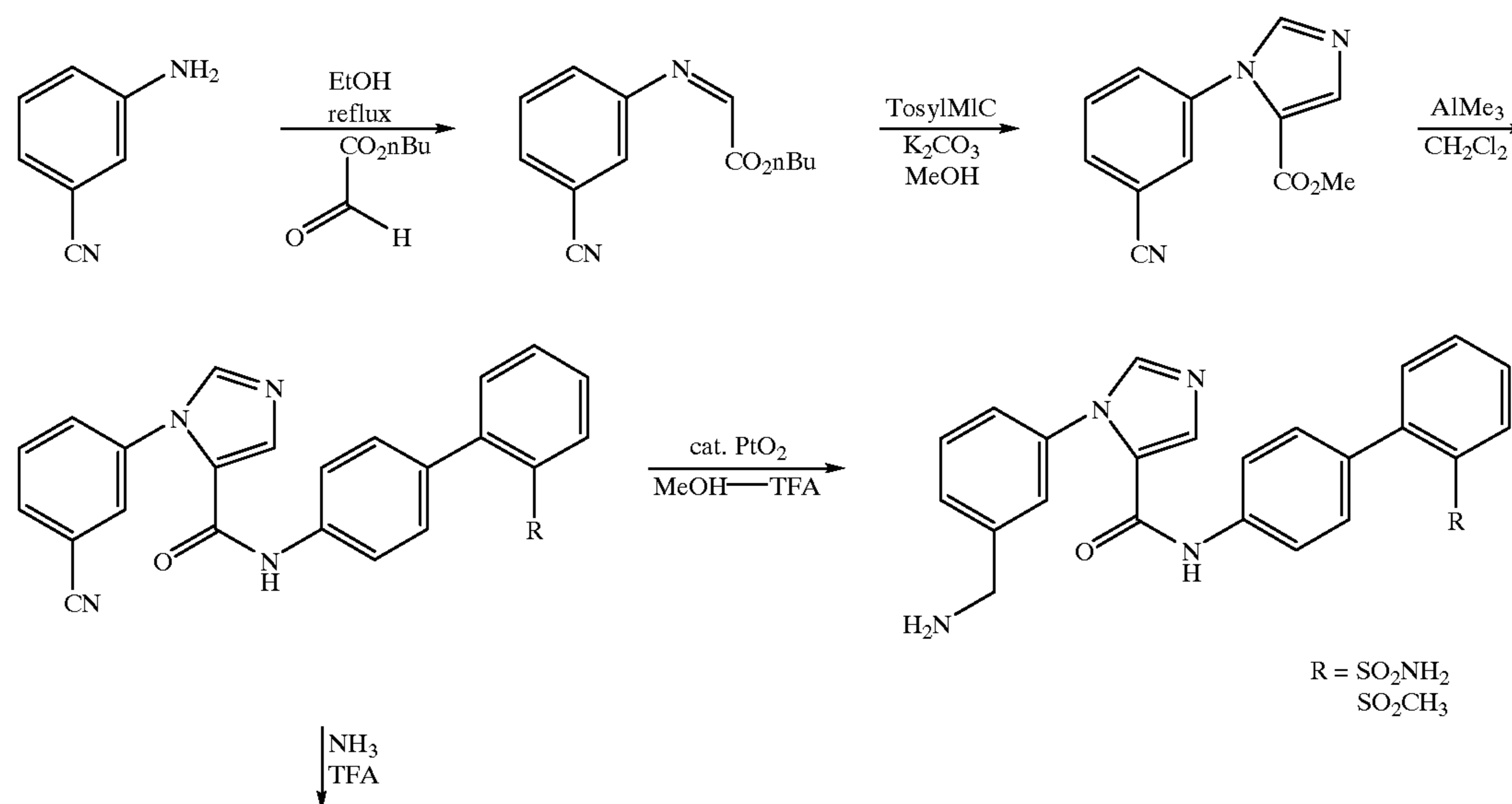
Scheme 32
