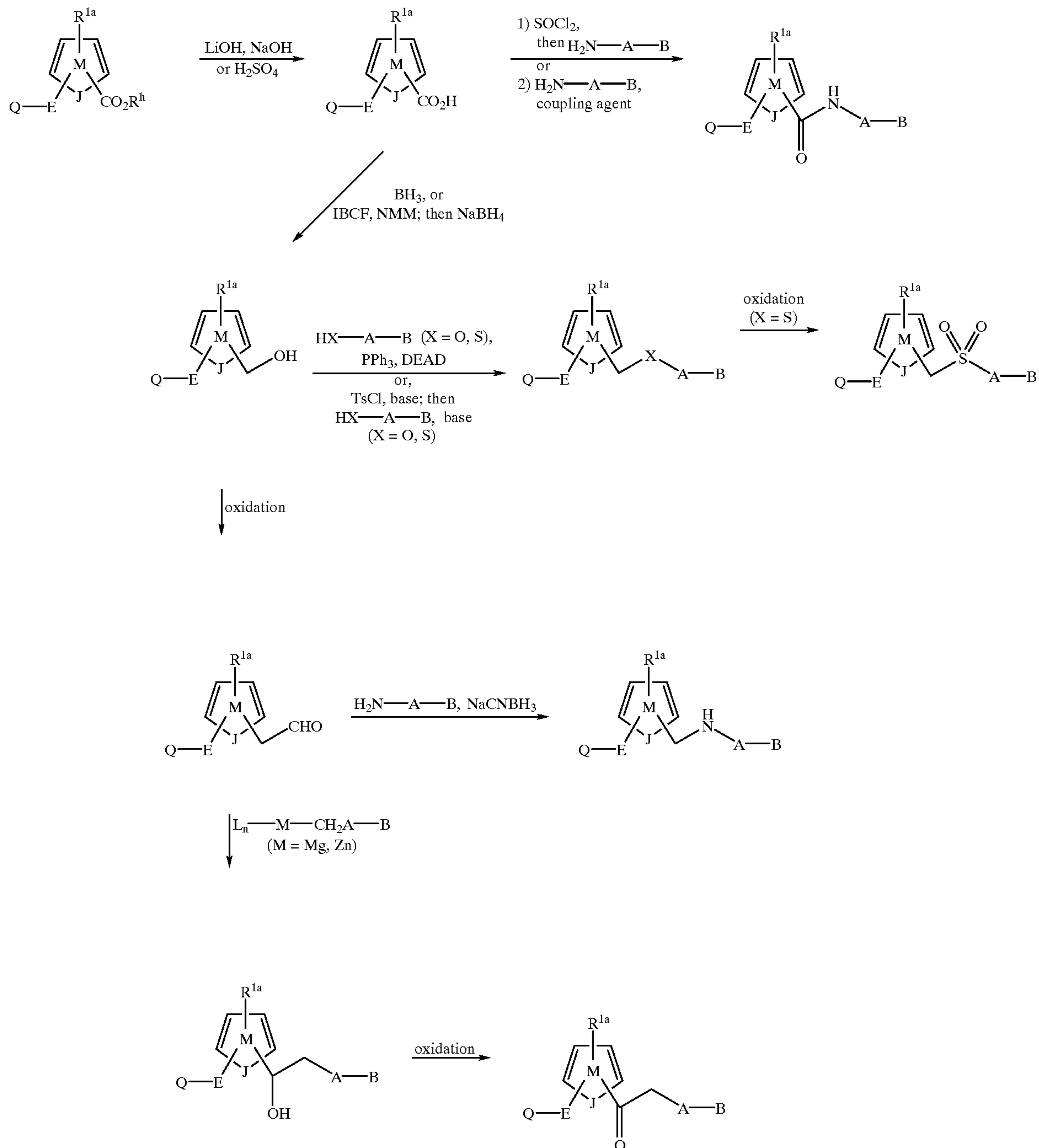
Scheme 7
