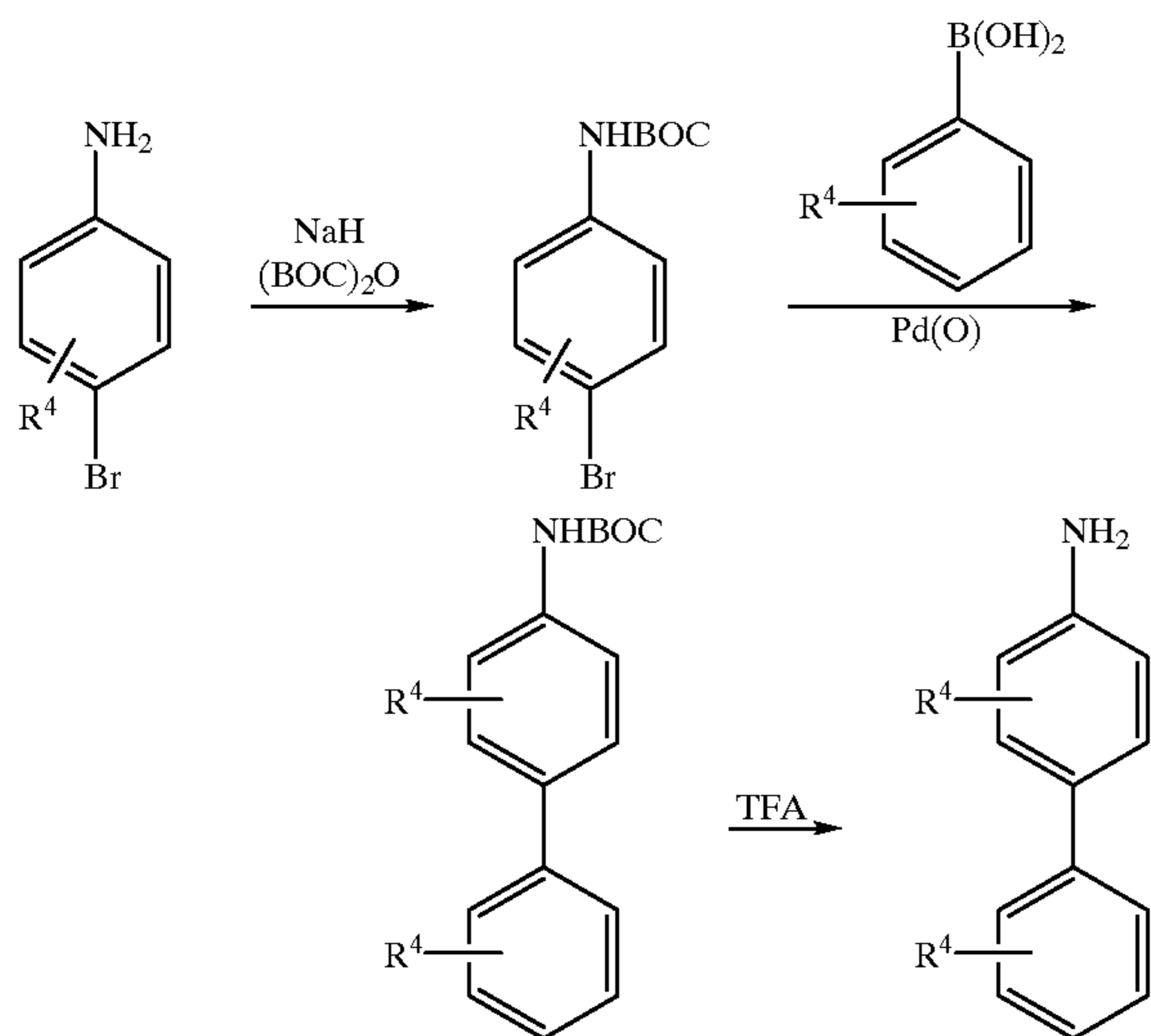
Scheme 33
