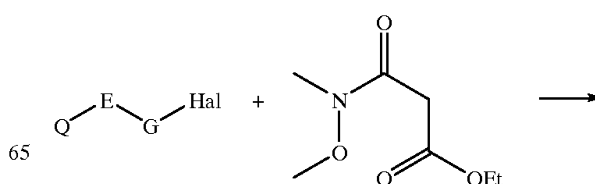
Scheme 16
