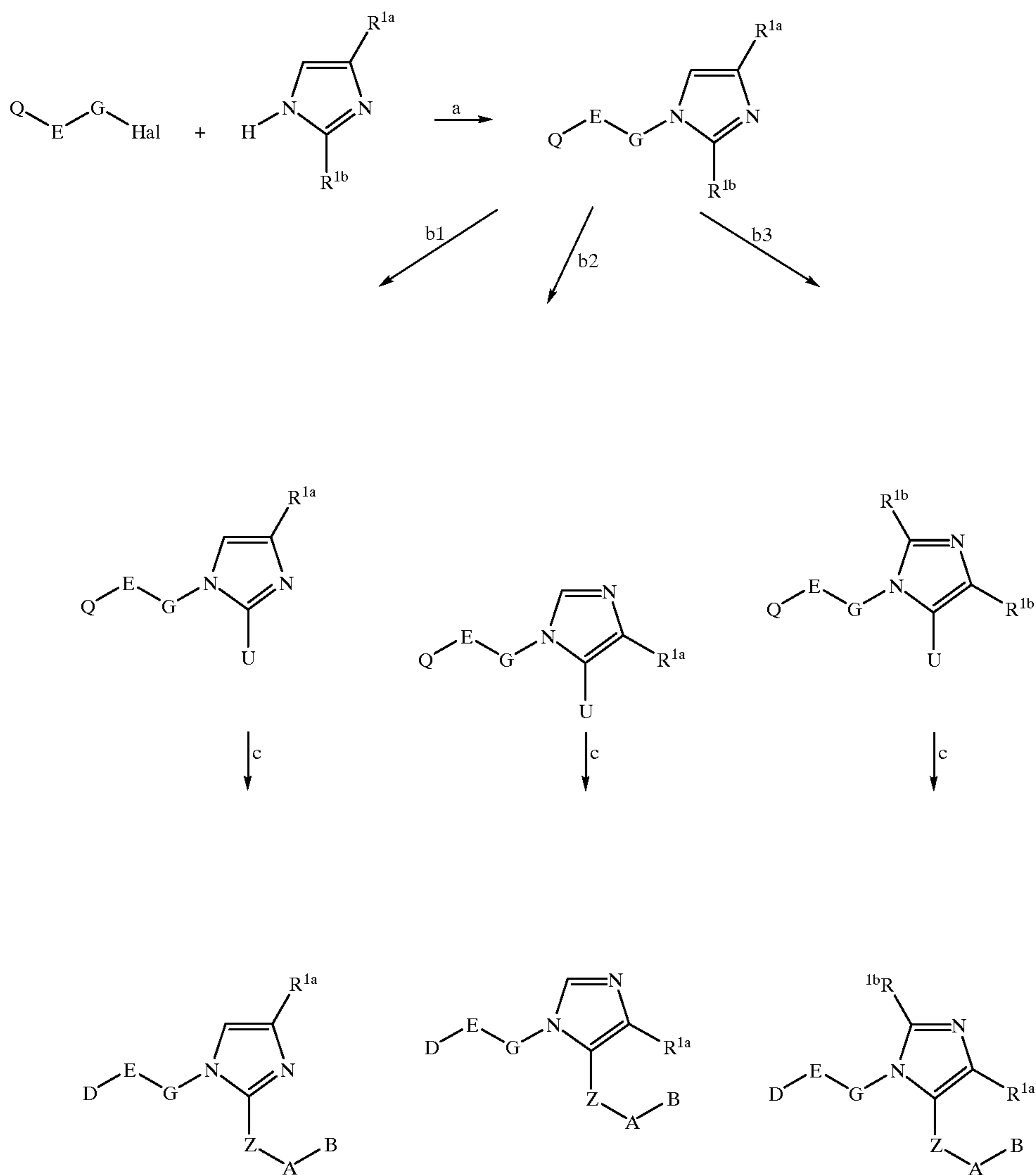
Scheme 12
