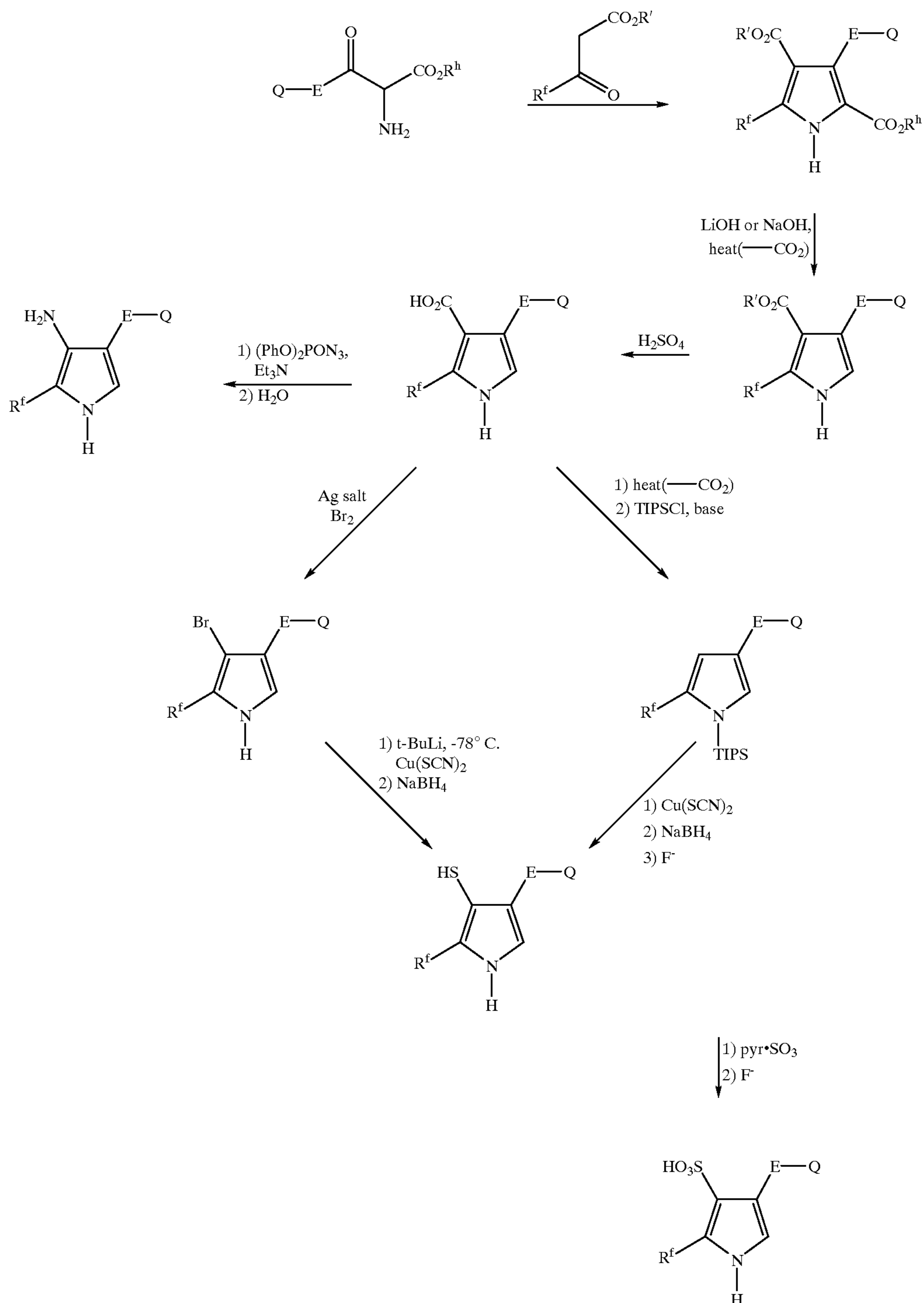
Scheme 4
