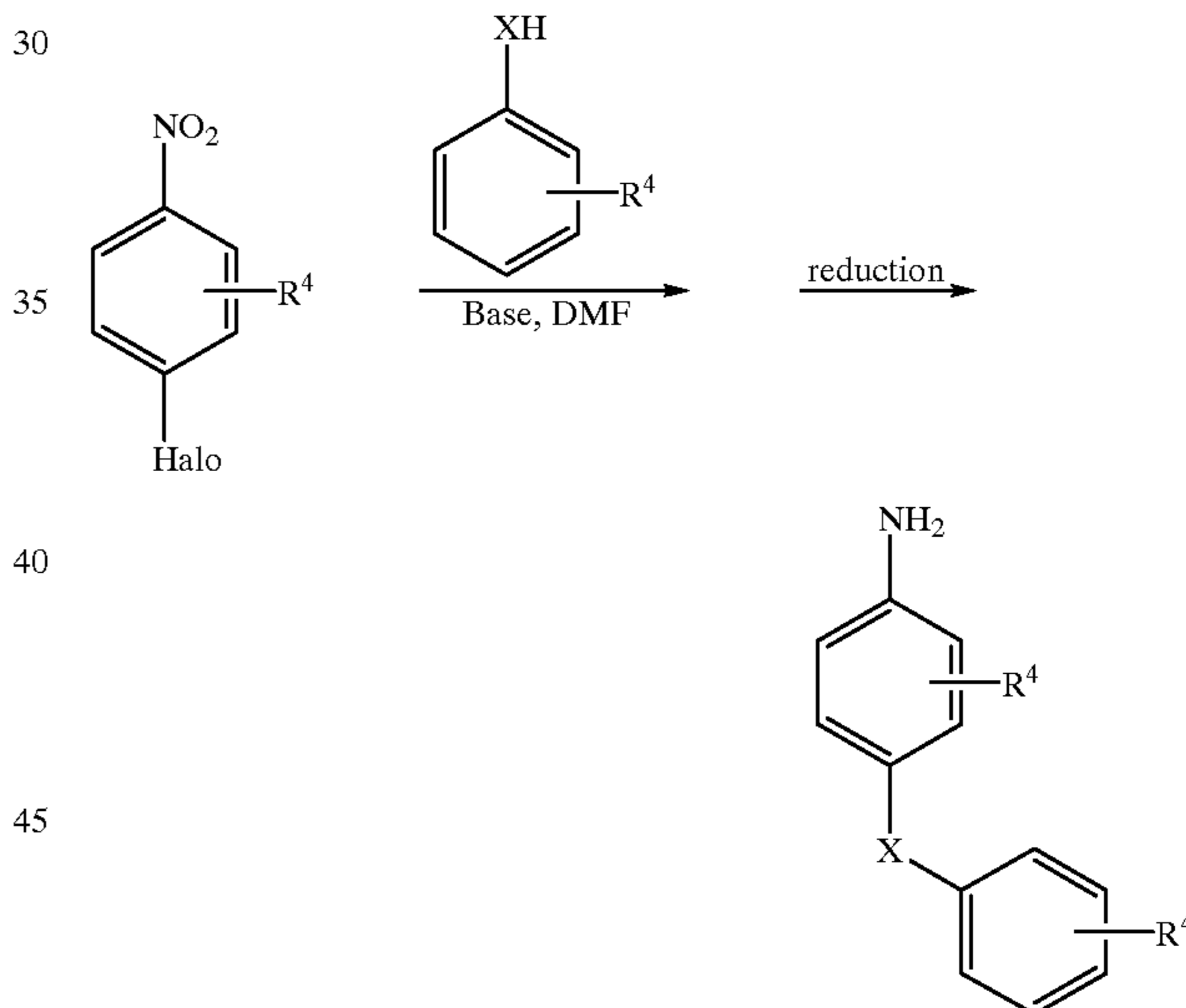
Scheme 35
