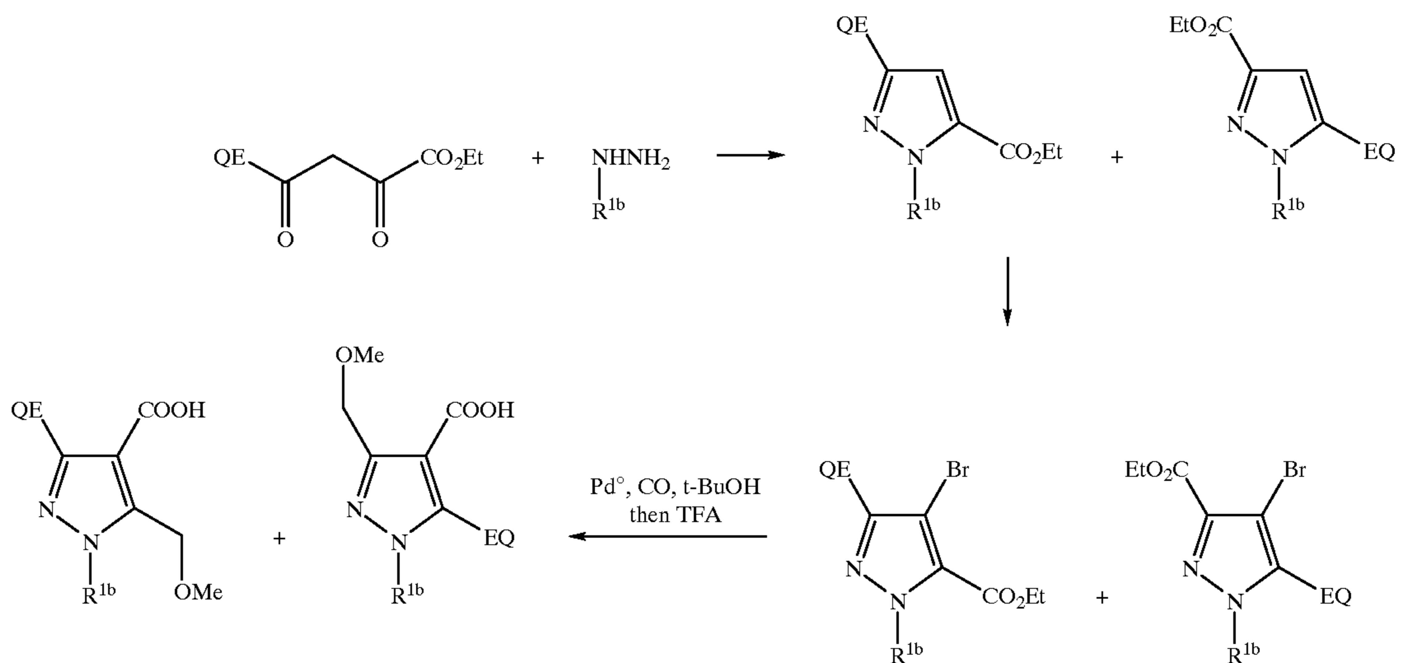
Scheme 24
