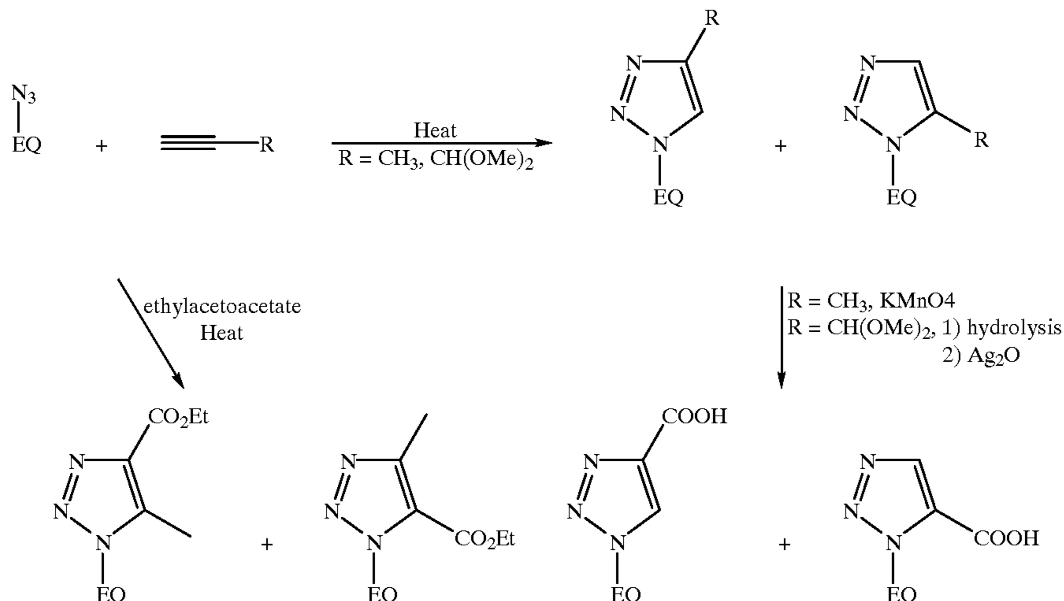
Scheme 27
