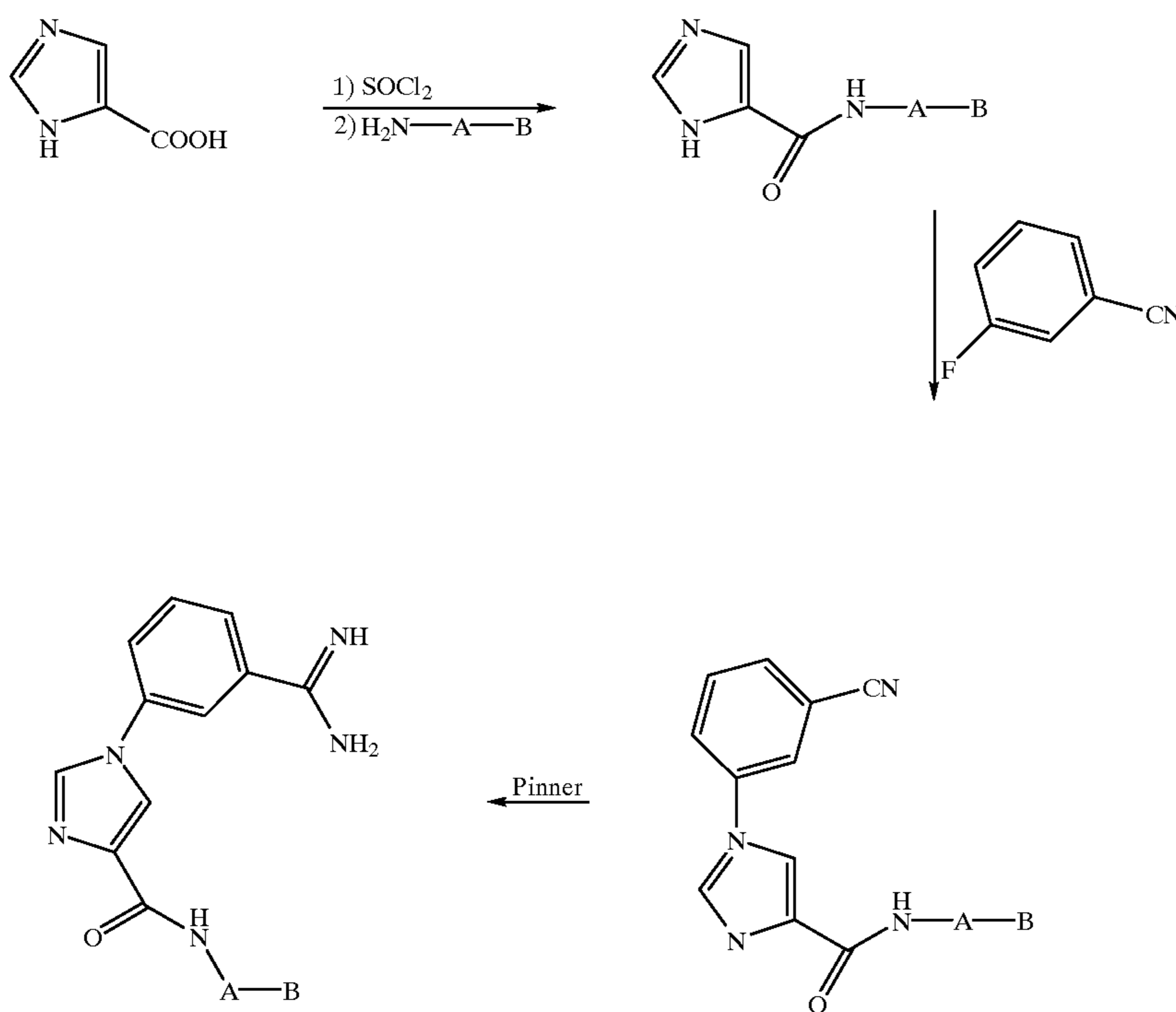
Scheme 11
