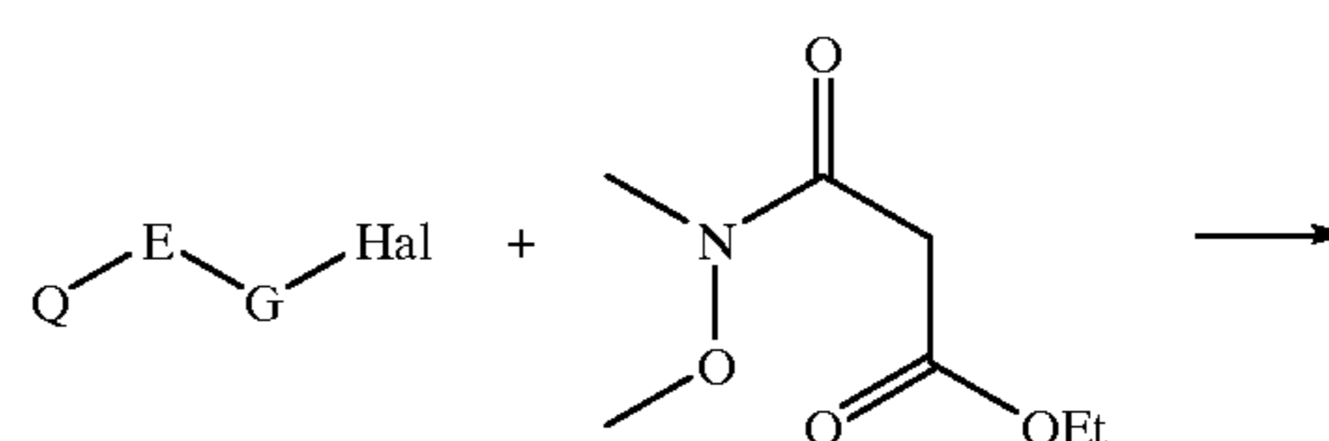
Scheme 16
