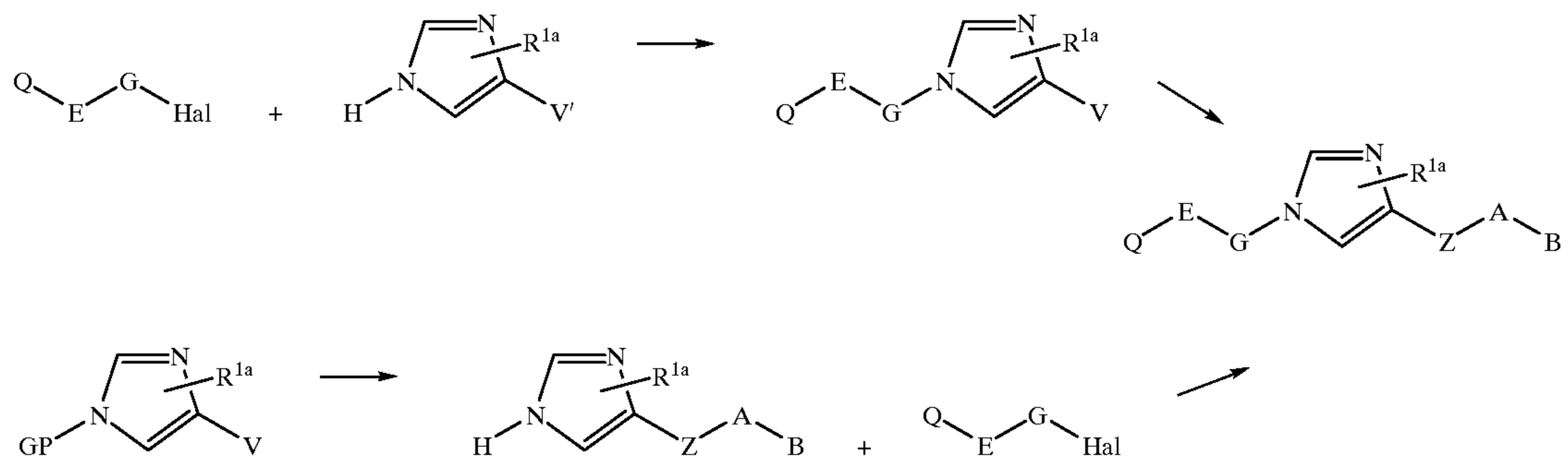
Scheme 10
