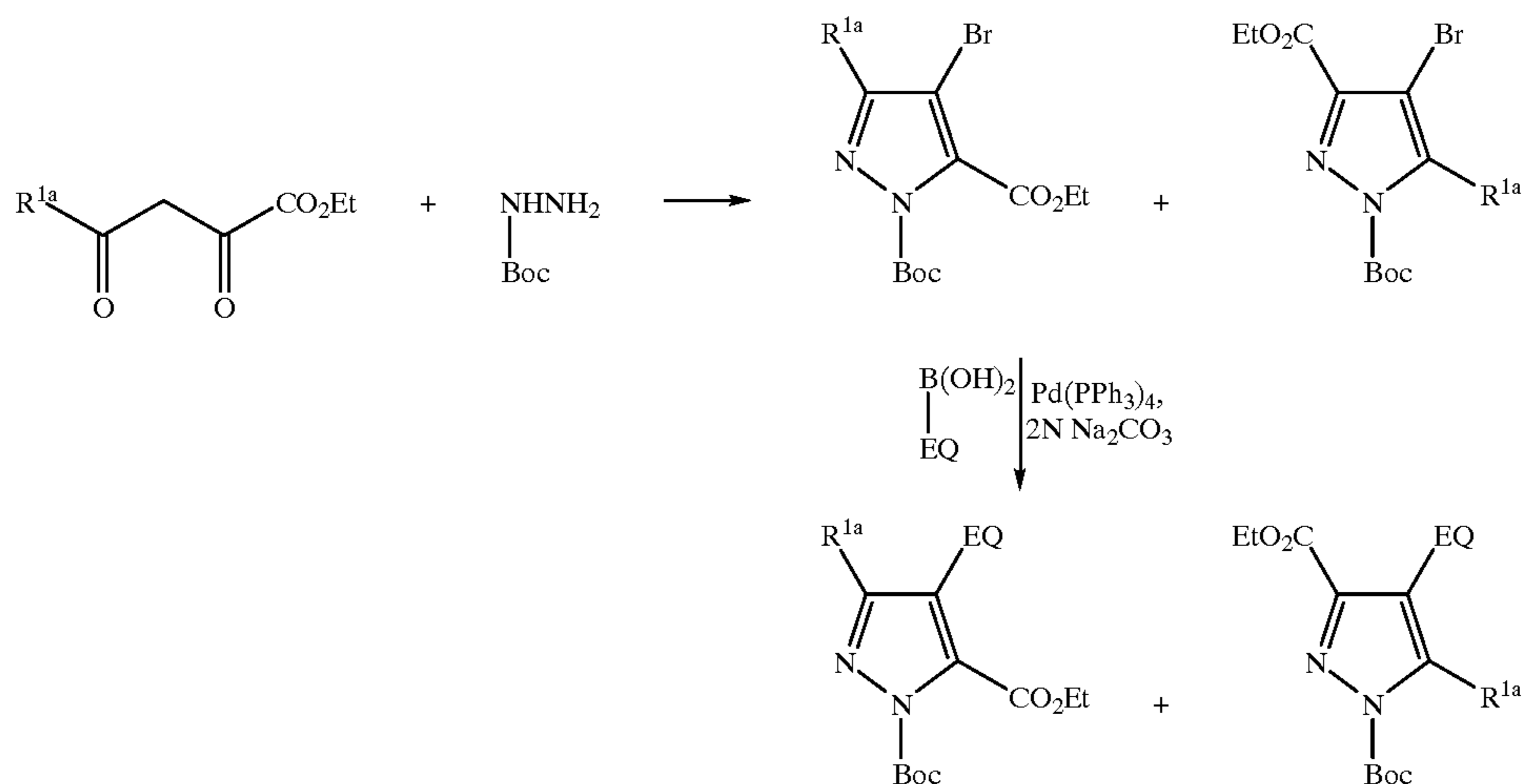
Scheme 25
