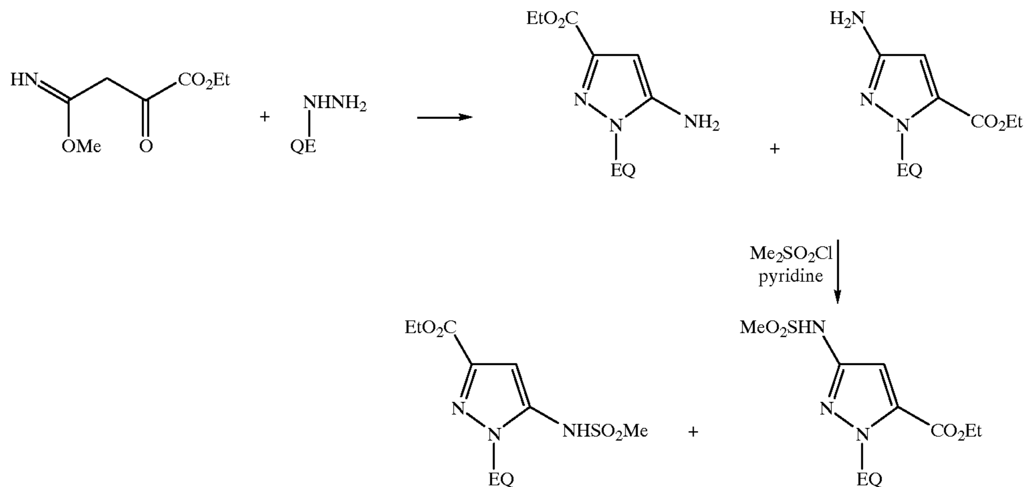
Scheme 23
