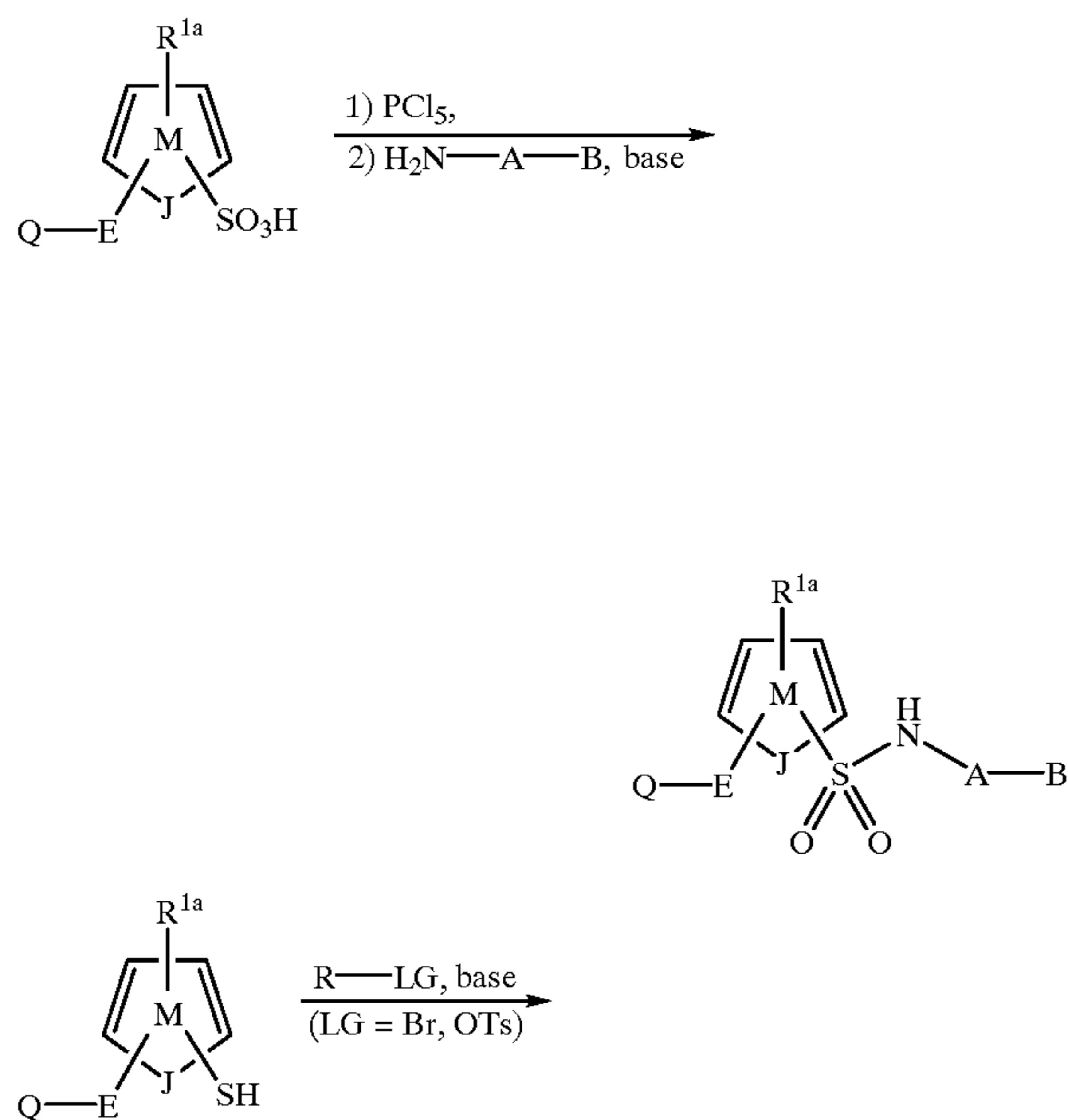
Scheme 9
