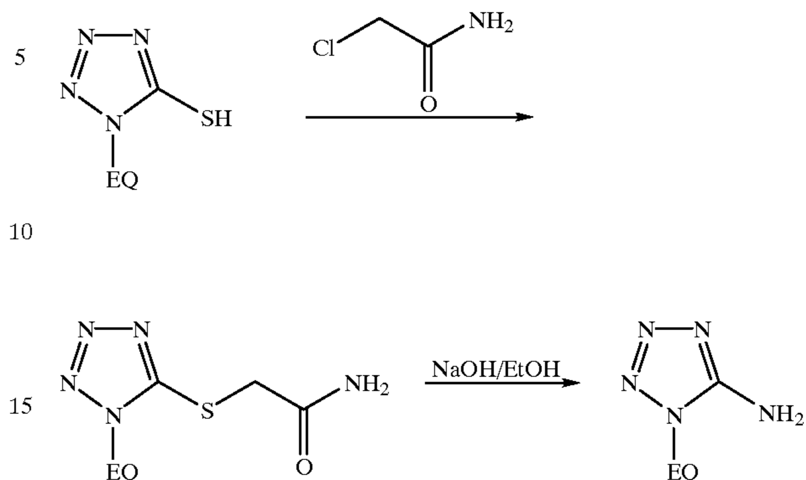
Scheme 21
