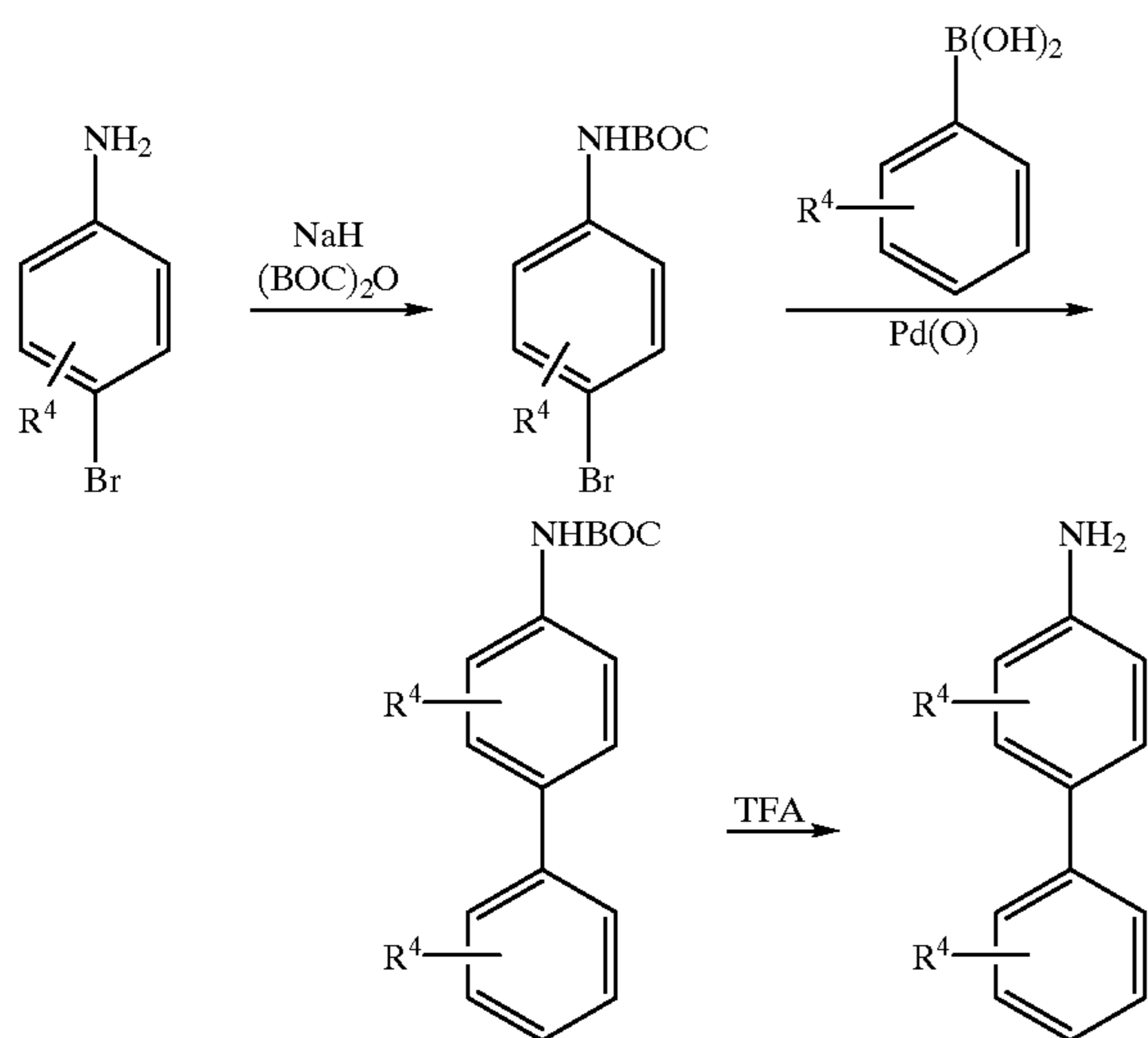
Scheme 33
