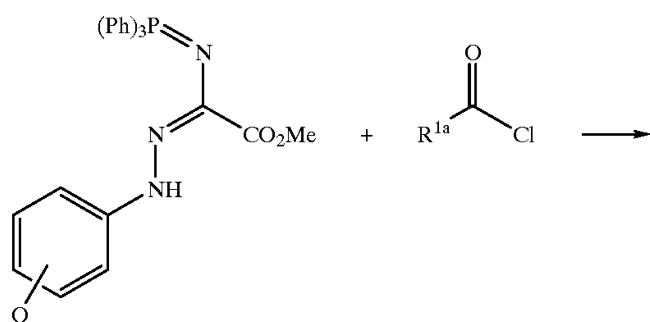
Scheme 29
