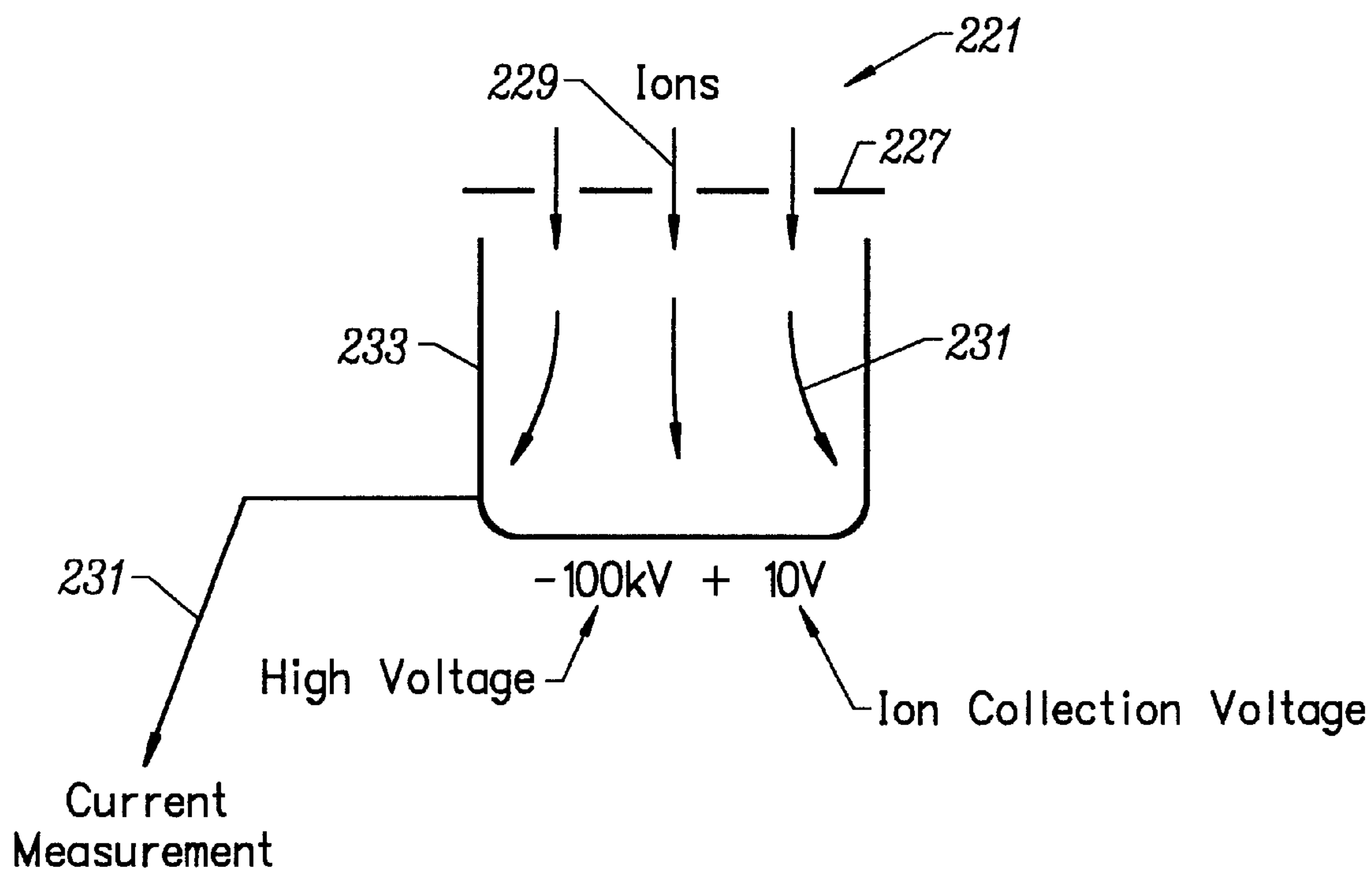
FIG. 2D
