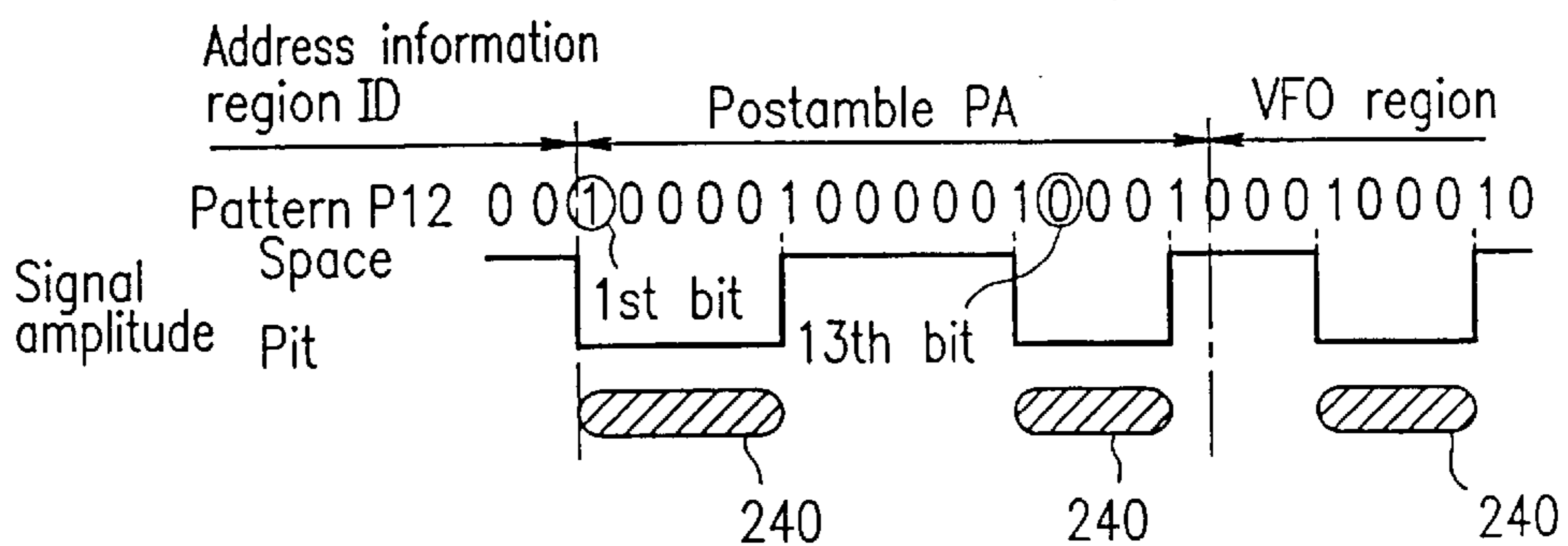
FIG. 24H Next state : 3 or 4, ID end : Space
