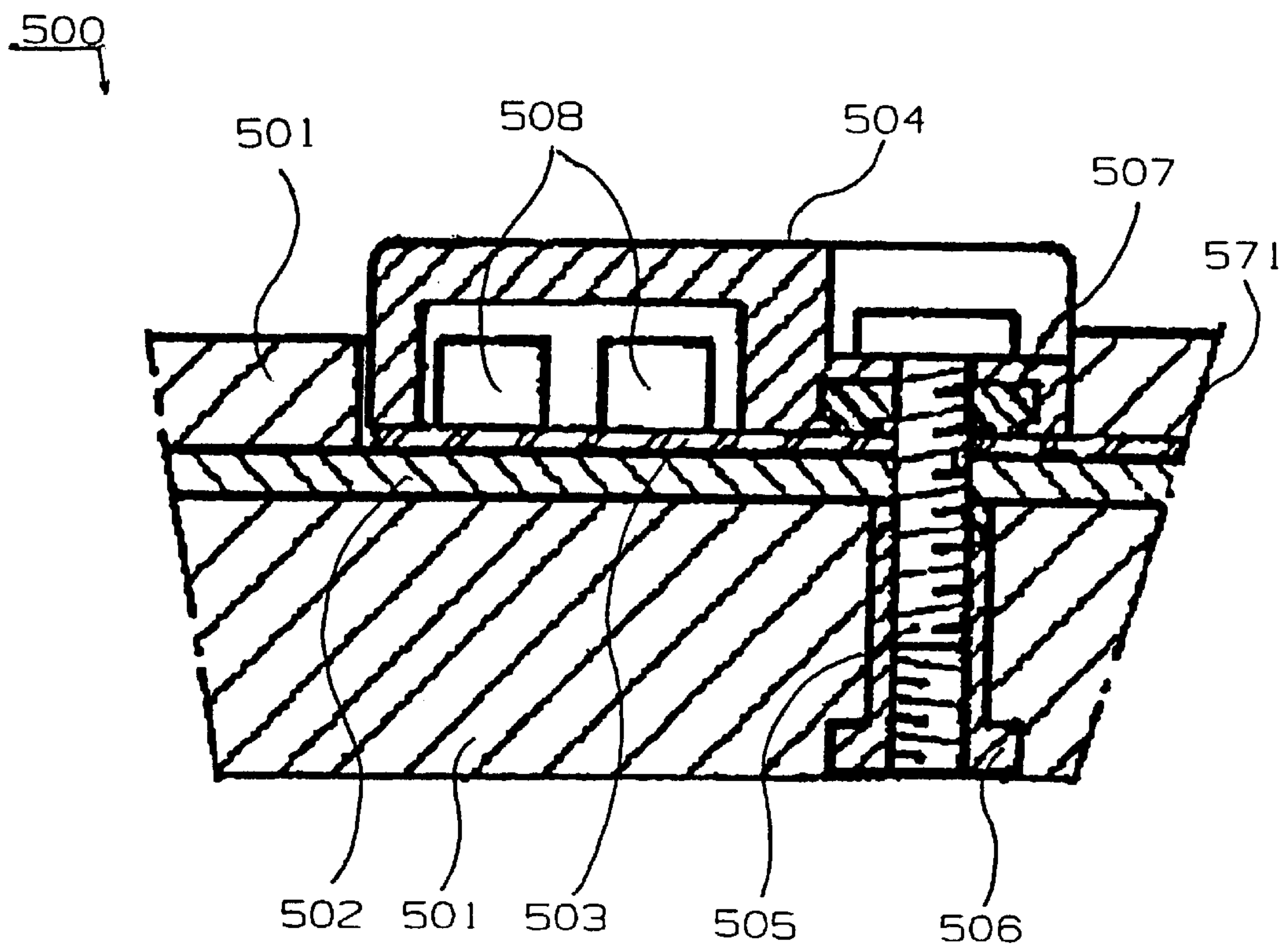
FIG. 6 Prior Art
