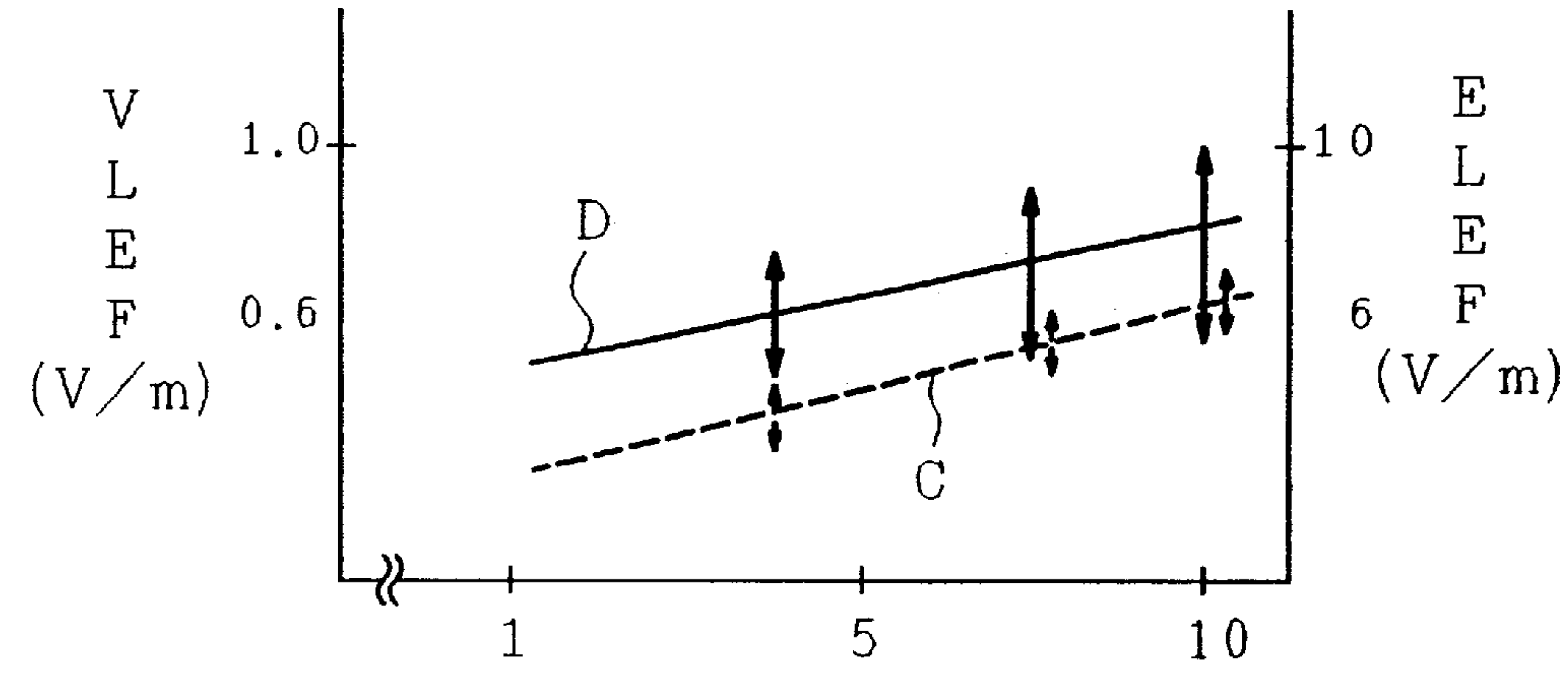
Surface resistance of surface treatment film ( \Omega/\square ) \times 100
