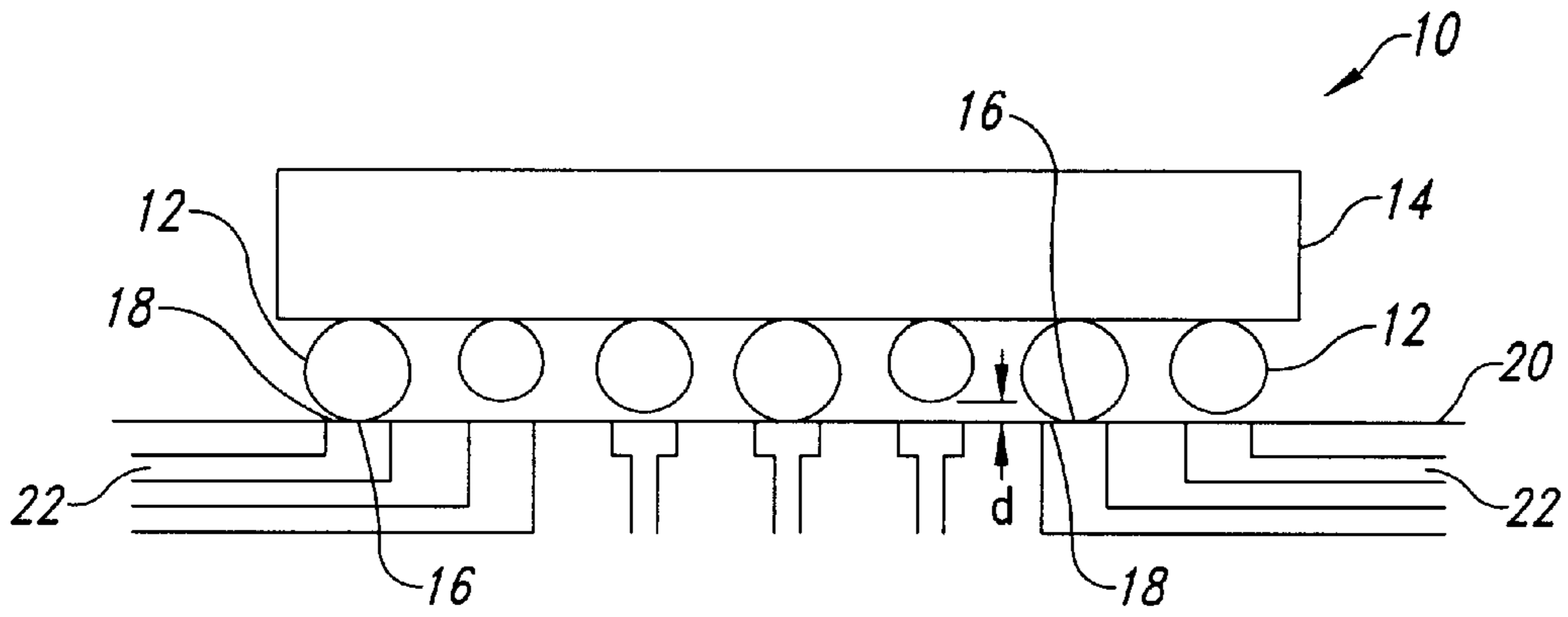
Fig. 1 (Prior Art)
