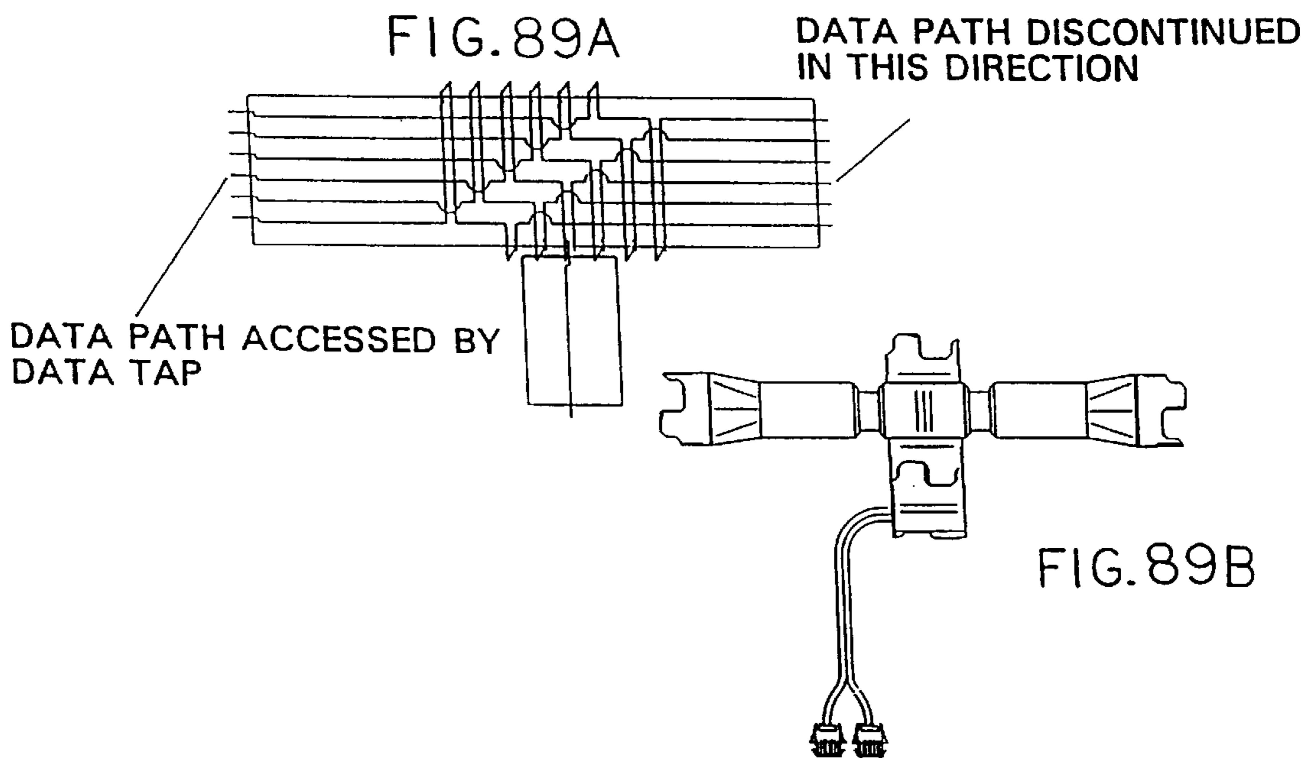
FIG. 89 DATA DISTRIBUTION SEGMENT WITH DATA TAP ATTACHED
