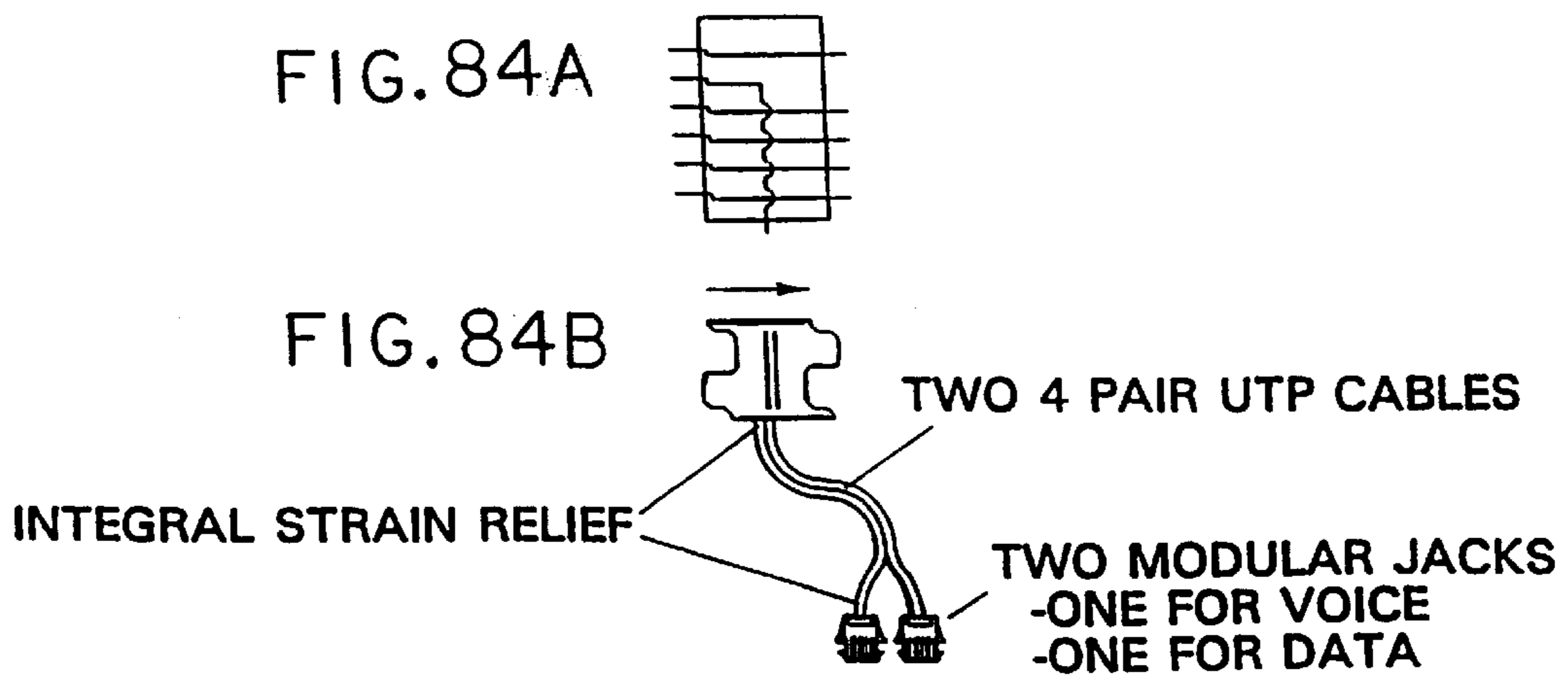
FIG. 84 IN-LINE DATA TAP
